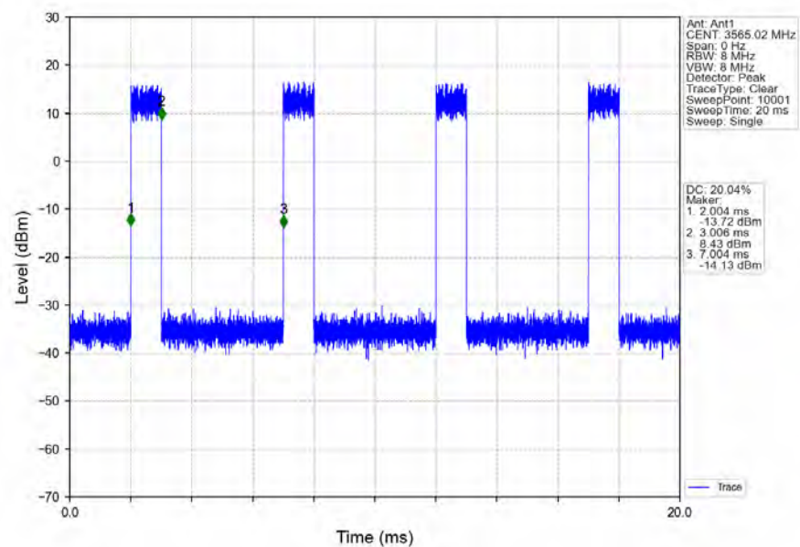
n78d_30kHz_SISO_NTNV_30MHz_CP-OFDM_256_QAM_3565.02MHz_Inner_Full
