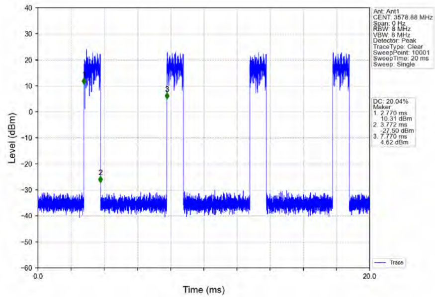
n78d_30kHz_SISO_NTNV_30MHz_DFT-s-OFDM_64_QAM_3565.02MHz_Edge_1RB_Right
