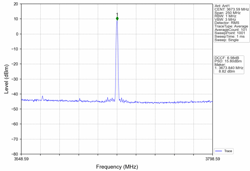
n78d_30kHz_SISO_NTNV_100MHz_DFT-s-OFDM_QPSK_3624.99MHz_Inner_1RB_Right
