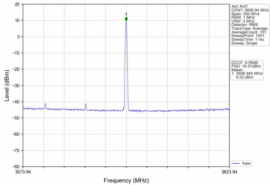
n78d_30kHz_SISO_NTNV_100MHz_CP-OFDM_QPSK_3649.98MHz_Edge_1RB_Right
