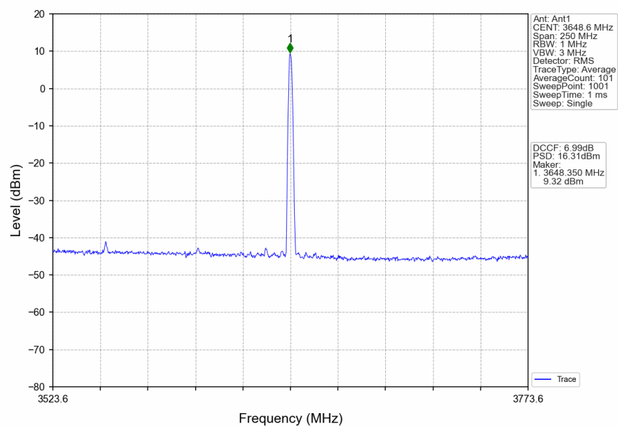
n78d_30kHz_SISO_NTNV_100MHz_DFT-s-OFDM_QPSK_3600MHz_Inner_1RB_Right
