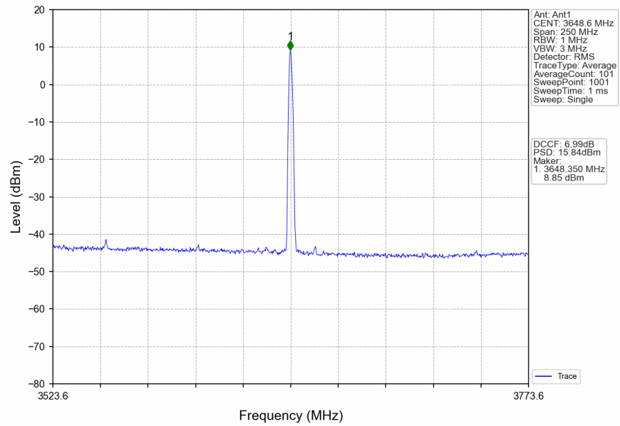
n78d_30kHz_SISO_NTNV_100MHz_CP-OFDM_QPSK_3600MHz_Inner_1RB_Right
