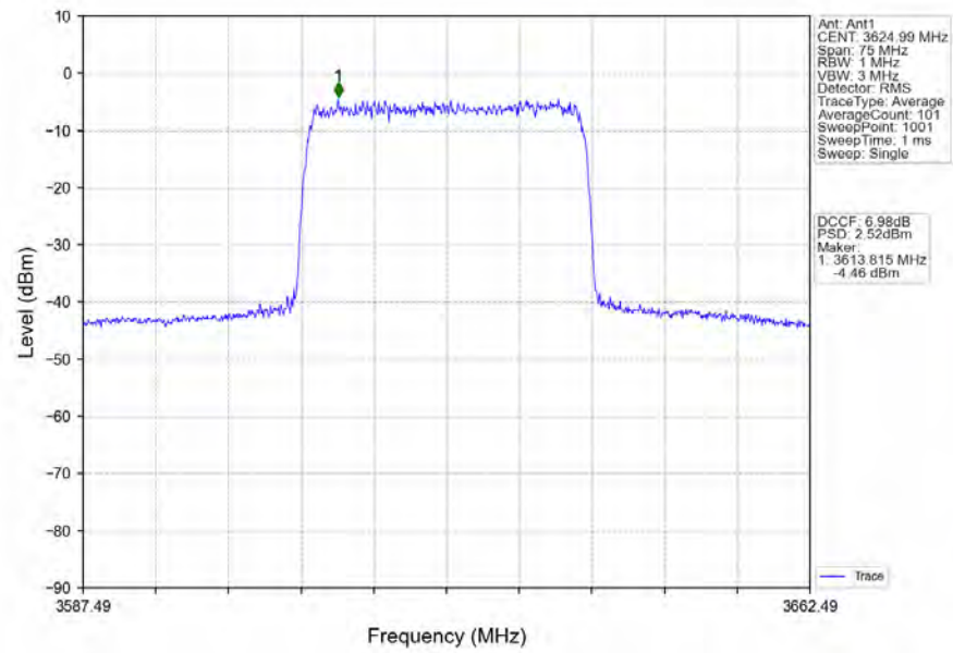
n78d_30kHz_SISO_NTNV_30MHz_CP-OFDM_16_QAM_3624.99MHz_Inner_Full
