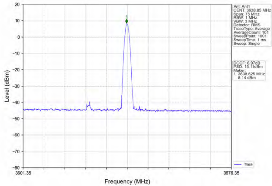
n78d_30kHz_SISO_NTNV_30MHz_DFT-s-OFDM_16_QAM_3624.99MHz_Edge_1RB_Right
