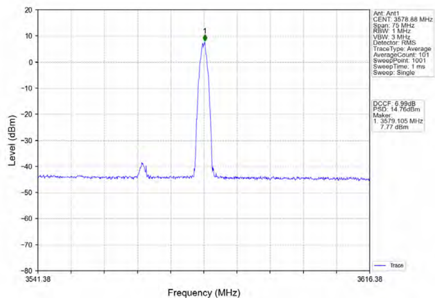
n78d_30kHz_SISO_NTNV_30MHz_CP-OFDM_256_QAM_3565.02MHz_Edge_1RB_Right
