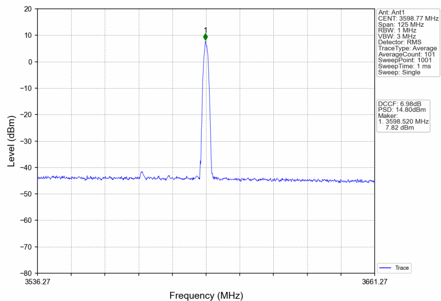
n78d_30kHz_SISO_NTNV_50MHz_CP-OFDM_16_QAM_3575.01MHz_Edge_1RB_Right
