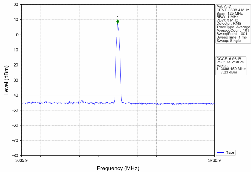
n78d_30kHz_SISO_NTNV_50MHz_CP-OFDM_16_QAM_3675MHz_Inner_1RB_Right
