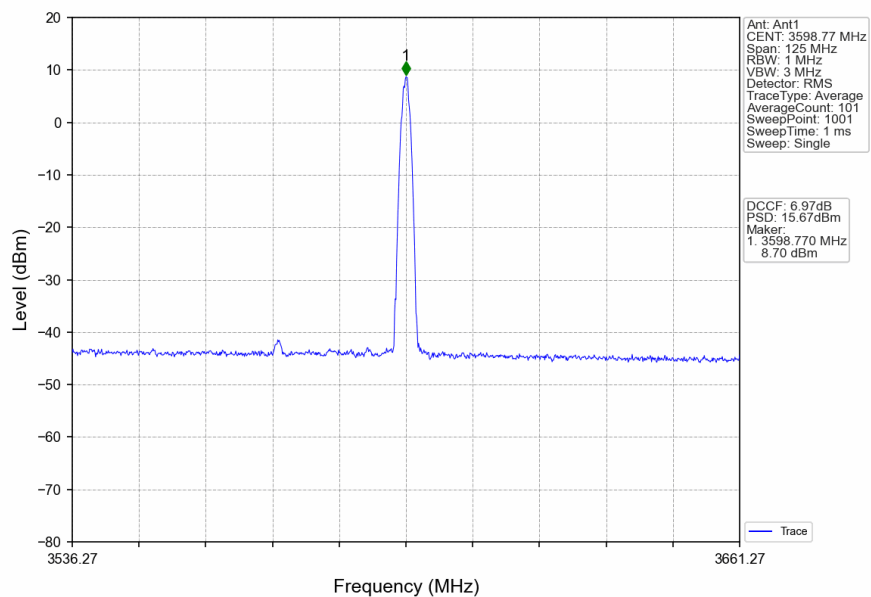
n78d_30kHz_SISO_NTNV_50MHz_DFT-s-OFDM_64_QAM_3575.01MHz_Edge_1RB_Right
