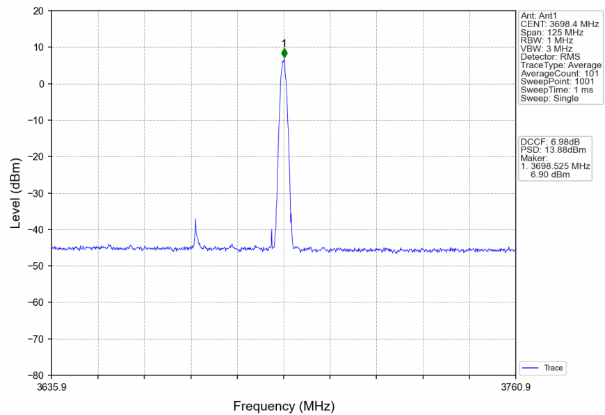
n78d_30kHz_SISO_NTNV_50MHz_CP-OFDM_64_QAM_3675MHz_Inner_1RB_Right
