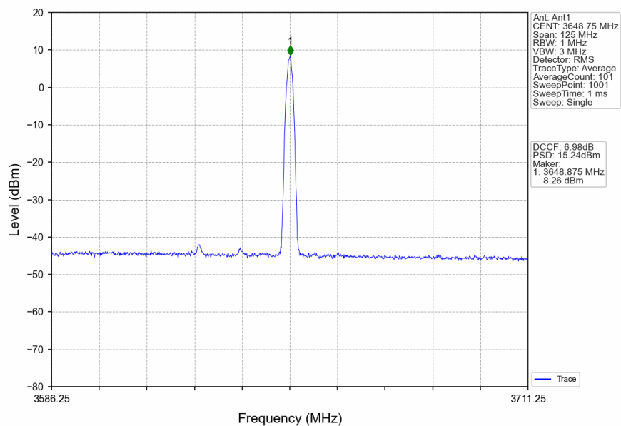
n78d_30kHz_SISO_NTNV_50MHz_DFT-s-OFDM_64_QAM_3624.99MHz_Edge_1RB_Right
