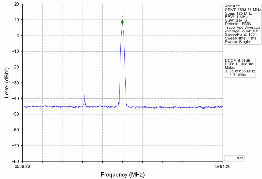
n78d_30kHz_SISO_NTNV_50MHz_CP-OFDM_16_QAM_3675MHz_Edge_1RB_Right
