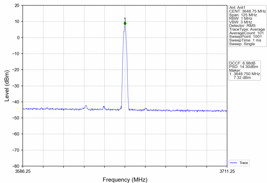
n78d_30kHz_SISO_NTNV_50MHz_CP-OFDM_16_QAM_3624.99MHz_Edge_1RB_Right
