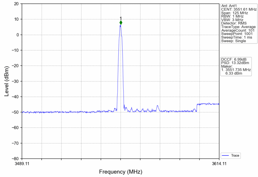
n78d_30kHz_SISO_NTNV_50MHz_CP-OFDM_QPSK_3575.01MHz_Inner_1RB_Right
