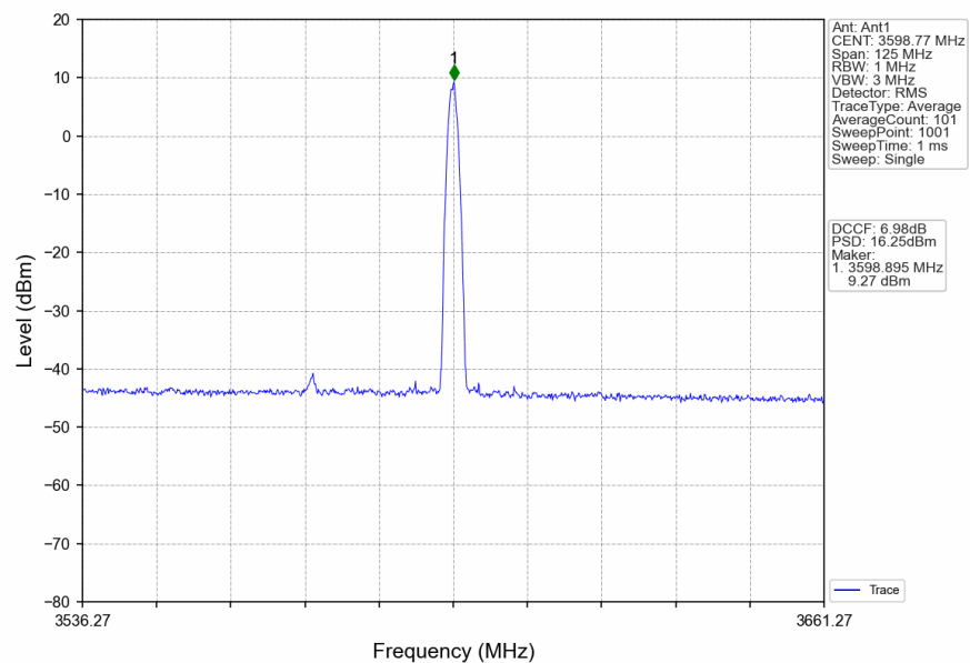
n78d_30kHz_SISO_NTNV_50MHz_CP-OFDM 64 QAM 3575.01MHz_Edge_1RB_Right
