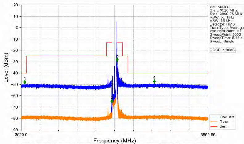
n78d_30kHz_MIMO_NTNV_10MHz_CP-OFDM_QPSK_3694.98MHz_Edge_1RB_Right
