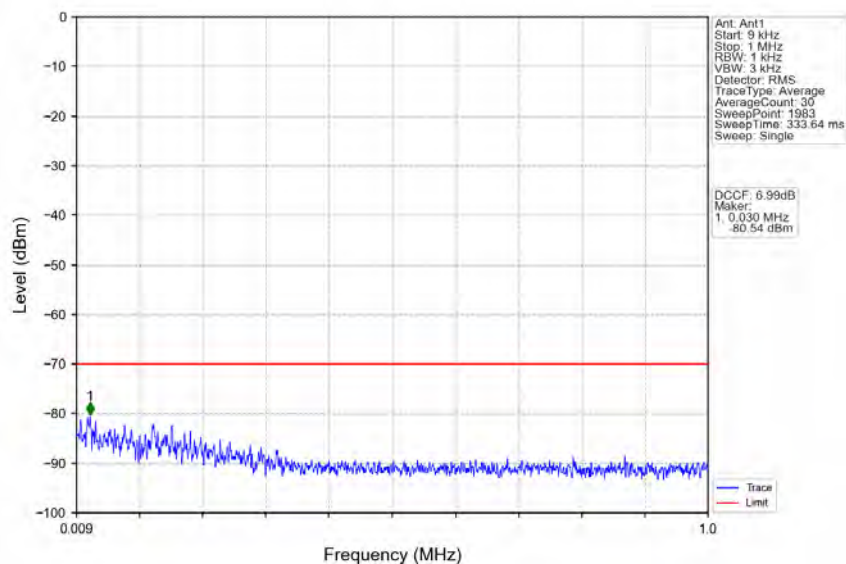
n78d 30kHz MIMO_NTNV_30MHz_CP-OFDM QPSK_3565.02MHz_Edge_1RB_Left
