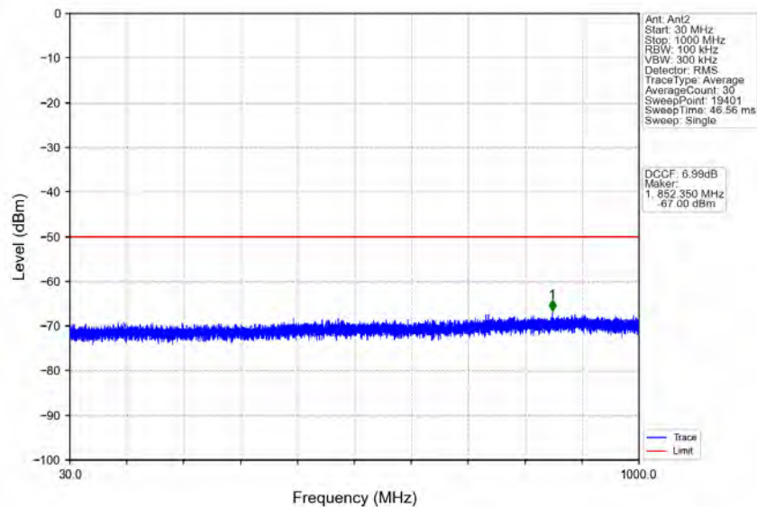
n78d_30kHz_MIMO_NTNV_15MHz_CP-OFDM QPSK_3692.49MHz_Edge_1RB_Right
