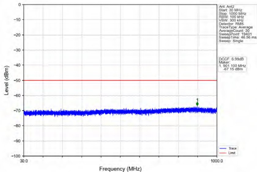
n78d_30kHz_MIMO_NTNV_20MHz_CP-OFDM QPSK_3690MHz_Edge_1RB_Right
