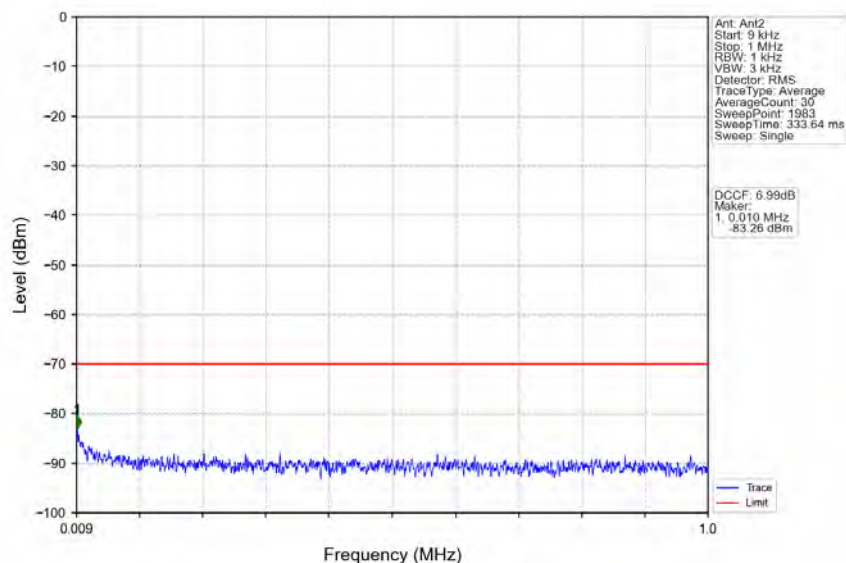
n78d_30kHz_MIMO_NTNV_15MHz_CP-OFDM_QPSK_3692.49MHz_Outer_Full
