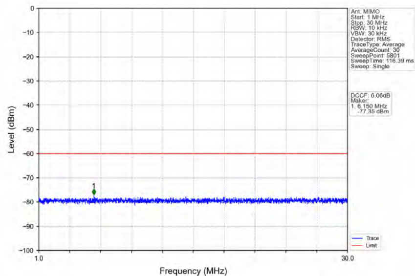
n78d_30kHz_MIMO_NTNV_10MHz_CP-OFDM_QPSK_3694.98MHz_Inner_1RB_Right
