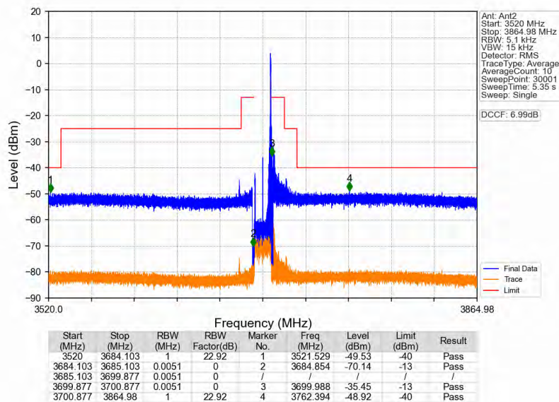
n78d_30kHz_MIMO_NTNV_15MHz_CP-OFDM_QPSK_3692.49MHz_Inner_1RB_Right
