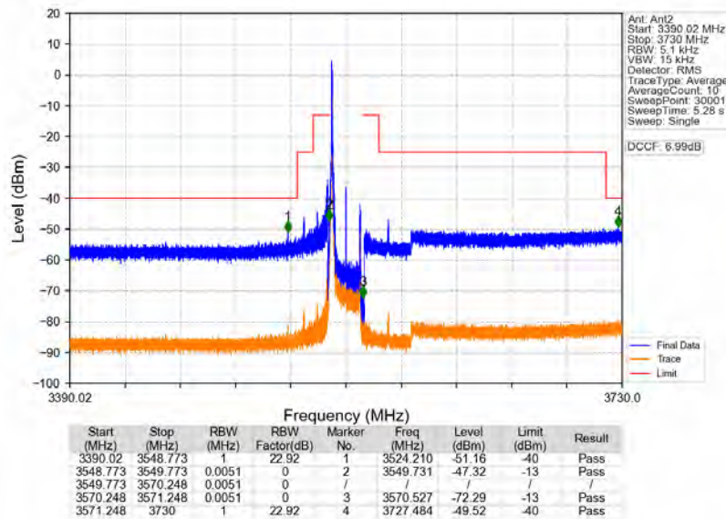
n78d_30kHz_MIMO_NTNV_20MHz_CP-OFDM_QPSK_3560.01MHz_Inner_1RB_Left
