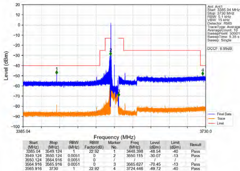
n78d 30kHz MIMO_NTNV_15MHz_CP-OFDM QPSK_3557.52MHz_Edge_1RB_Left
