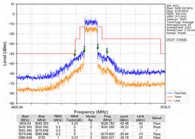
n78d_30kHz_MIMO_NTNV_30MHz_CP-OFDM_QPSK_3565.02MHz_Outer_Full
