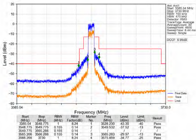
n78d_30kHz_MIMO_NTNV_15MHz_CP-OFDM QPSK_3557.52MHz_Outer_Full
