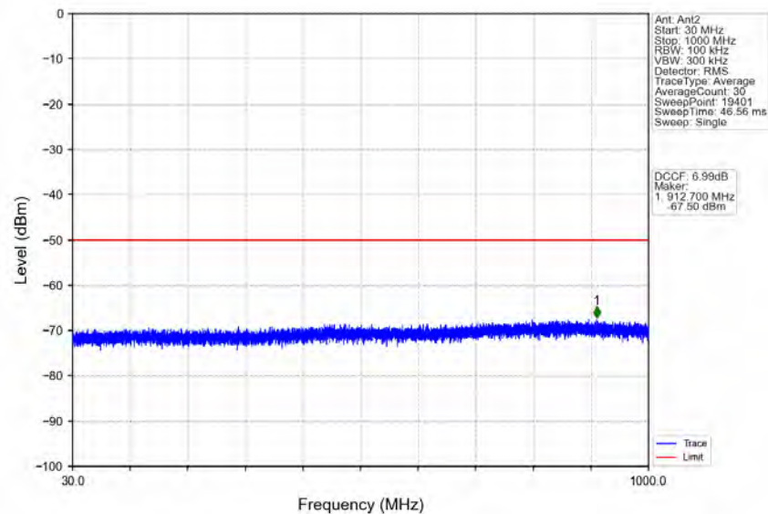
n78d_30kHz_MIMO_NTNV_30MHz_CP-OFDM_QPSK_3565.02MHz_Outer_Full
