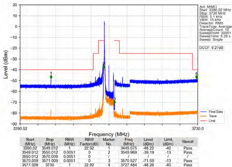
n78d_30kHz_MIMO_NTNV_20MHz_CP-OFDM_QPSK_3560.01MHz_Inner_1RB_Left
