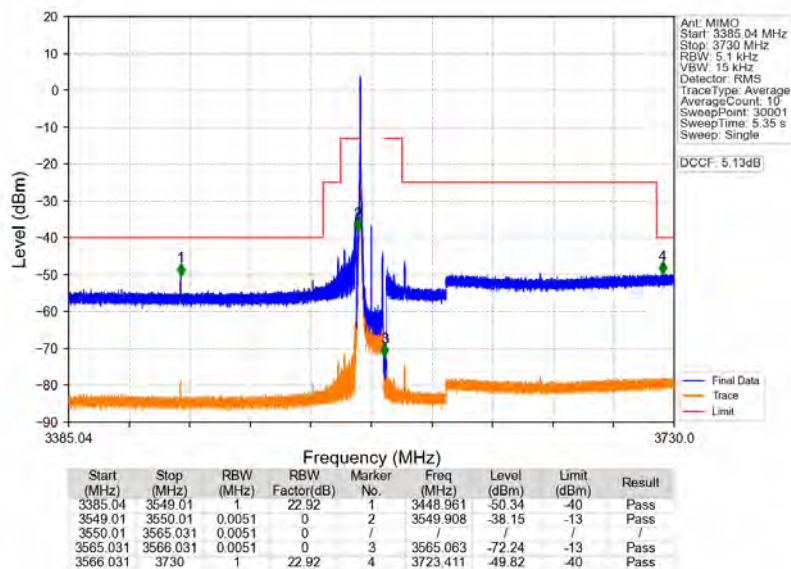
n78d_30kHz_MIMO_NTNV_15MHz_CP-OFDM_QPSK_3557.52MHz_Inner_1RB_Left
