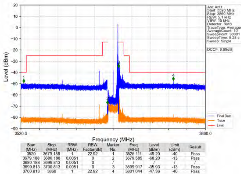
n78d_30kHz_MIMO_NTNV_20MHz_CP-OFDM_QPSK_3690MHz_Inner_1RB_Right
