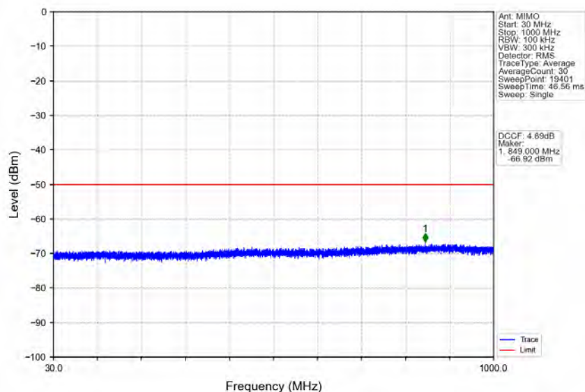
n78d_30kHz_MIMO_NTNV_10MHz_CP-OFDM QPSK_3694.98MHz_Edge_1RB_Right
