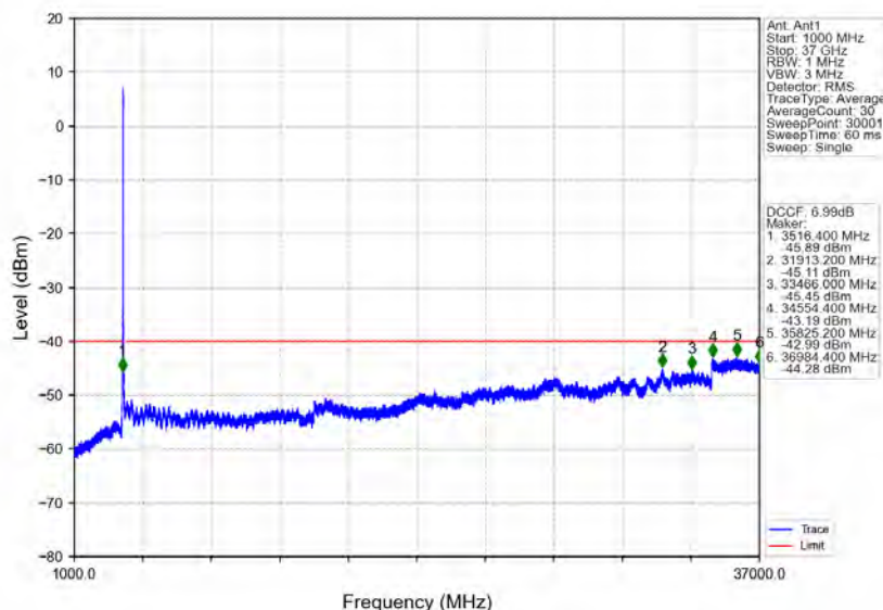
n78d_30kHz_MIMO_NTNV_20MHz_CP-OFDM_QPSK_3560.01MHz_Outer_Full
