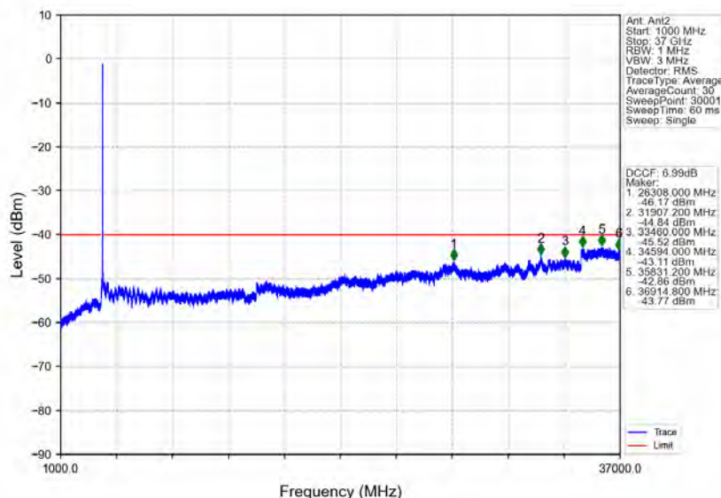
n78d_30kHz_MIMO_NTNV_20MHz_CP-OFDM_QPSK_3690MHz_Outer_Full
