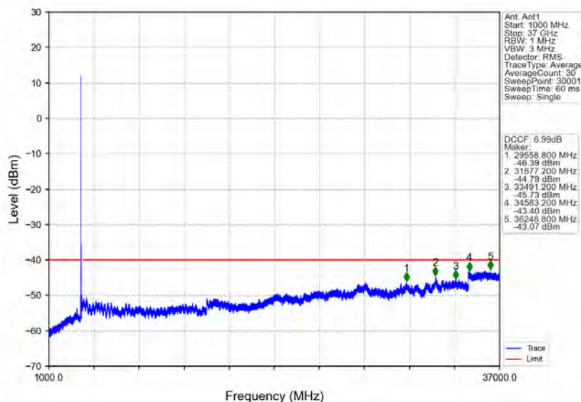
n78d_30kHz_MIMO_NTNV_30MHz_CP-OFDM_QPSK_3565.02MHz_Edge_1RB_Left
