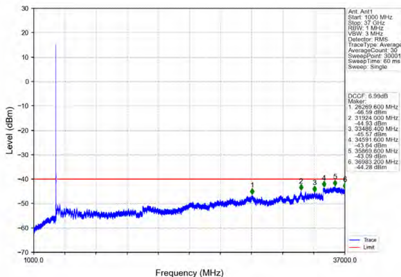
n78d_30kHz_MIMO_NTNV_15MHz_CP-OFDM_QPSK_3557.52MHz_Inner_1RB_Left
