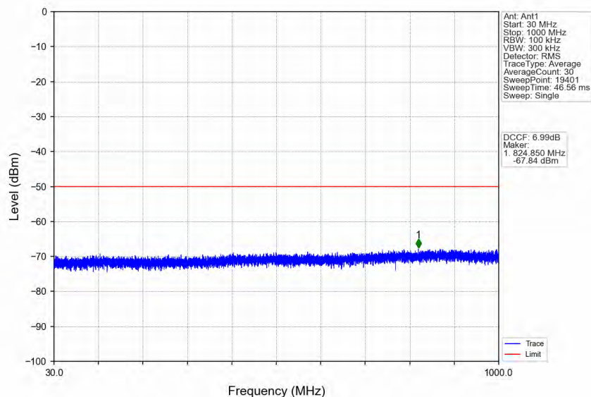
n78d_30kHz_MIMO_NTNV_20MHz_CP-OFDM_QPSK_3560.01MHz_Outer_Full
