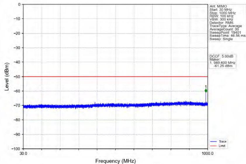
n78d_30kHz_MIMO_NTNV_15MHz_CP-OFDM_QPSK_3557.52MHz_Edge_1RB_Left
