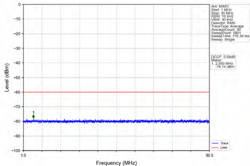
n78d_30kHz_MIMO_NTNV_30MHz_CP-OFDM_QPSK_3565.02MHz_Outer_Full
