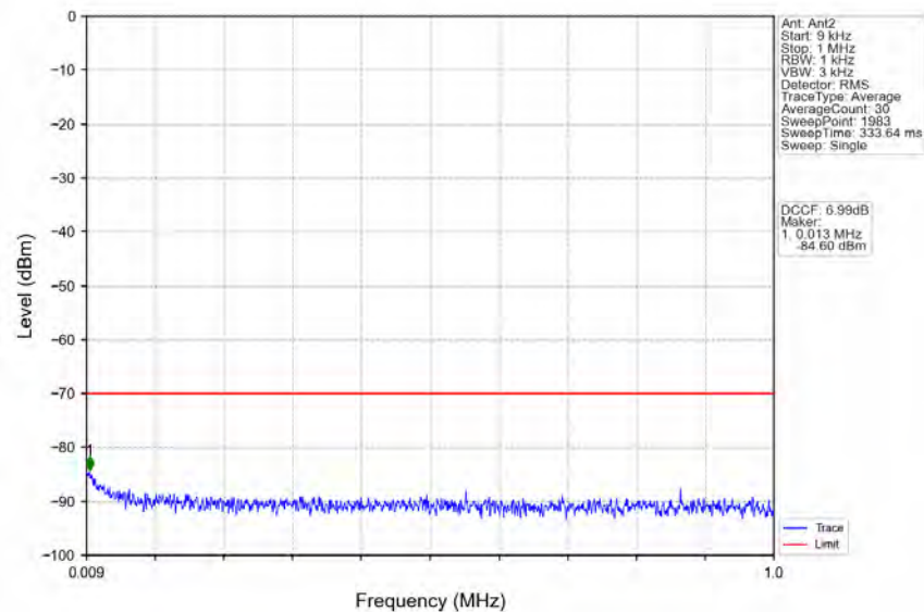
n78d_30kHz_MIMO_NTNV_20MHz_CP-OFDM_QPSK_3690MHz_Outer_Full
