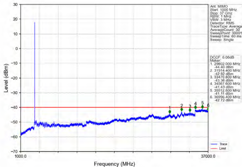
n78d_30kHz_MIMO_NTNV_10MHz_CP-OFDM QPSK_3694.98MHz_Inner_1RB_Right
