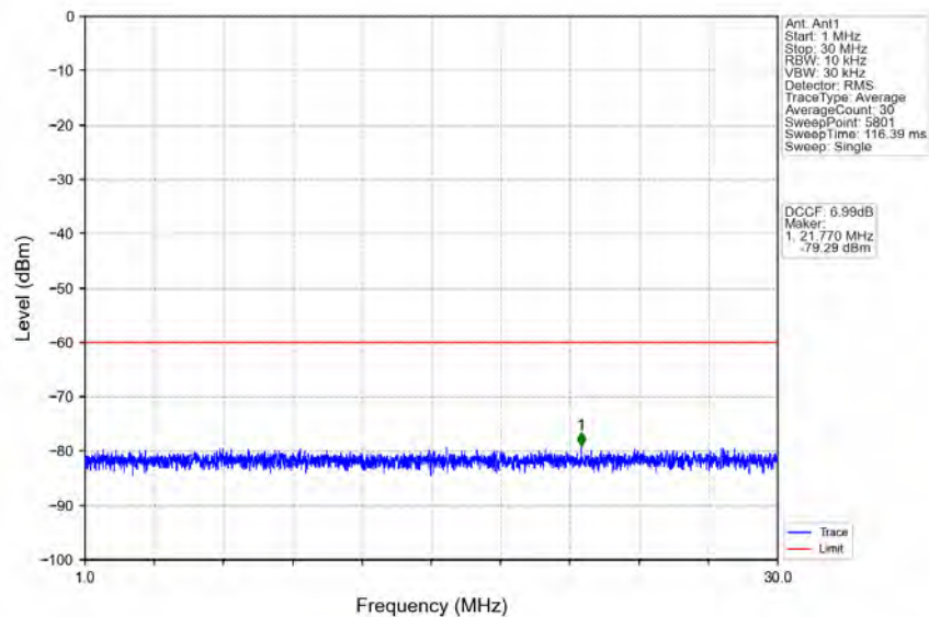
n78d_30kHz_MIMO_NTNV_20MHz_CP-OFDM_QPSK_3560.01MHz_Edge_1RB_Left
