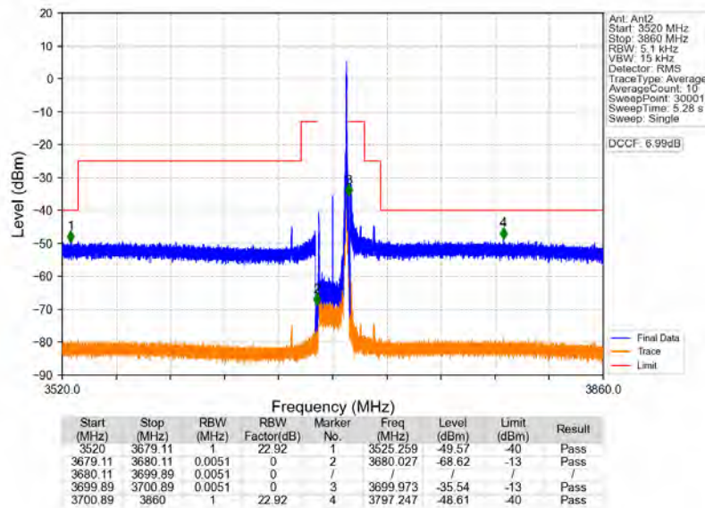
n78d_30kHz_MIMO_NTNV_20MHz_CP-OFDM_QPSK_3690MHz_Inner_1RB_Right
