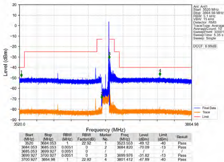
n78d_30kHz_MIMO_NTNV_15MHz_CP-OFDM_QPSK_3692.49MHz_Edge_1RB_Right
