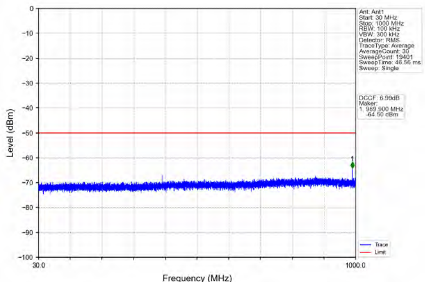
n78d_30kHz_MIMO_NTNV_30MHz_CP-OFDM_QPSK_3565.02MHz_Edge_1RB_Left
