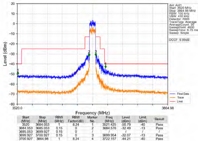
n78d_30kHz_MIMO_NTNV_15MHz_CP-OFDM_QPSK_3692.49MHz_Outer_Full
