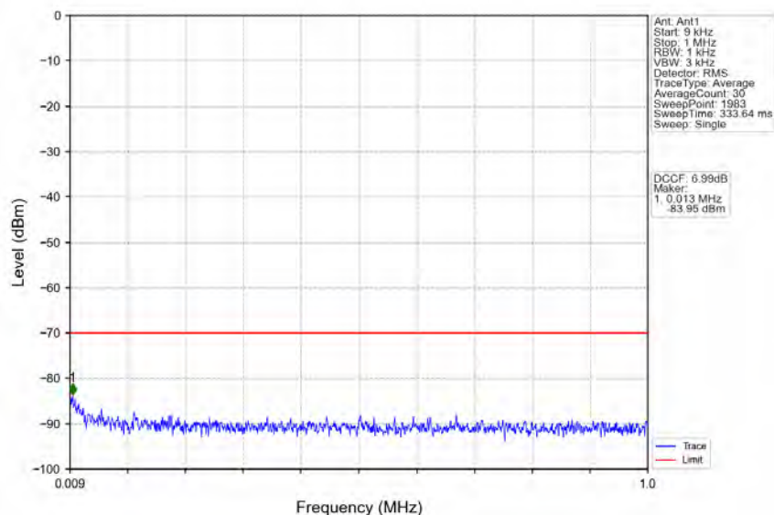
n78d_30kHz_MIMO_NTNV_15MHz_CP-OFDM_QPSK_3557.52MHz_Outer_Full
