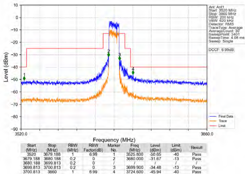
n78d_30kHz_MIMO_NTNV_20MHz_CP-OFDM_QPSK_3690MHz_Outer_Full
