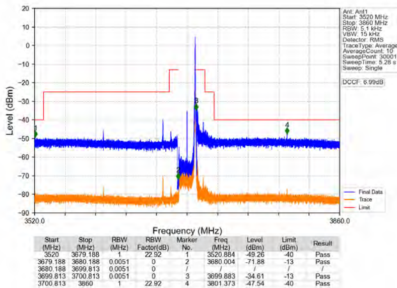
n78d_30kHz_MIMO_NTNV_20MHz_CP-OFDM_QPSK_3690MHz_Edge_1RB_Right
