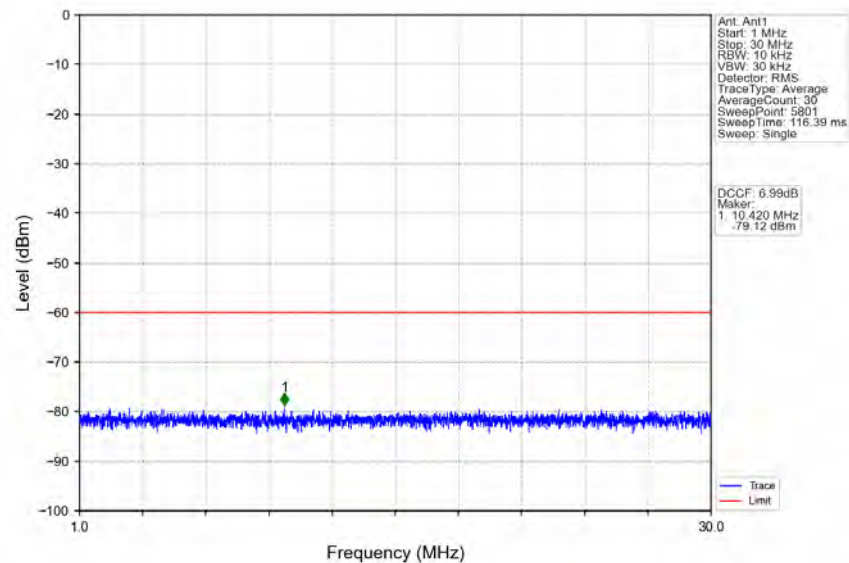
n78d_30kHz_MIMO_NTNV_15MHz_CP-OFDM_QPSK_3557.52MHz_Inner_1RB_Left
