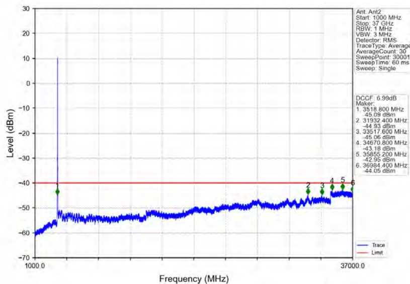
n78d 30kHz MIMO NTV 15MHz CP-OFDM QPSK 3557.52MHz Outer Full
