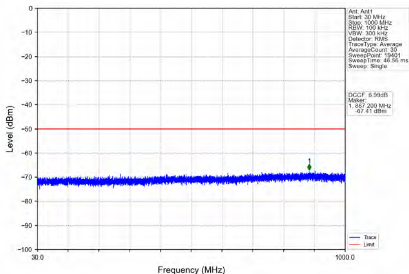
n78d_30kHz_MIMO_NTNV_30MHz_CP-OFDM QPSK_3565.02MHz_Outer_Full
