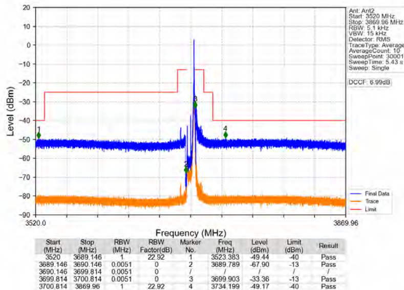
n78d_30kHz_MIMO_NTNV_10MHz_CP-OFDM_QPSK_3694.98MHz_Inner_1RB_Right
