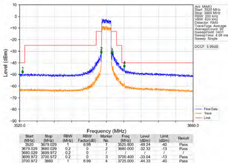
n78d_30kHz_MIMO_NTNV_20MHz_CP-OFDM_QPSK_3690MHz_Outer_Full
