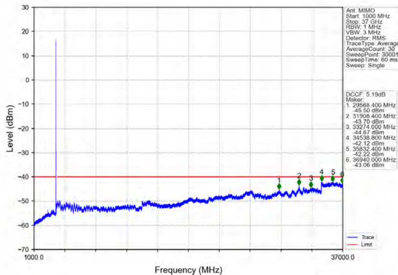
n78d_30kHz_MIMO_NTNV_10MHz_CP-OFDM QPSK_3694.98MHz_Edge_1RB_Right
