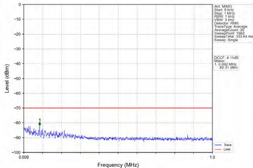
n78d_30kHz_MIMO_NTNV_15MHz_CP-OFDM QPSK_3692.49MHz_Inner_1RB_Right
