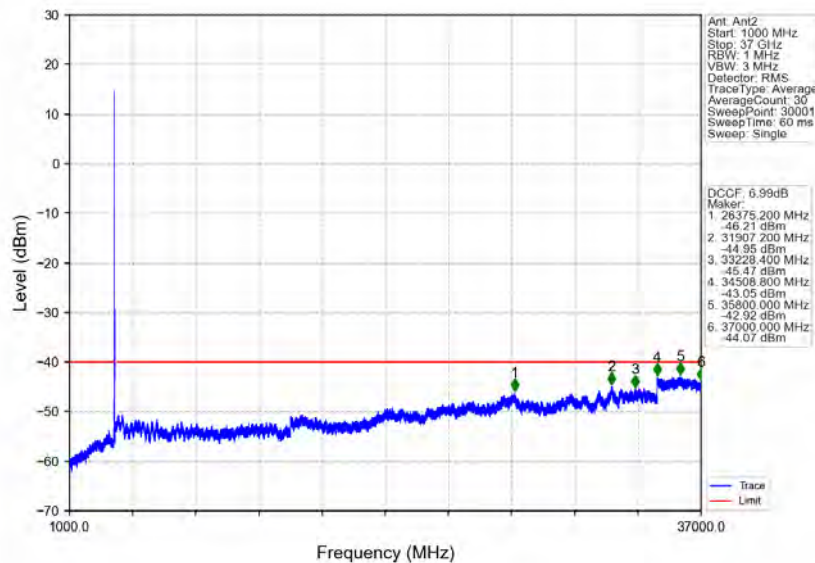
n78d_30kHz_MIMO_NTNV_20MHz_CP-OFDM_QPSK_3560.01MHz_Edge_1RB_Left
