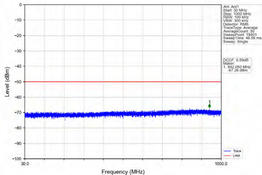
n78d_30kHz_MIMO_NTNV_15MHz_CP-OFDM_QPSK_3692.49MHz_Inner_1RB_Right
