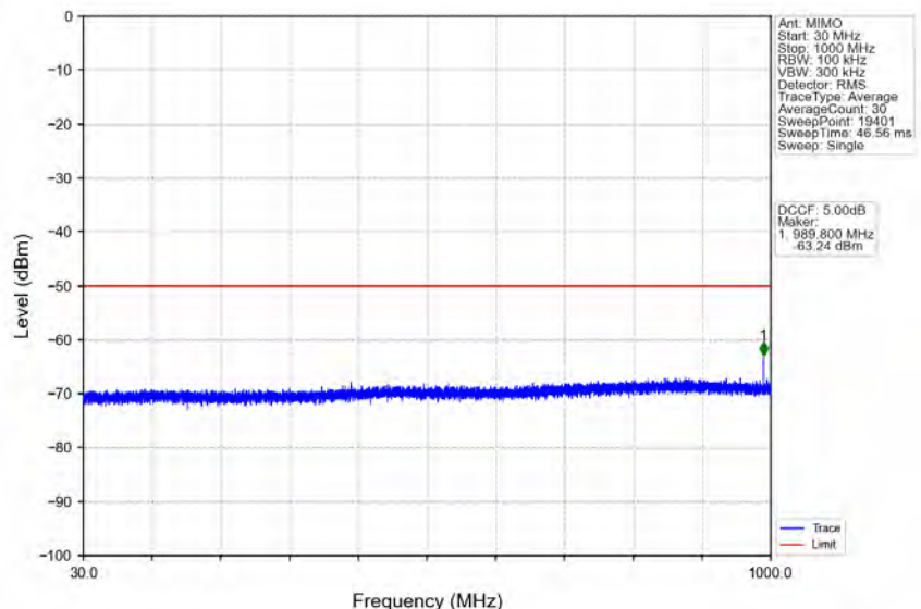
n78d_30kHz_MIMO_NTNV_20MHz_CP-OFDM_QPSK_3560.01MHz_Edge_1RB_Left
