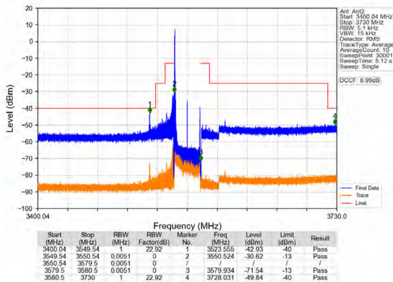
n78d_30kHz_MIMO_NTNV_30MHz_CP-OFDM_QPSK_3565.02MHz_Edge_1RB_Left
