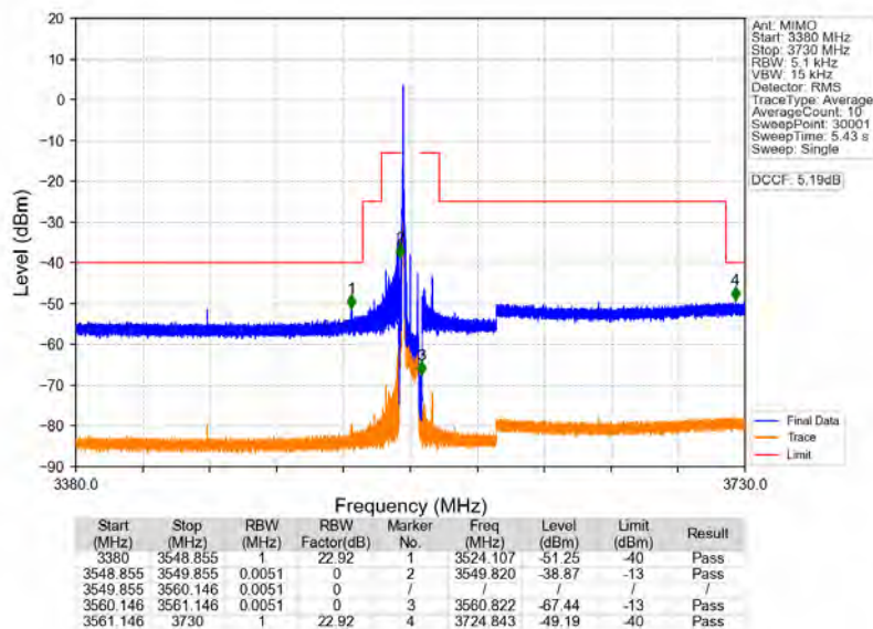
n78d_30kHz_MIMO_NTNV_10MHz_CP-OFDM_QPSK_3555MHz_Inner_1RB_Left
