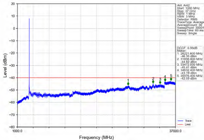
n78d_30kHz_MIMO_NTNV_15MHz_CP-OFDM_QPSK_3692.49MHz_Outer_Full
