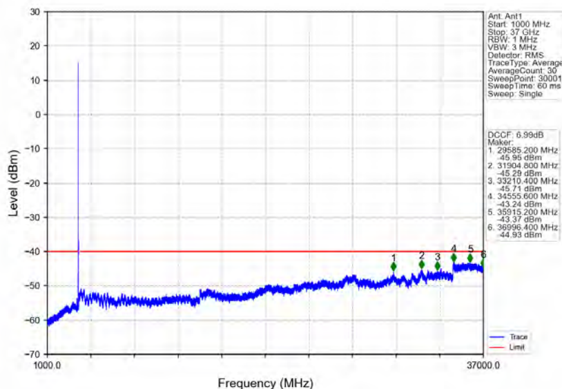
n78d_30kHz_MIMO_NTNV_15MHz_CP-OFDM_QPSK_3557.52MHz_Edge_1RB_Left
