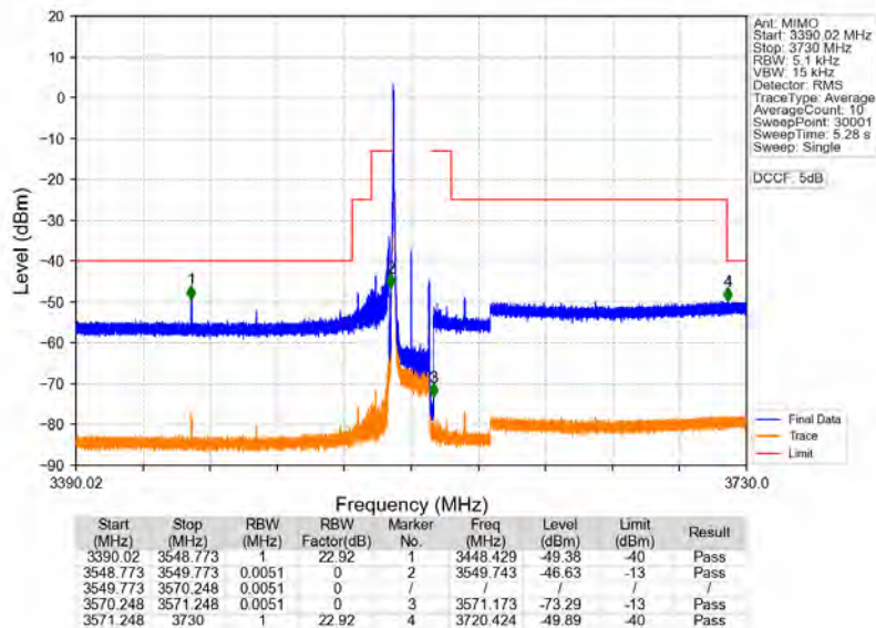
n78d_30kHz_MIMO_NTNV_20MHz_CP-OFDM_QPSK_3560.01MHz_Edge_1RB_Left
