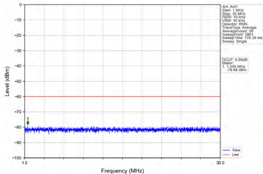
n78d_30kHz_MIMO_NTNV_20MHz_CP-OFDM_QPSK_3690MHz_Inner_1RB_Right
