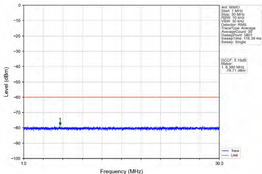
n78d_30kHz_MIMO_NTNV_10MHz_CP-OFDM QPSK_3555MHz_Inner_1RB_Left
