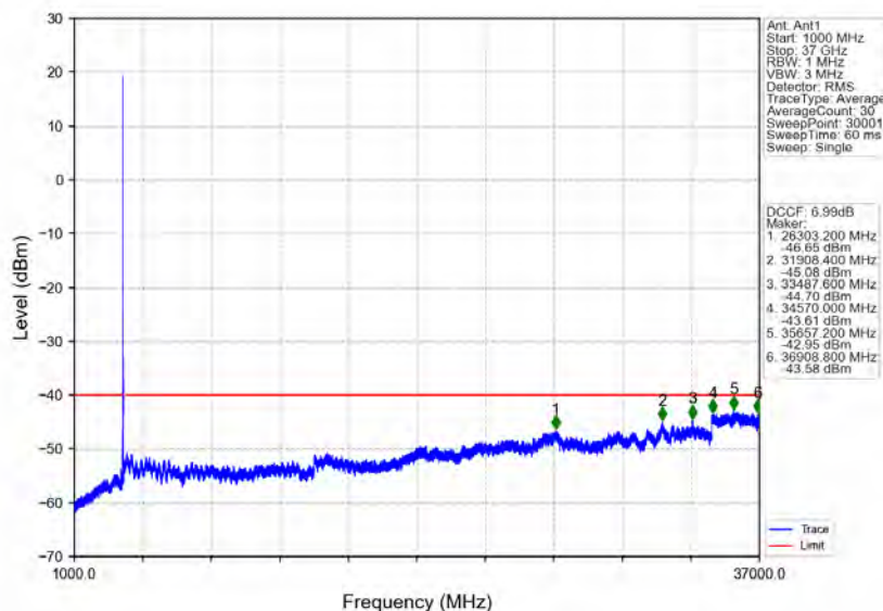
n78d_30kHz_MIMO_NTNV_20MHz_CP-OFDM_QPSK_3560.01MHz_Inner_1RB_Left
