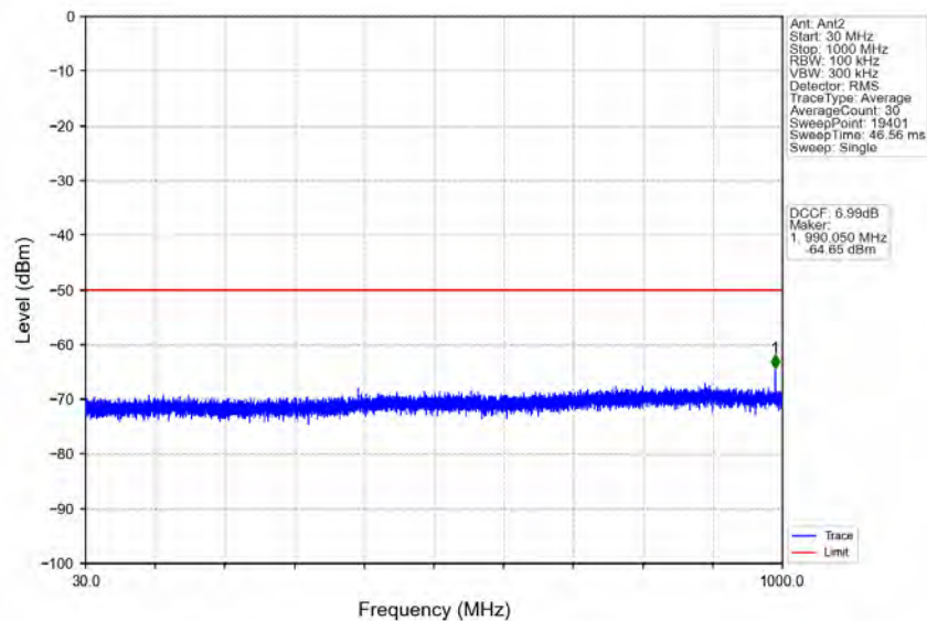
n78d_30kHz_MIMO_NTNV_20MHz_CP-OFDM_QPSK_3560.01MHz_Inner_1RB_Left
