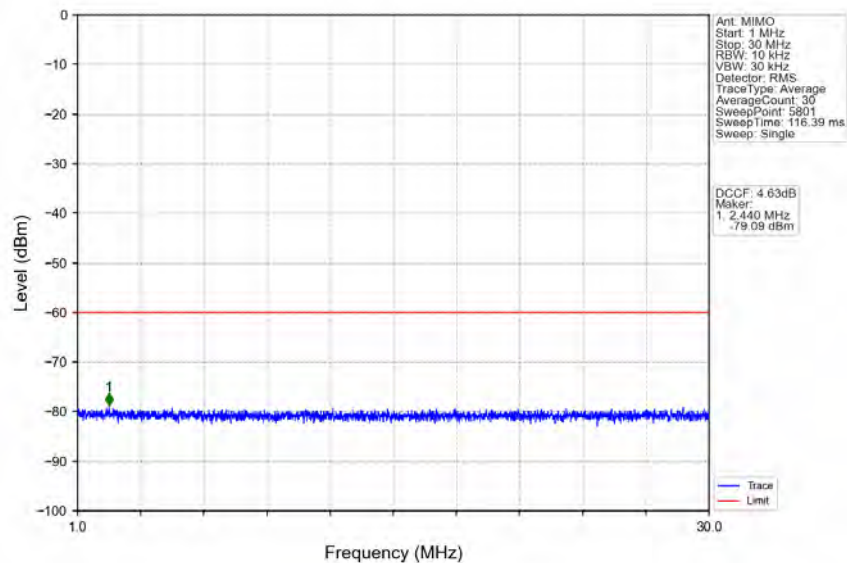
n78d_30kHz_MIMO_NTNV_10MHz_CP-OFDM QPSK_3694.98MHz_Outer_Full
