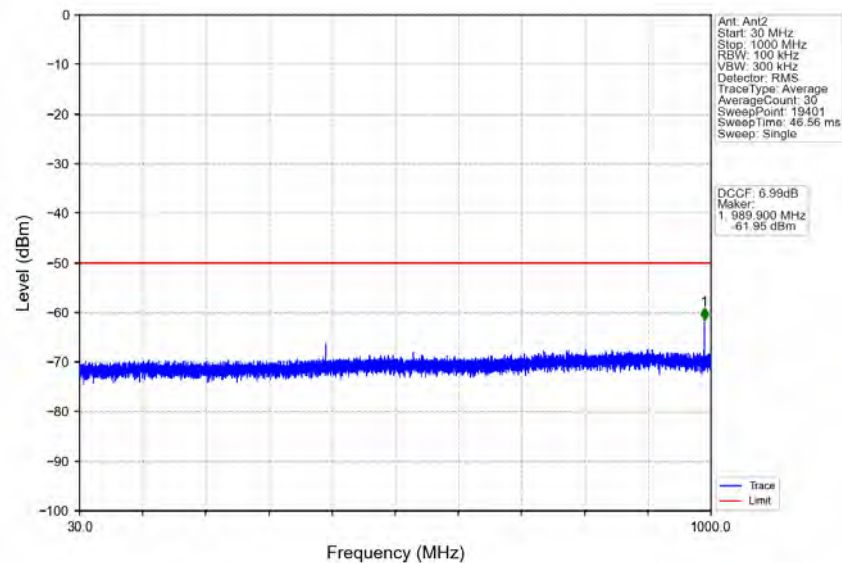
n78d_30kHz_MIMO_NTNV_30MHz_CP-OFDM_QPSK_3565.02MHz_Edge_1RB_Left
