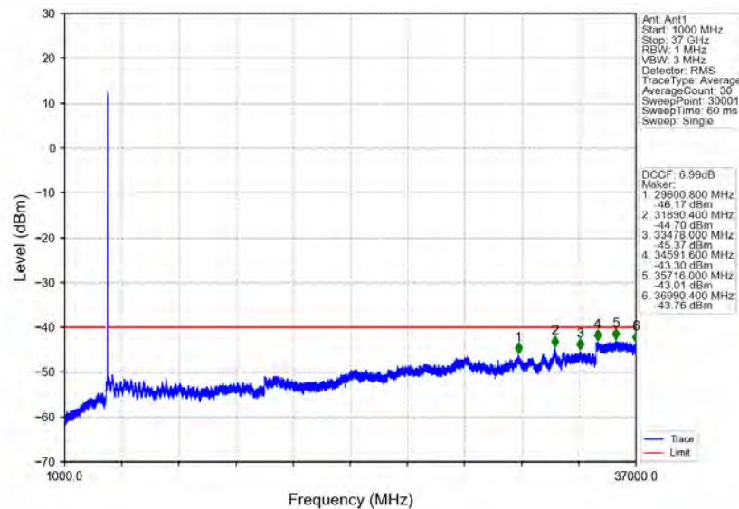
n78d_30kHz_MIMO_NTNV_15MHz_CP-OFDM_QPSK_3692.49MHz_Inner_1RB_Right
