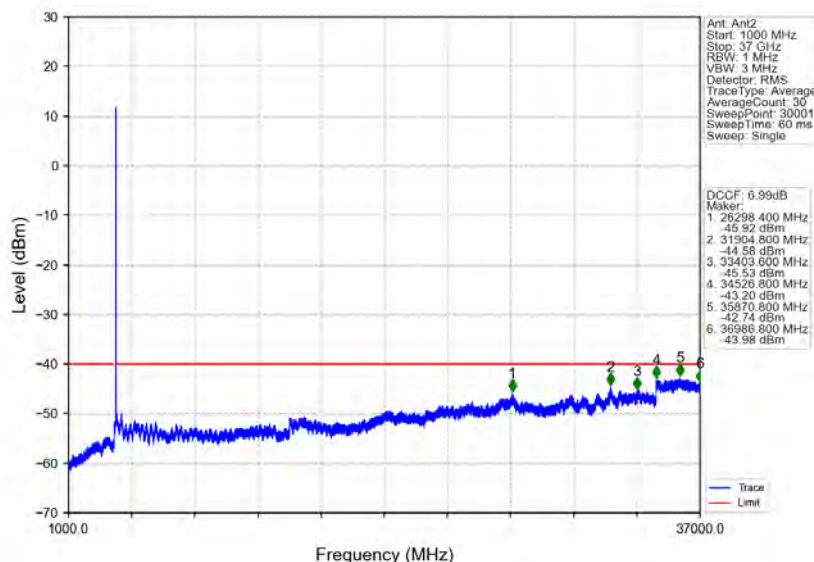
n78d_30kHz_MIMO_NTNV_10MHz_CP-OFDM_QPSK_3694.98MHz_Outer_Full
