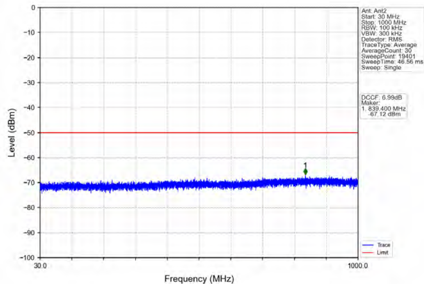
n78d_30kHz_MIMO_NTNV_15MHz_CP-OFDM_QPSK_3692.49MHz_Outer_Full
