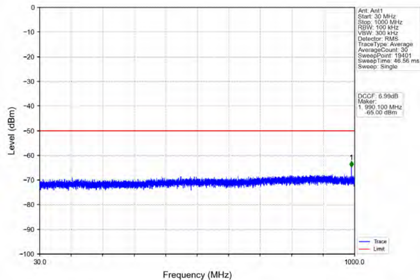
n78d_30kHz_MIMO_NTNV_20MHz_CP-OFDM_QPSK_3560.01MHz_Inner_1RB_Left
