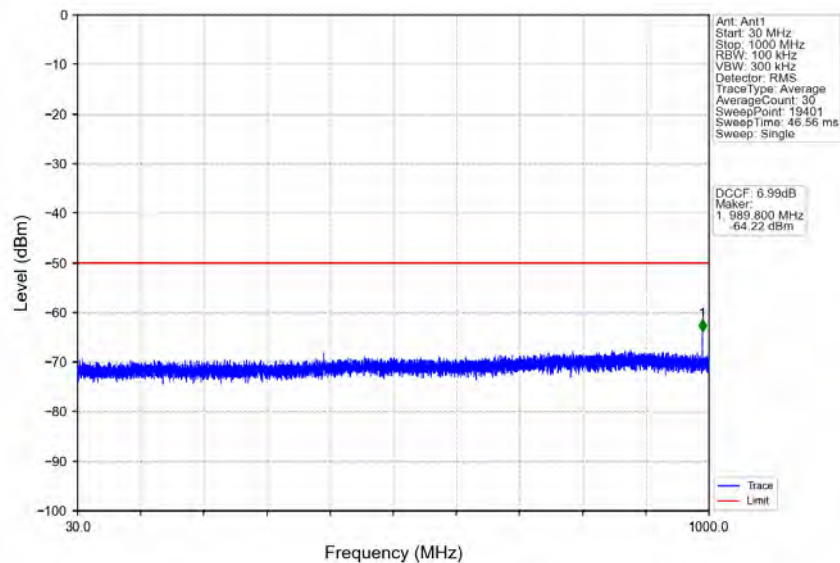
n78d_30kHz_MIMO_NTNV_20MHz_CP-OFDM_QPSK_3560.01MHz_Edge_1RB_Left
