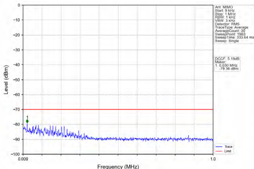
n78d_30kHz_MIMO_NTNV_10MHz_CP-OFDM_QPSK_3555MHz_Inner_1RB_Left
