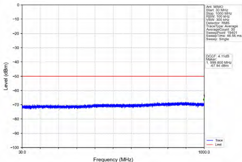
n78d_30kHz_MIMO_NTNV_15MHz_CP-OFDM QPSK_3692.49MHz_Inner_1RB_Right
