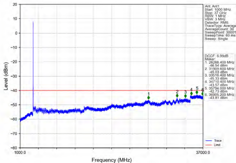
n78d_30kHz_MIMO_NTNV_15MHz_CP-OFDM QPSK_3557.52MHz_Outer_Full
