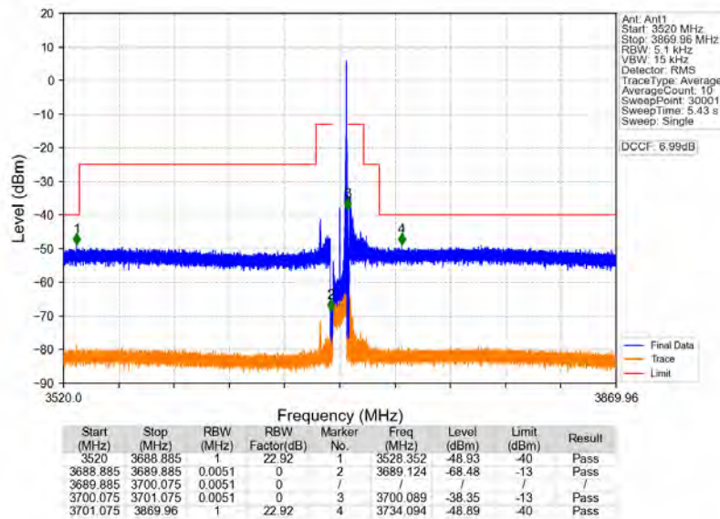
n78d_30kHz_MIMO_NTNV_10MHz_CP-OFDM QPSK_3694.98MHz_Edge_1RB_Right
