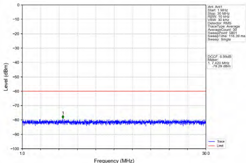
n78d_30kHz_MIMO_NTNV_10MHz_CP-OFDM QPSK_3694.98MHz_Edge_1RB_Right
