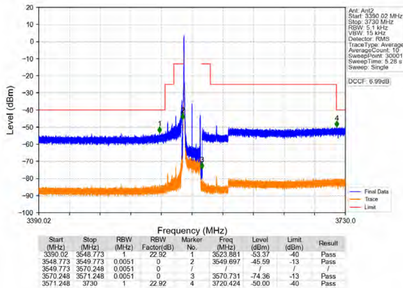
n78d_30kHz_MIMO_NTNV_20MHz_CP-OFDM_QPSK_3560.01MHz_Edge_1RB_Left
