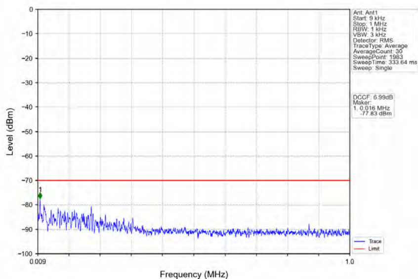
n78d 30kHz MIMO_NTNV_15MHz_CP-OFDM QPSK_3557.52MHz_Edge_1RB_Left
