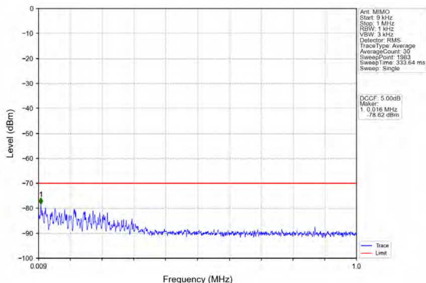
n78d_30kHz_MIMO_NTNV_15MHz_CP-OFDM_QPSK_3557.52MHz_Edge_1RB_Left
