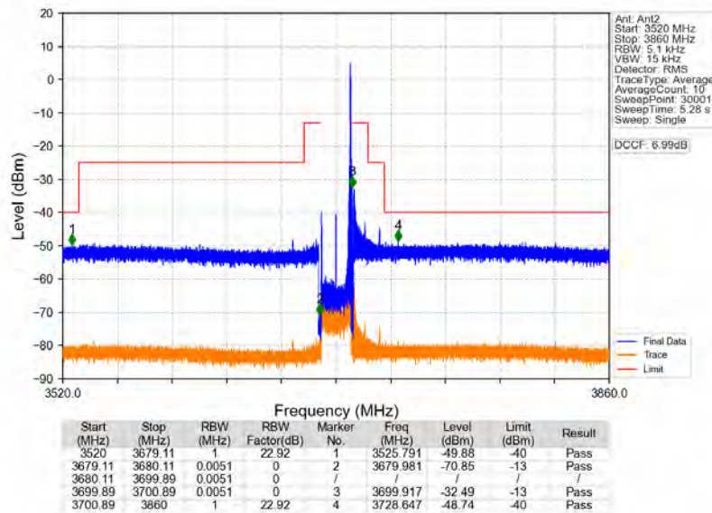
n78d_30kHz_MIMO_NTNV_20MHz_CP-OFDM_QPSK_3690MHz_Edge_1RB_Right
