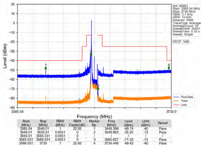
n78d_30kHz_MIMO_NTNV_15MHz_CP-OFDM_QPSK_3557.52MHz_Edge_1RB_Left
