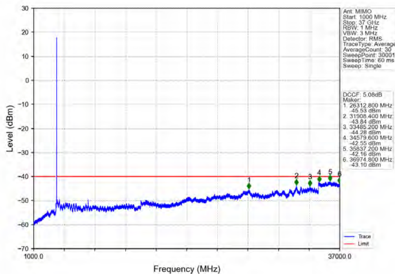
n78d_30kHz_MIMO_NTNV_15MHz_CP-OFDM QPSK_3692.49MHz_Edge_1RB_Right
