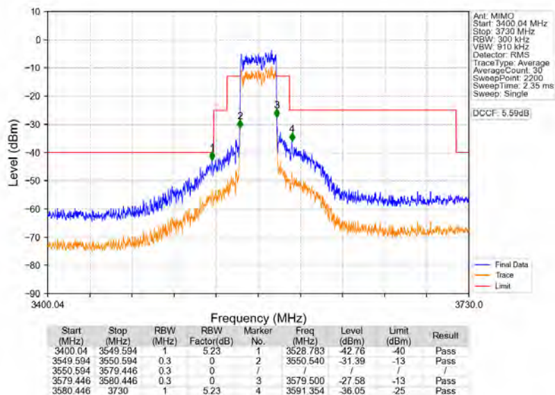
n78d_30kHz_MIMO_NTNV_30MHz_CP-OFDM_QPSK_3565.02MHz_Outer_Full
