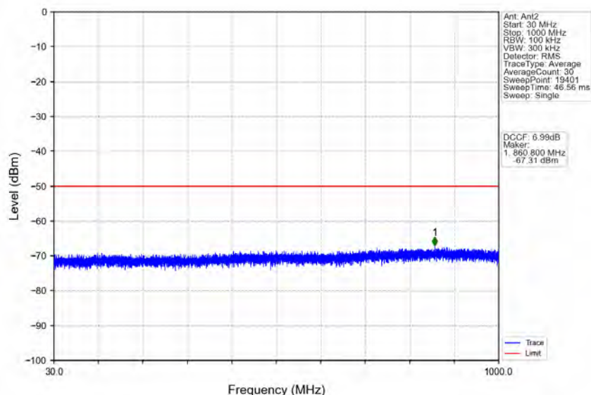
n78d_30kHz_MIMO_NTNV_10MHz_CP-OFDM_QPSK_3694.98MHz_Inner_1RB_Right
