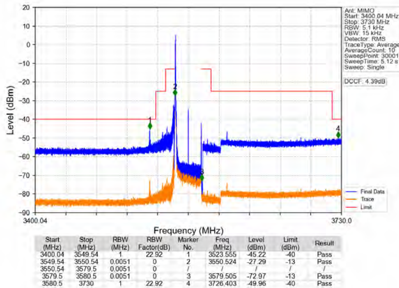
n78d_30kHz_MIMO_NTNV_30MHz_CP-OFDM_QPSK_3565.02MHz_Edge_1RB_Left
