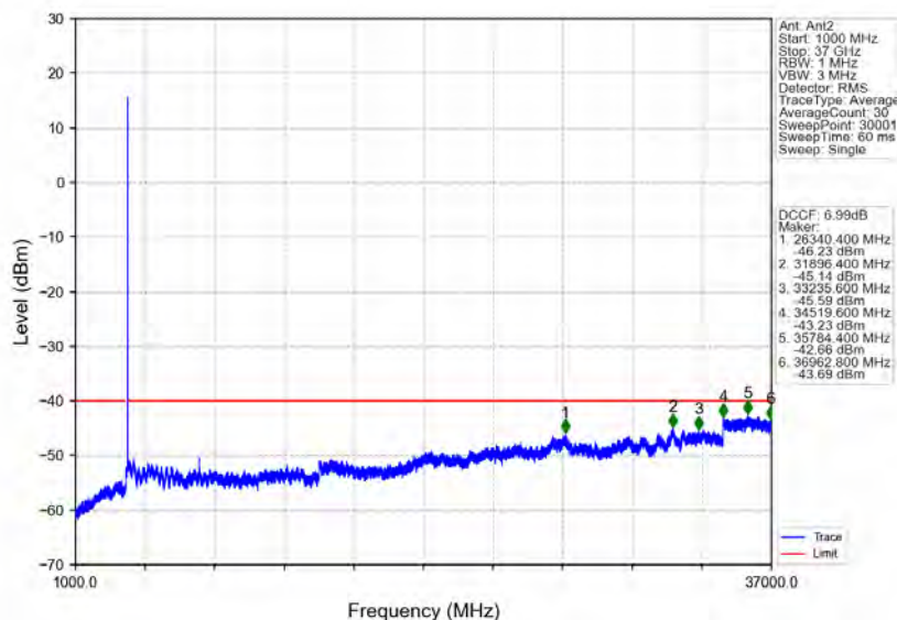
n78d_30kHz_MIMO_NTNV_20MHz_CP-OFDM_QPSK_3690MHz_Edge_1RB_Right
