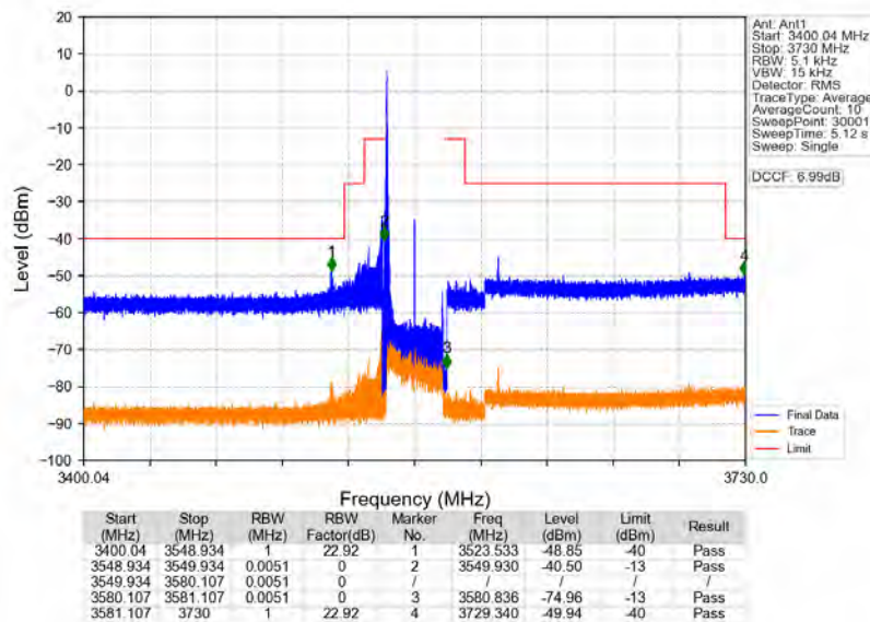
n78d 30kHz MIMO_NTNV_30MHz_CP-OFDM QPSK_3565.02MHz_Edge_1RB_Left
