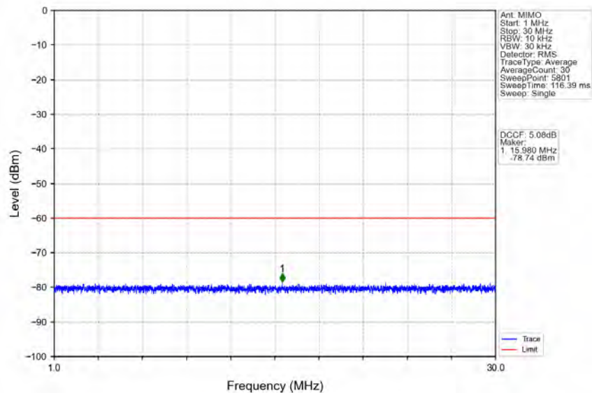
n78d_30kHz_MIMO_NTNV_15MHz_CP-OFDM QPSK_3692.49MHz_Edge_1RB_Right
