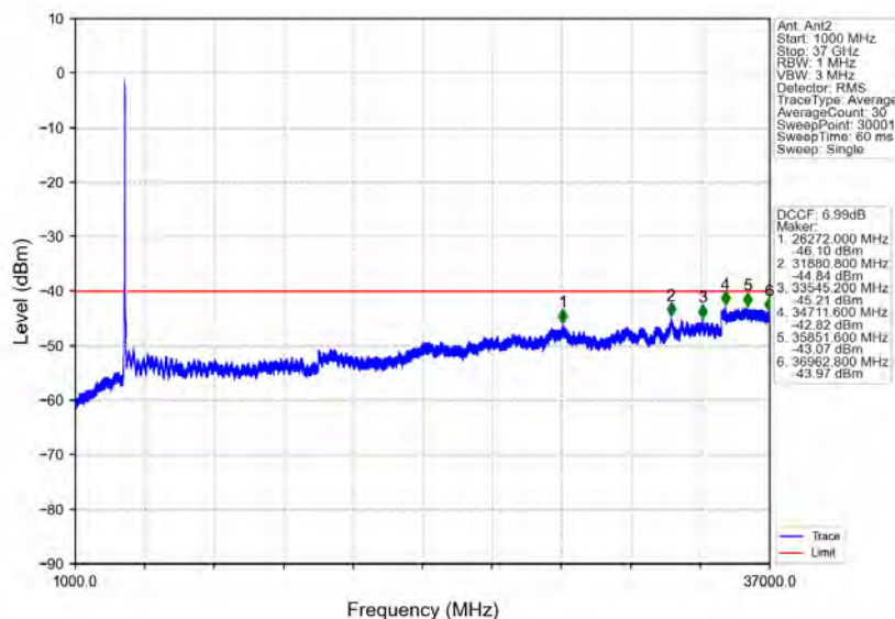
n78d_30kHz_MIMO_NTNV_30MHz_CP-OFDM_QPSK_3565.02MHz_Outer_Full
