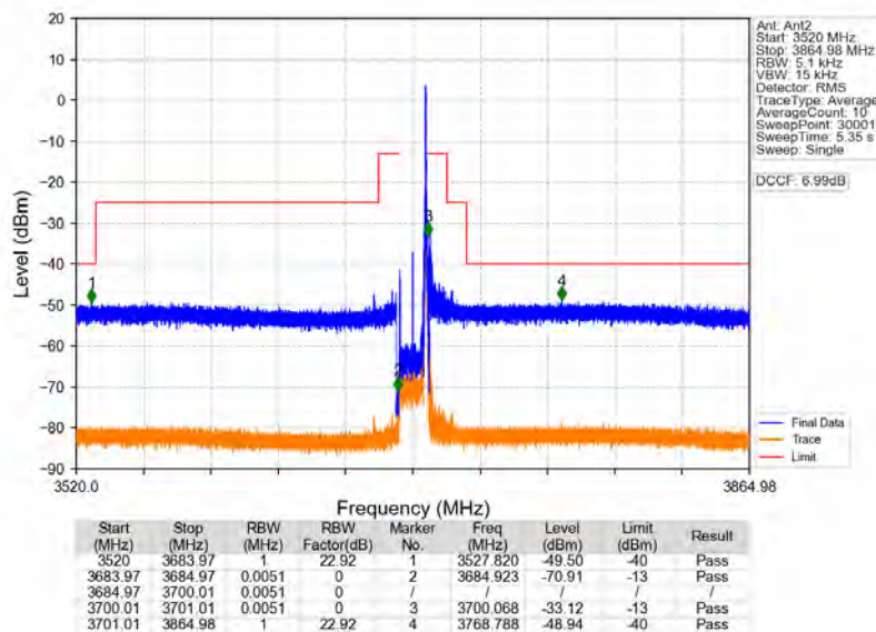
n78d_30kHz_MIMO_NTNV_15MHz_CP-OFDM_QPSK_3692.49MHz_Edge_1RB_Right
