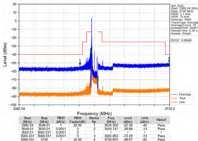
n78d_30kHz_MIMO_NTNV_15MHz_CP-OFDM_QPSK_3557.52MHz_Inner_1RB_Left
