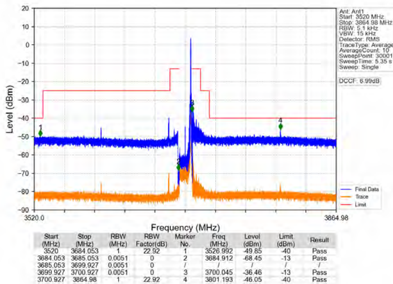
n78d_30kHz_MIMO_NTNV_15MHz_CP-OFDM_QPSK_3692.49MHz_Inner_1RB_Right
