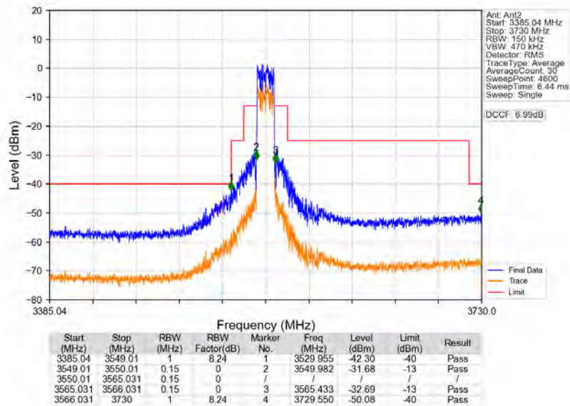
n78d_30kHz_MIMO_NTNV_15MHz_CP-OFDM_QPSK_3557.52MHz_Outer_Full
