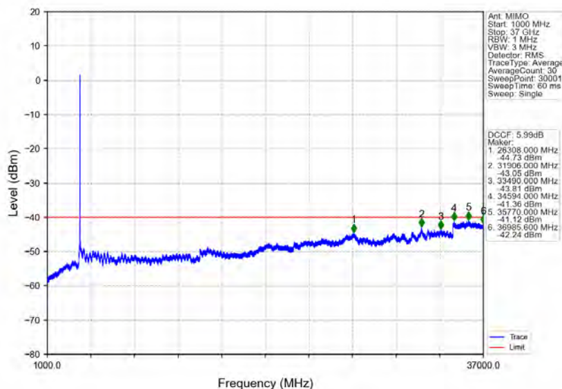
n78d_30kHz_MIMO_NTNV_20MHz_CP-OFDM_QPSK_3690MHz_Inner_1RB_Right
