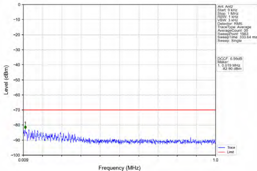
n78d_30kHz_MIMO_NTNV_10MHz_CP-OFDM_QPSK_3694.98MHz_Inner_1RB_Right
