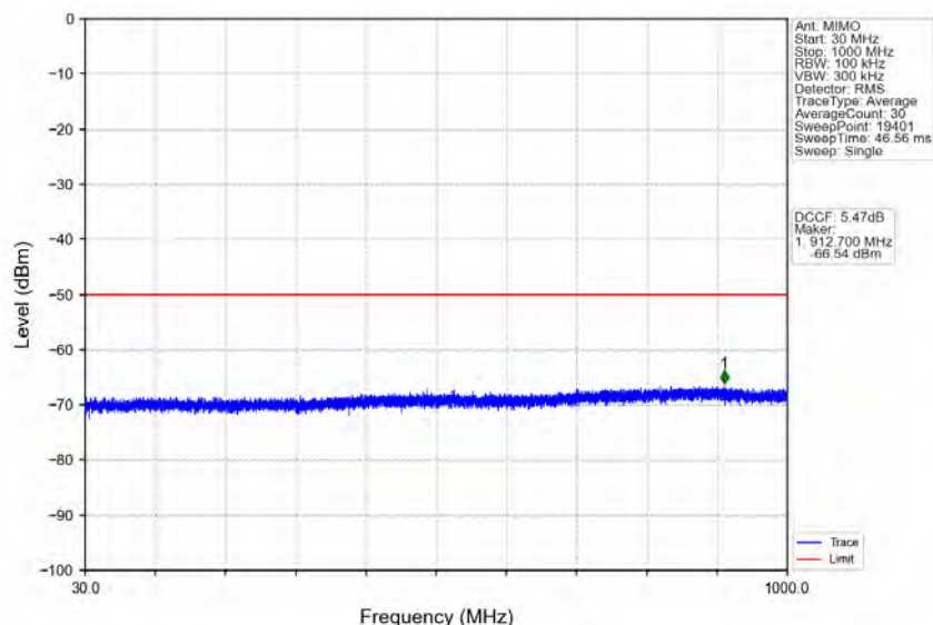
n78d_30kHz_MIMO_NTNV_15MHz_CP-OFDM_QPSK_3692.49MHz_Outer_Full
