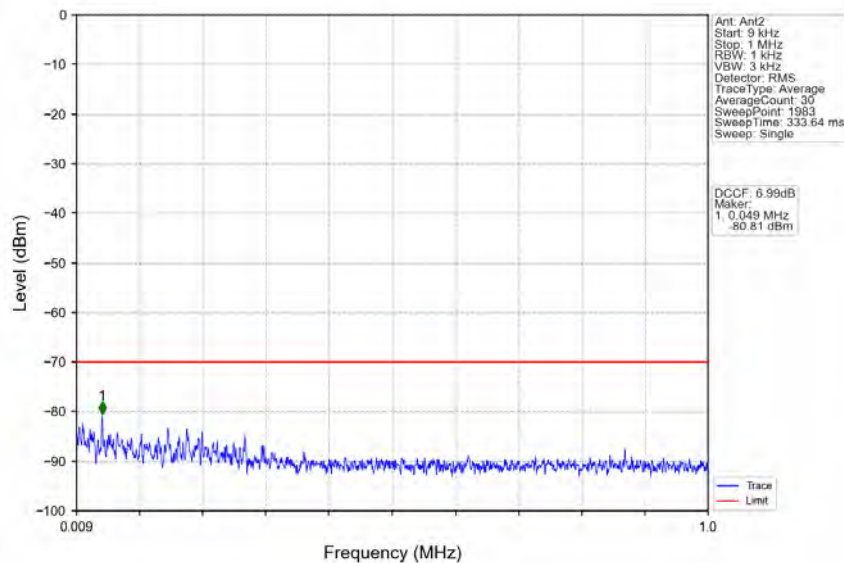
n78d_30kHz_MIMO_NTNV_20MHz_CP-OFDM_QPSK_3690MHz_Inner_1RB_Right
