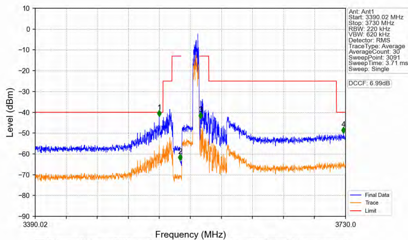
n78d_30kHz_MIMO_NTNV_20MHz_CP-OFDM_QPSK_3560.01MHz_Outer_Full
