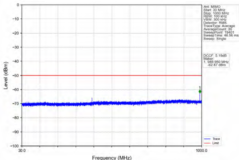
n78d_30kHz_MIMO_NTNV_10MHz_CP-OFDM QPSK_3555MHz_Inner_1RB_Left
