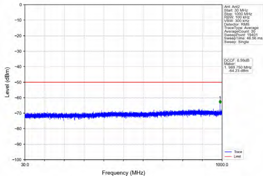
n78d_30kHz_MIMO_NTNV_20MHz_CP-OFDM_QPSK_3560.01MHz_Edge_1RB_Left
