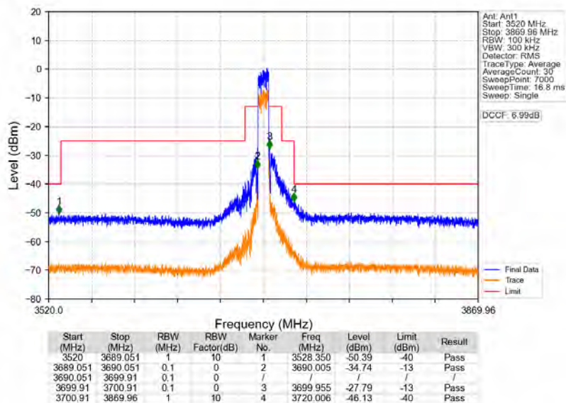
n78d_30kHz_MIMO_NTNV_10MHz_CP-OFDM_QPSK_3694.98MHz_Outer_Full
