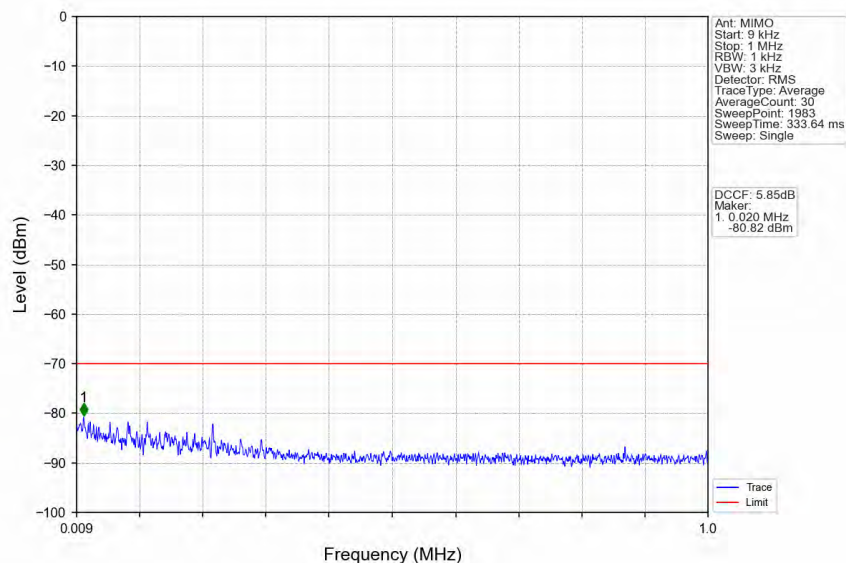
n78d_30kHz_MIMO_NTNV_20MHz_CP-OFDM QPSK_3690MHz_Edge_1RB_Right
