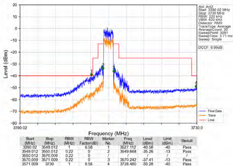
n78d_30kHz_MIMO_NTNV_20MHz_CP-OFDM_QPSK_3560.01MHz_Outer_Full
