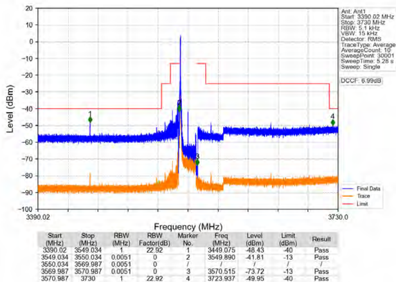
n78d_30kHz_MIMO_NTNV_20MHz_CP-OFDM_QPSK_3560.01MHz_Inner_1RB_Left
