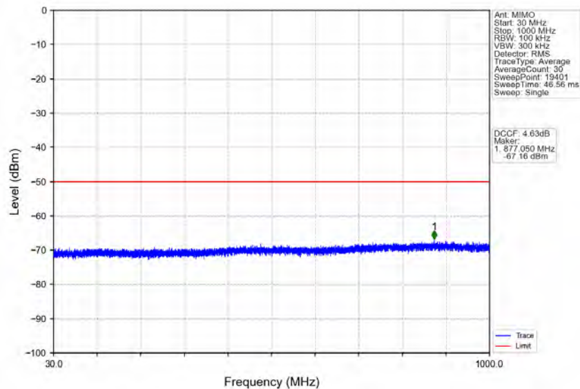
n78d_30kHz_MIMO_NTNV_10MHz_CP-OFDM QPSK_3694.98MHz_Outer_Full
