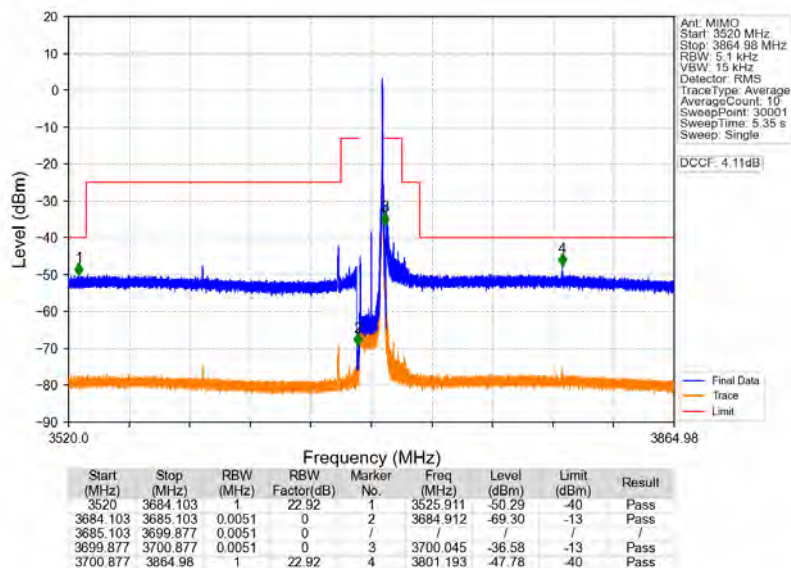
n78d 30kHz MIMO NTNV 15MHz CP-OFDM QPSK 3692.49MHz Inner 1RB Right
