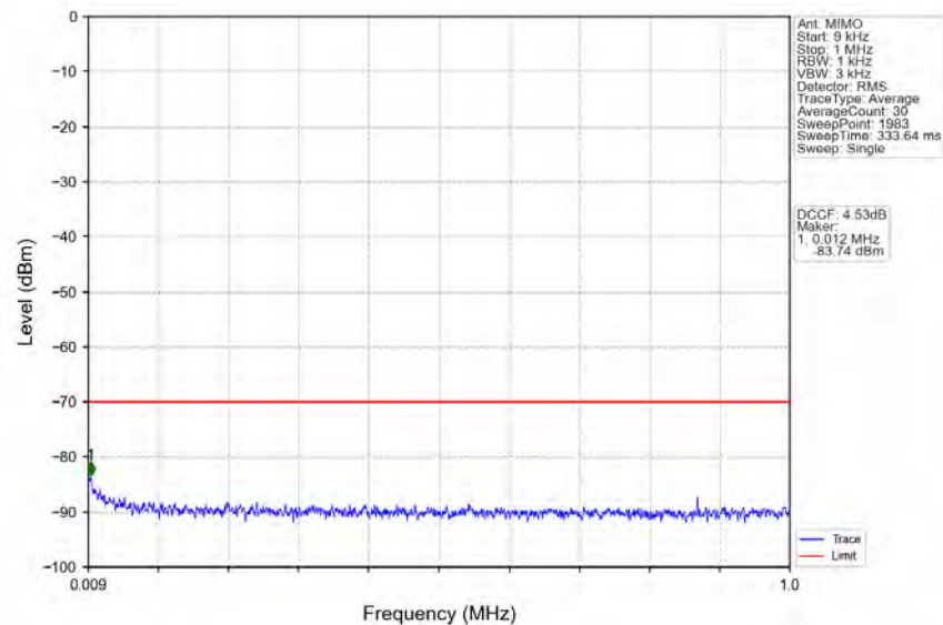
n78d_30kHz_MIMO_NTNV_20MHz_CP-OFDM_QPSK_3560.01MHz_Outer_Full
