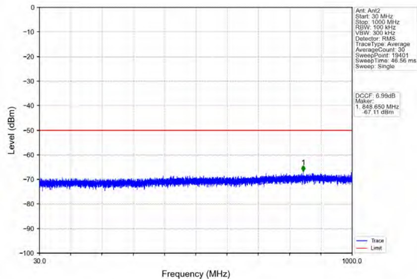
n78d_30kHz_MIMO_NTNV_15MHz_CP-OFDM_QPSK_3557.52MHz_Outer_Full
