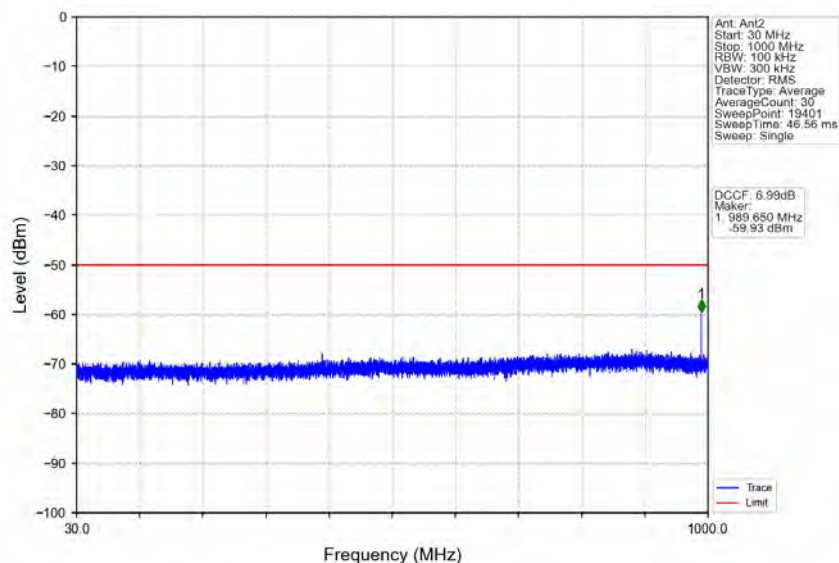
n78d_30kHz_MIMO_NTNV_15MHz_CP-OFDM_QPSK_3557.52MHz_Edge_1RB_Left
