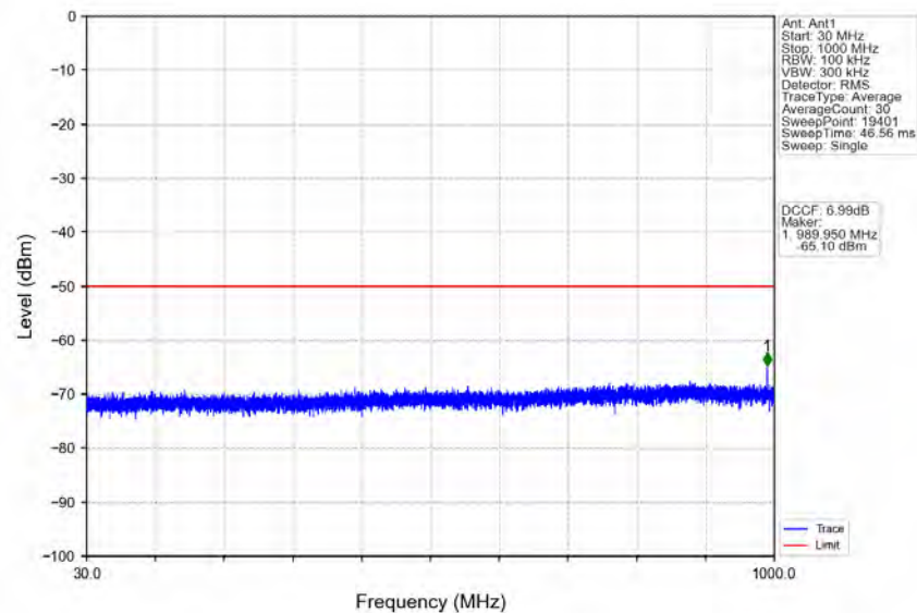
n78d_30kHz_MIMO_NTNV_15MHz_CP-OFDM_QPSK_3557.52MHz_Inner_1RB_Left
