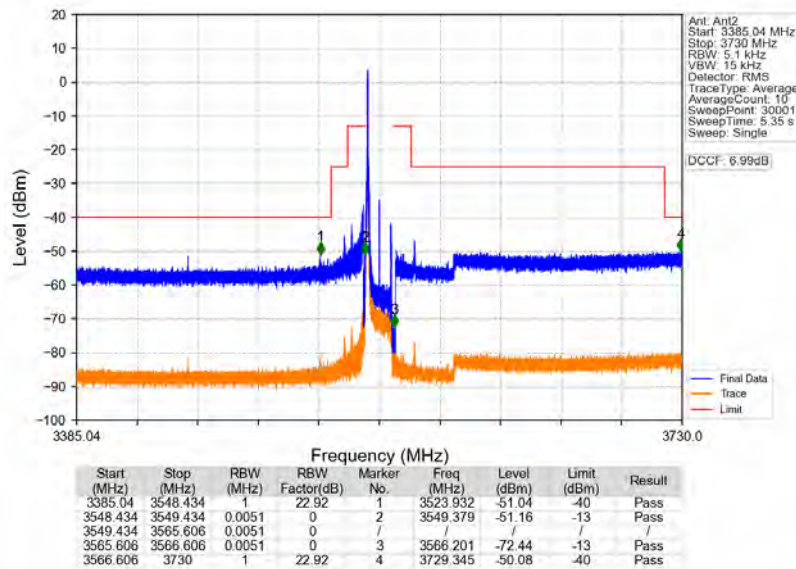
n78d_30kHz_MIMO_NTNV_15MHz_CP-OFDM_QPSK_3557.52MHz_Edge_1RB_Left
