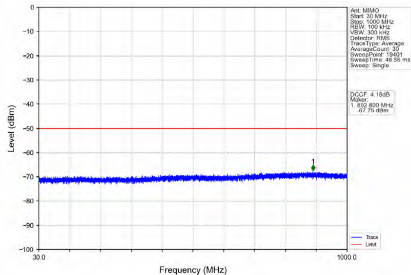
n78d_30kHz_MIMO_NTNV_60MHz_CP-OFDM QPSK_3669.99MHz_Inner_1RB_Right
