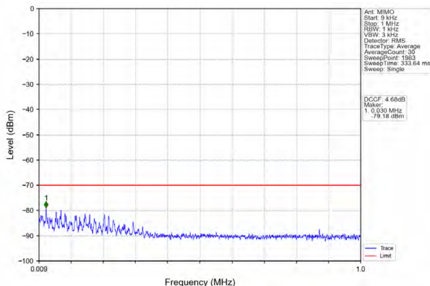
n78d_30kHz_MIMO_NTNV_60MHz_CP-OFDM_QPSK_3580.02MHz_Inner_1RB_Left
