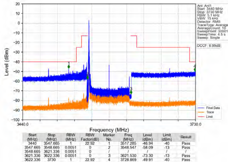
n78d 30kHz MIMO_NTNV_70MHz_CP-OFDM QPSK_3585MHz_Edge_1RB_Left
