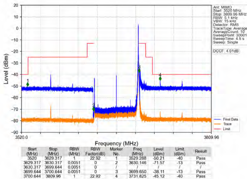
n78d_30kHz_MIMO_NTNV_70MHz_CP-OFDM_QPSK_3664.98MHz_Inner_1RB_Right
