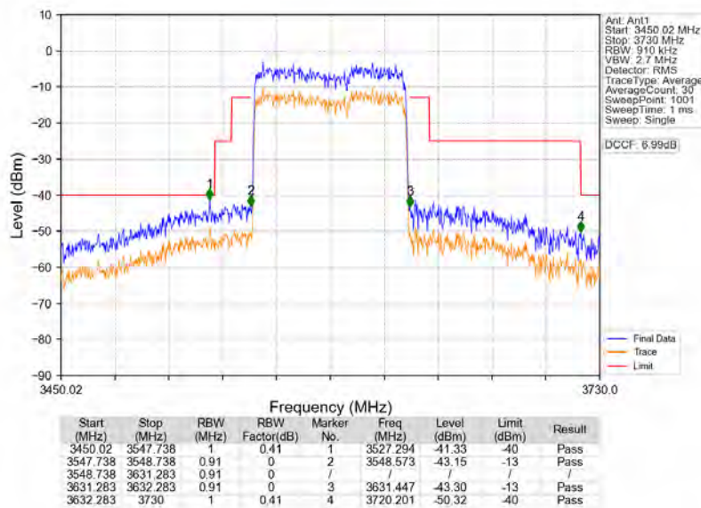
n78d_30kHz_MIMO_NTNV_80MHz_CP-OFDM_QPSK_3590.01MHz_Outer_Full
