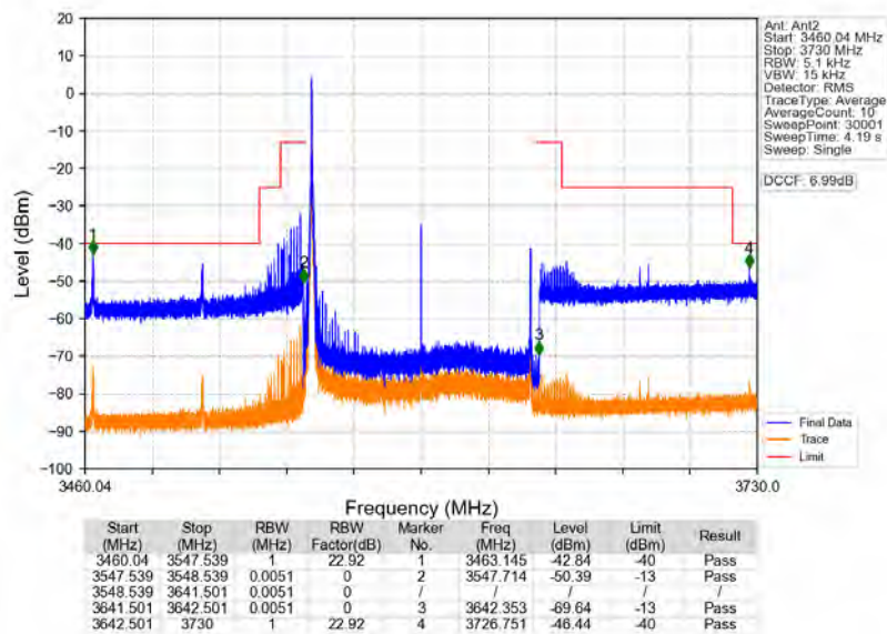
n78d_30kHz_MIMO_NTNV_90MHz_CP-OFDM_QPSK_3595.02MHz_Edge_1RB_Left
