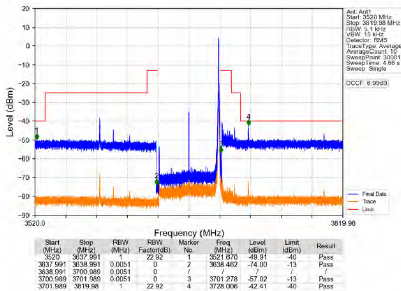
n78d_30kHz_MIMO_NTNV_60MHz_CP-OFDM_QPSK_3669.99MHz_Edge_1RB_Right
