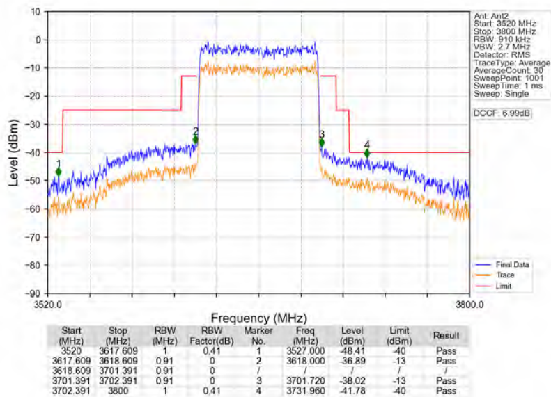
n78d_30kHz_MIMO_NTNV_80MHz_CP-OFDM_QPSK_3660MHz_Outer_Full
