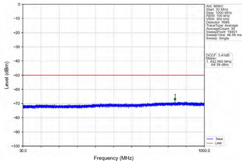
n78d_30kHz_MIMO_NTNV_70MHz_CP-OFDM QPSK_3664.98MHz_Edge_1RB_Right
