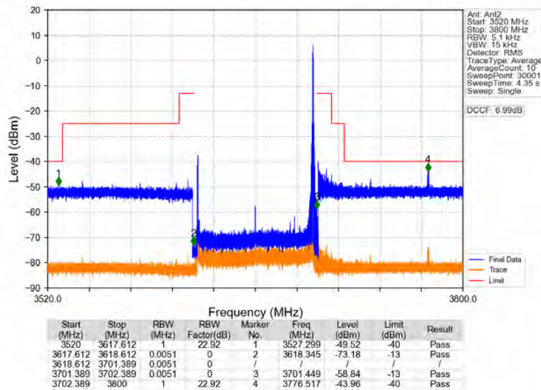
n78d_30kHz_MIMO_NTNV_80MHz_CP-OFDM_QPSK_3660MHz_Edge_1RB_Right
