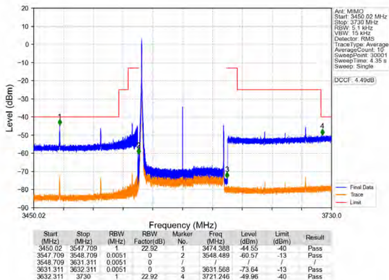
n78d_30kHz_MIMO_NTNV_80MHz_CP-OFDM_QPSK_3590.01MHz_Inner_1RB_Left
