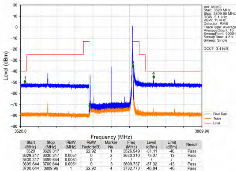
n78d_30kHz_MIMO_NTNV_70MHz_CP-OFDM_QPSK_3664.98MHz_Edge_1RB_Right
