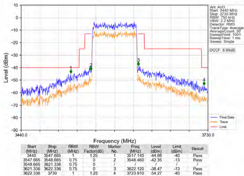
n78d_30kHz_MIMO_NTNV_70MHz_CP-OFDM QPSK_3585MHz_Outer_Full
