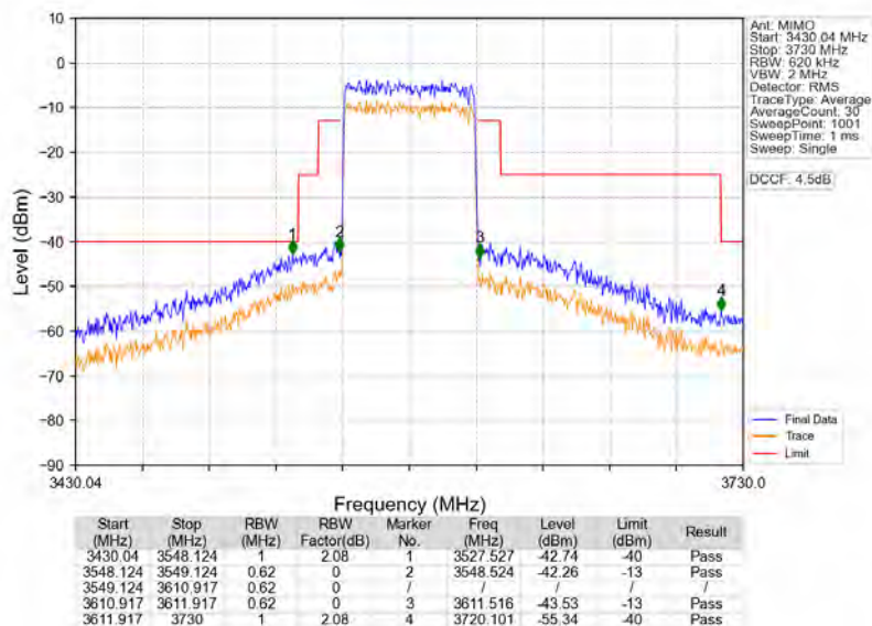
n78d_30kHz_MIMO_NTNV_60MHz_CP-OFDM_QPSK_3580.02MHz_Outer_Full
