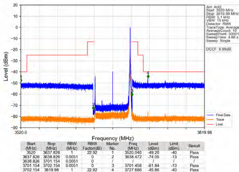
n78d_30kHz_MIMO_NTNV_60MHz_CP-OFDM_QPSK_3669.99MHz_Inner_1RB_Right
