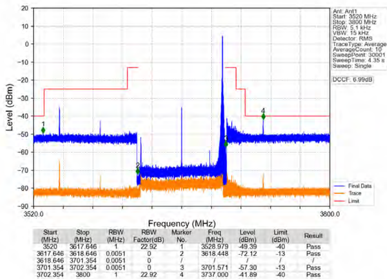
n78d_30kHz_MIMO_NTNV_80MHz_CP-OFDM_QPSK_3660MHz_Inner_1RB_Right
