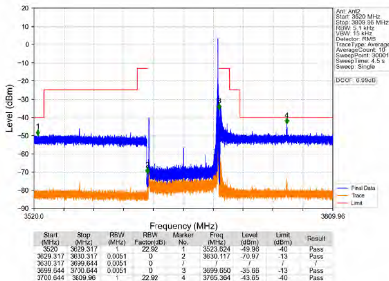
n78d_30kHz_MIMO_NTNV_70MHz_CP-OFDM_QPSK_3664.98MHz_Inner_1RB_Right
