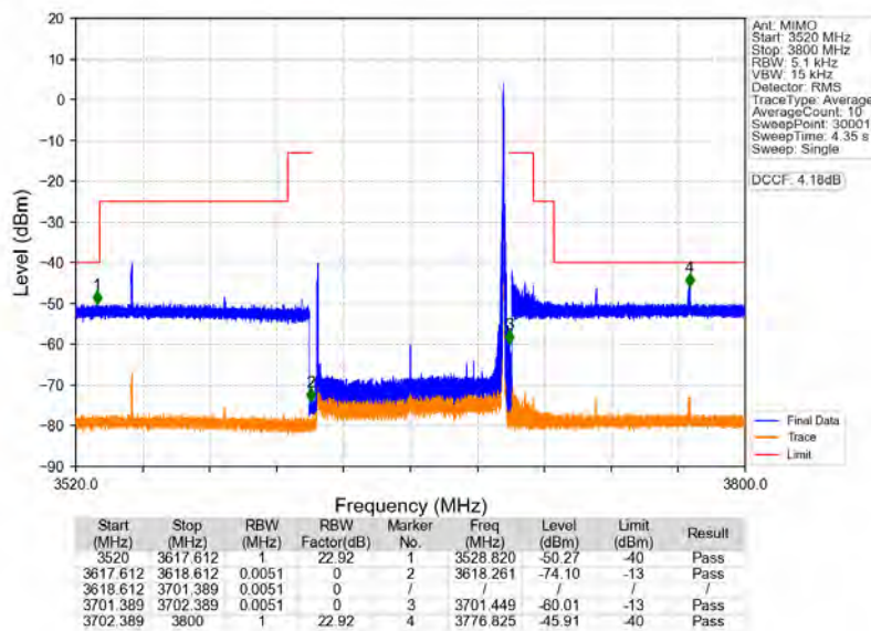
n78d_30kHz_MIMO_NTNV_80MHz_CP-OFDM_QPSK_3660MHz_Edge_1RB_Right
