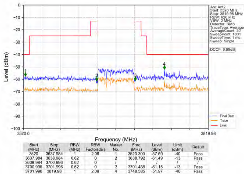
n78d_30kHz_MIMO_NTNV_60MHz_CP-OFDM_QPSK_3669.99MHz_Outer_Full
