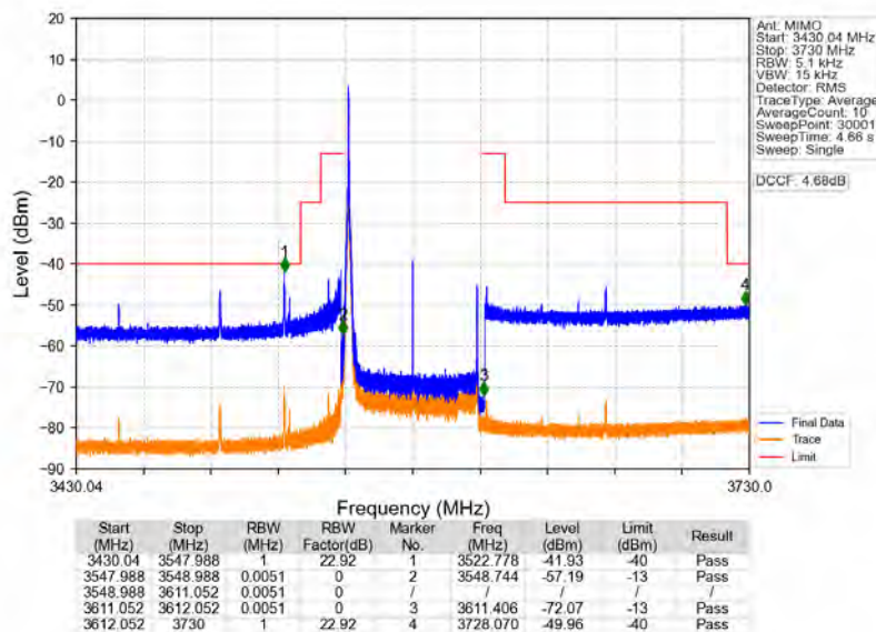
n78d_30kHz_MIMO_NTNV_60MHz_CP-OFDM_QPSK_3580.02MHz_Inner_1RB_Left
