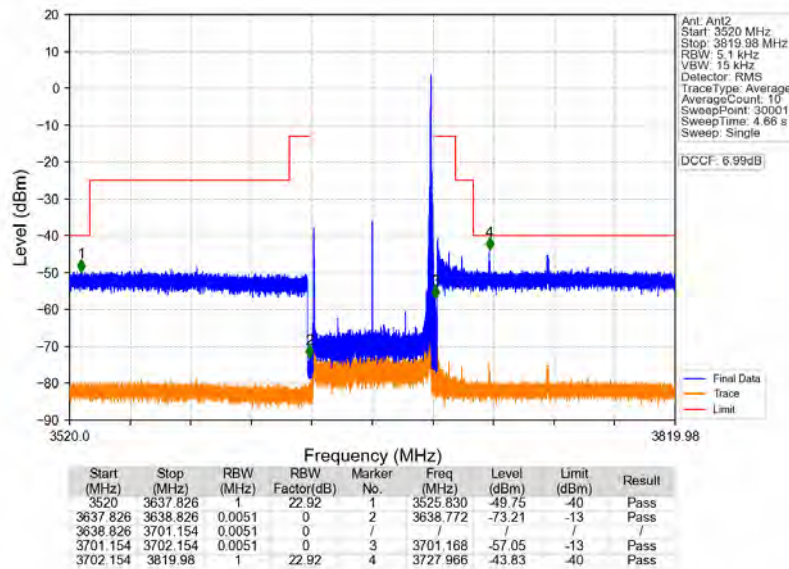
n78d_30kHz_MIMO_NTNV_60MHz_CP-OFDM_QPSK_3669.99MHz_Edge_1RB_Right
