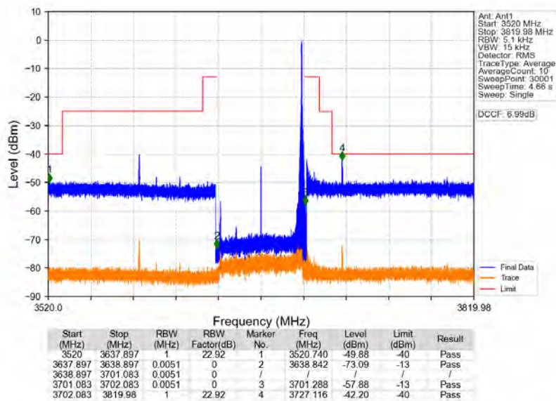
n78d_30kHz_MIMO_NTNV_60MHz_CP-OFDM_QPSK_3669.99MHz_Inner_1RB_Right
