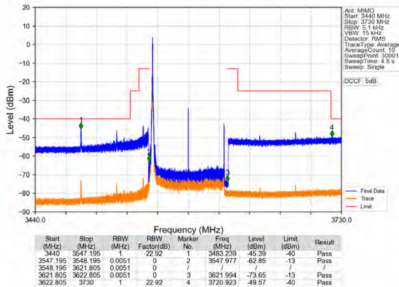
n78d_30kHz_MIMO_NTNV_70MHz_CP-OFDM_QPSK_3585MHz_Edge_1RB_Left
