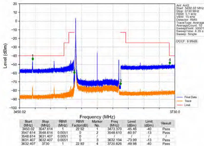
n78d_30kHz_MIMO_NTNV_80MHz_CP-OFDM_QPSK_3590.01MHz_Edge_1RB_Left
