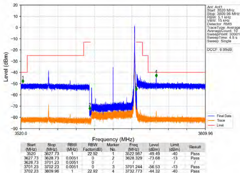
n78d_30kHz_MIMO_NTNV_70MHz_CP-OFDM QPSK_3664.98MHz_Edge_1RB_Right
