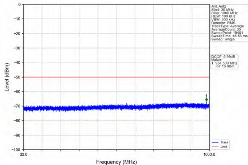
n78d_30kHz_MIMO_NTNV_80MHz_CP-OFDM_QPSK_3660MHz_Inner_1RB_Right
