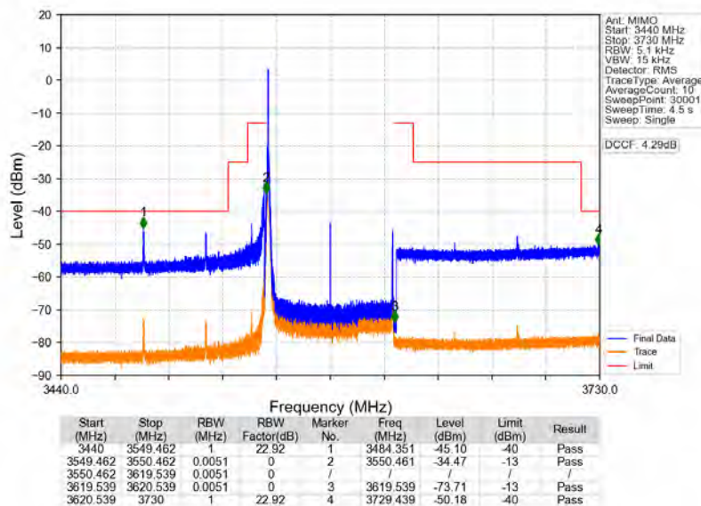
n78d_30kHz_MIMO_NTNV_70MHz_CP-OFDM_QPSK_3585MHz_Inner_1RB_Left
