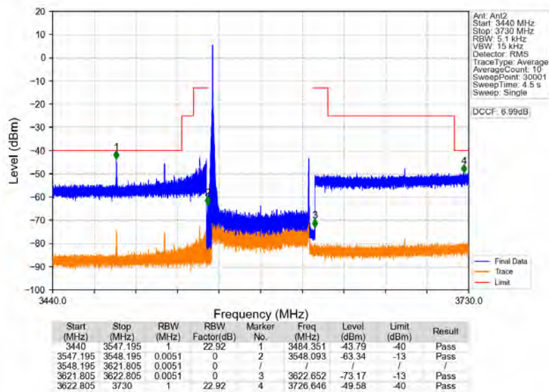
n78d_30kHz_MIMO_NTNV_70MHz_CP-OFDM_QPSK_3585MHz_Inner_1RB_Left
