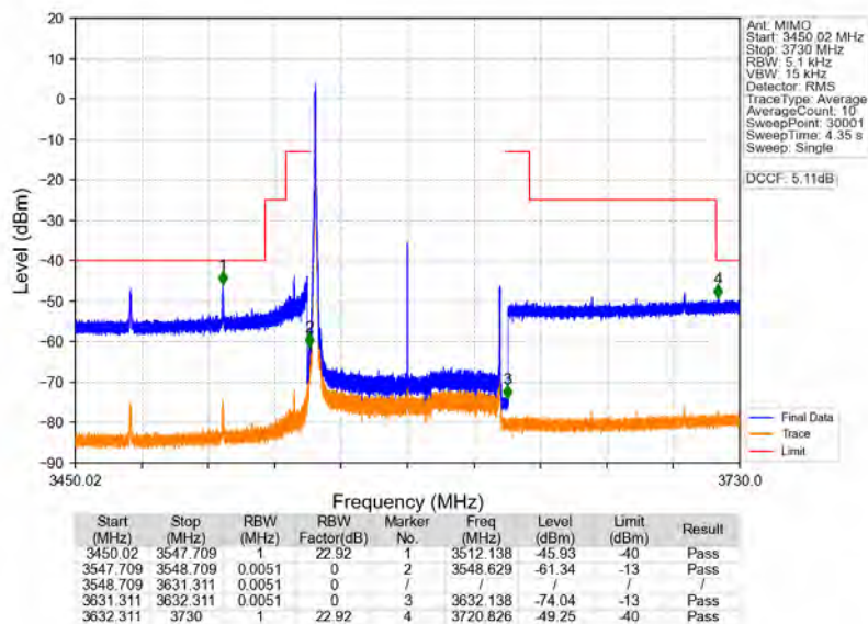
n78d_30kHz_MIMO_NTNV_80MHz_CP-OFDM_QPSK_3590.01MHz_Edge_1RB_Left
