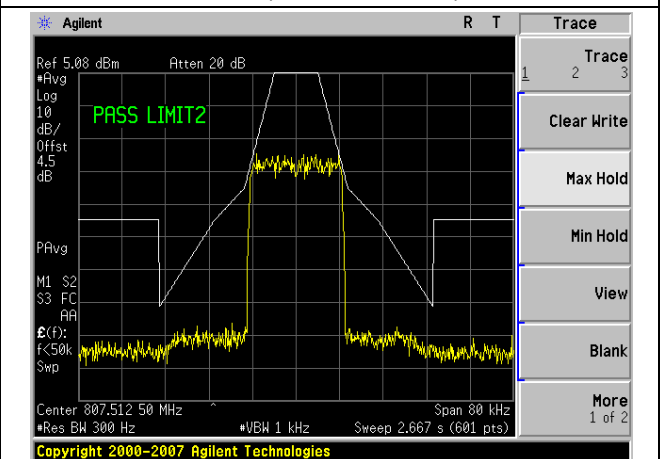
Mask(Highest channel)
