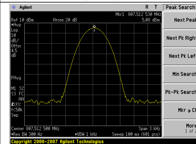
Unmodulated power (Highest channel)
