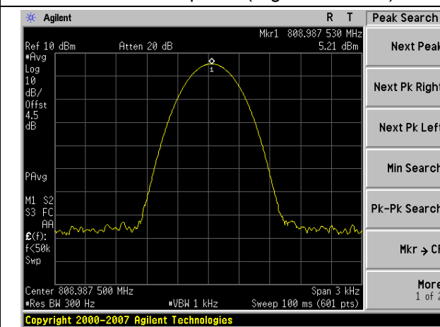
Unmodulated power (Highest channel)
