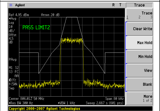
Mask(Middle channel)
