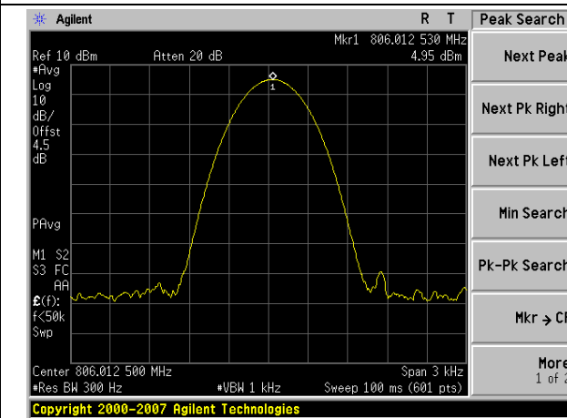
Unmodulated power (Middle channel)
