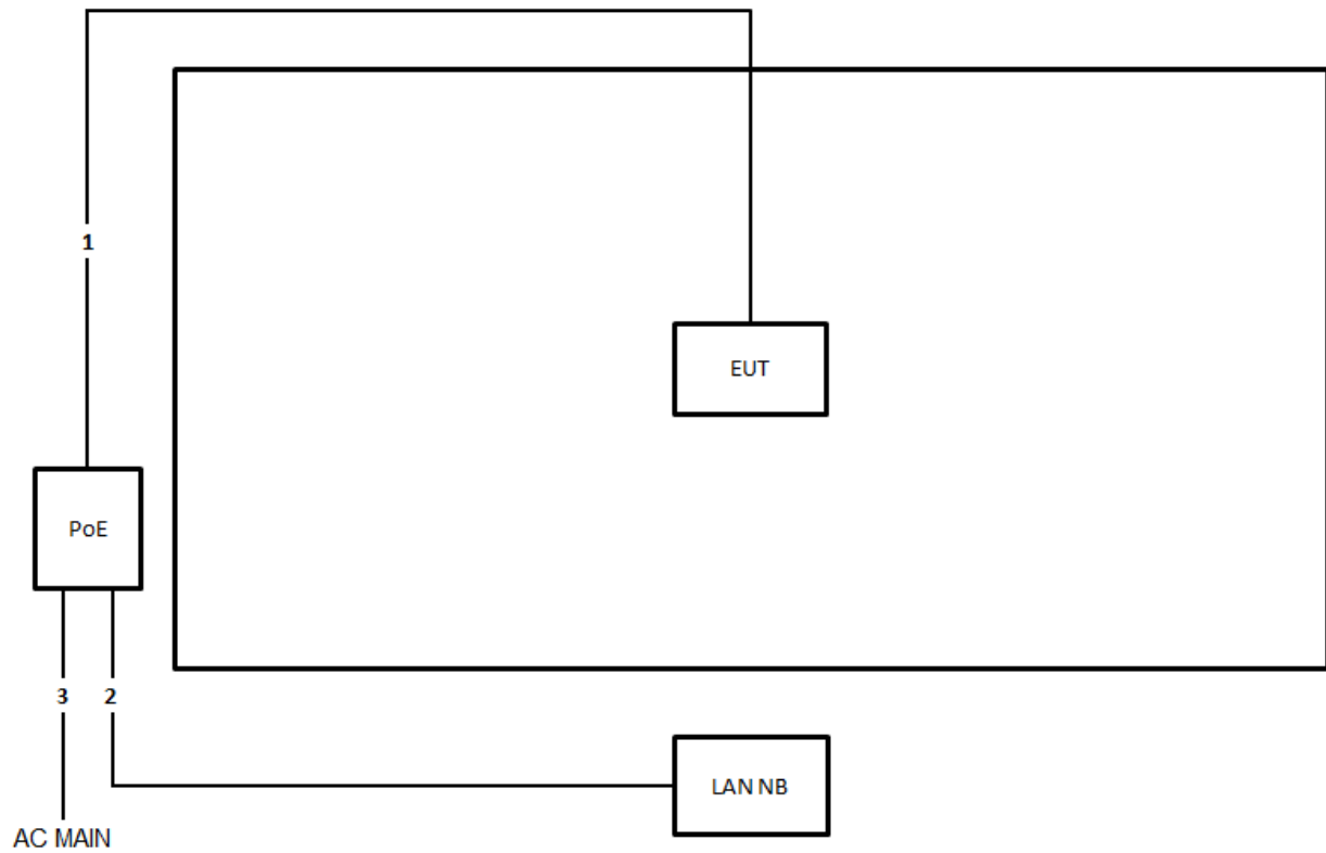
Test Setup Diagram - Radiated Test > 1GHz / For non-beamforming mode
