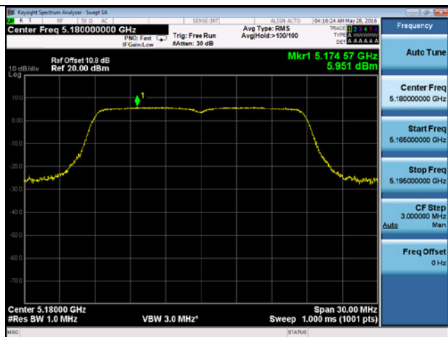
PSD-802.11n-20M -5180M-chain2
