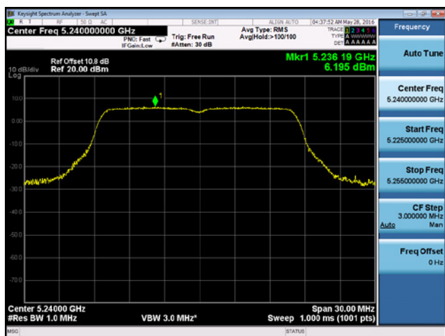
PSD-802.11a-5240M-chain3
