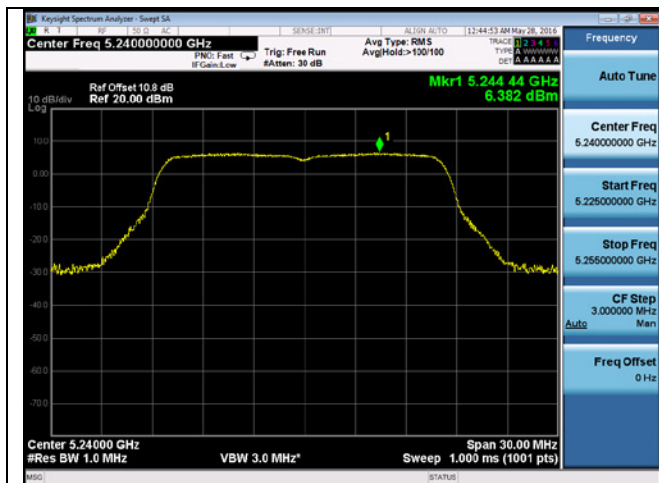
PSD-802.11a-5240M-chain1
