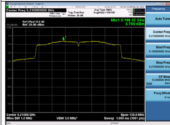
PSD-802.11ac-80M-5210M-chain3
