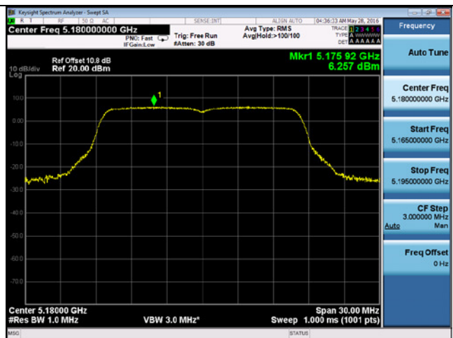
PSD-802.11n-20M -5180M-chain3
