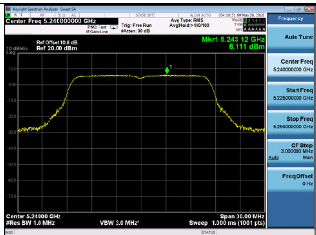
PSD-802.11a-5240M-chain2
