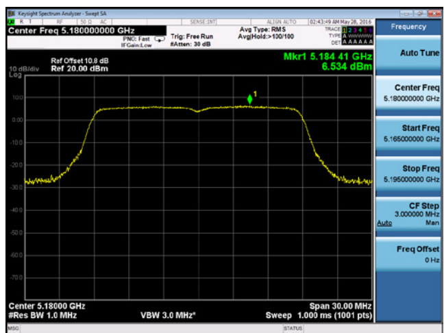
PSD-802.11n-20M -5180M-chain1
