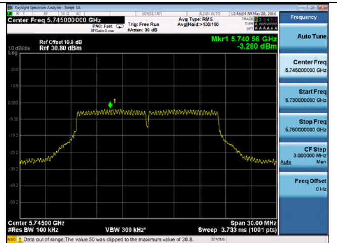
PSD-802.11a-5745M-chain1
