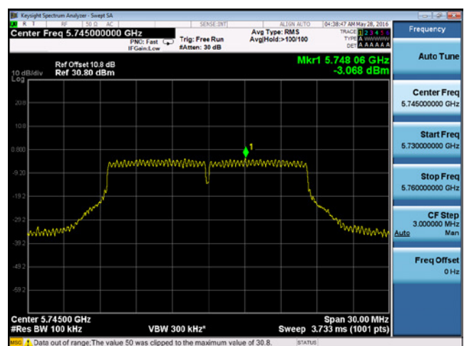
PSD-802.11a-5745M-chain3
