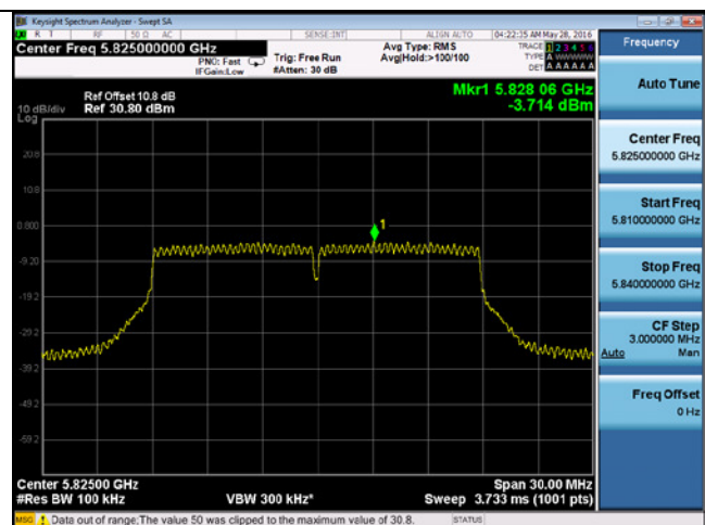
PSD-802.11n-20-5825M-chain2
