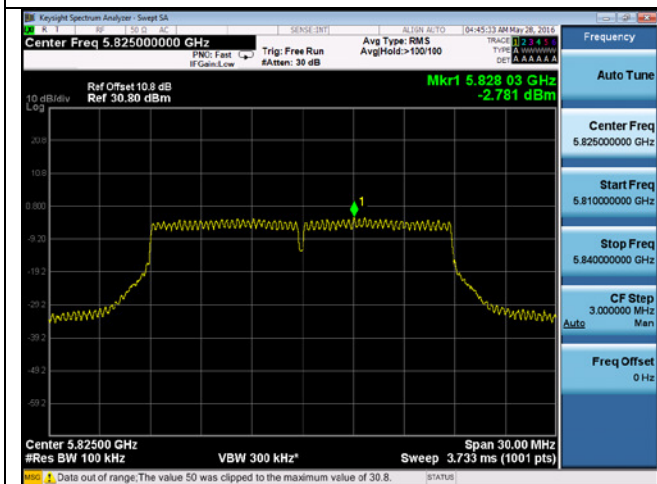
PSD-802.11n-20-5825M-chain3
