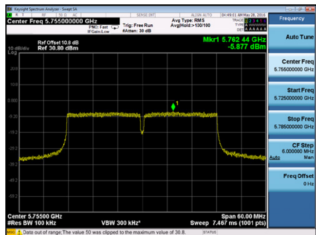
PSD-802.11n-40-5755M-chain3
