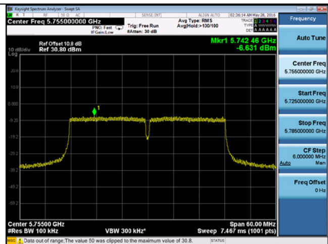
PSD-802.11n-40-5755M-chain1
