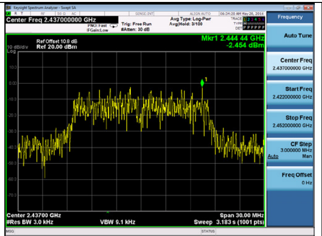
PSD-2.4G-802.11n-20M 2437MHz
