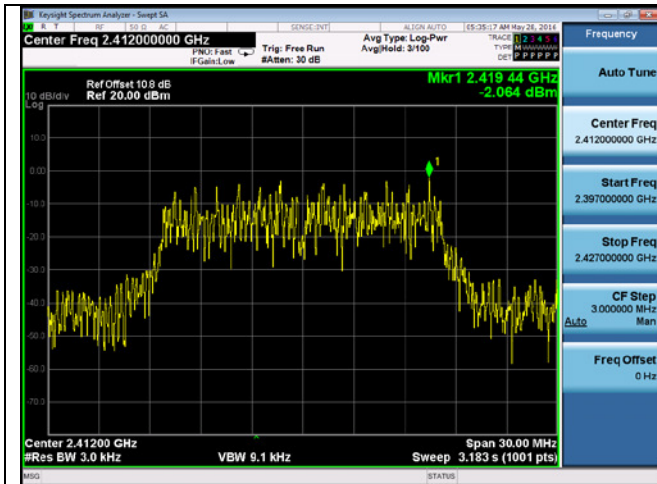
PSD-2.4G-802.11n-20M 2412MHz
