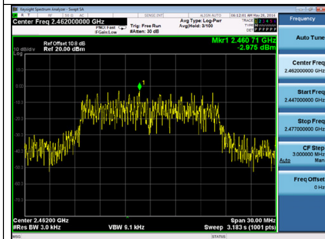
PSD-2.4G-802.11n-20M 2462MHz
