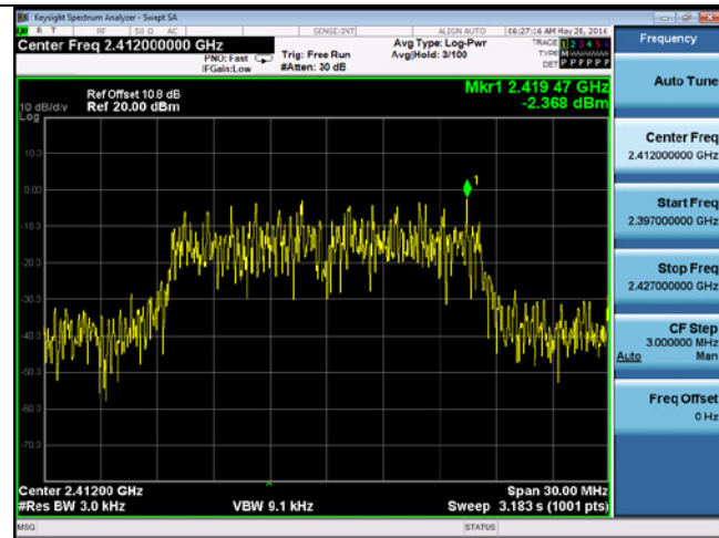
PSD-2.4G-802.11n-20M 2412MHz
