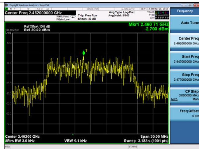
PSD-2.4G-802.11n-20M 2462MHz
