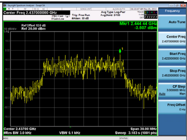
PSD-2.4G-802.11n-20M 2437MHz
