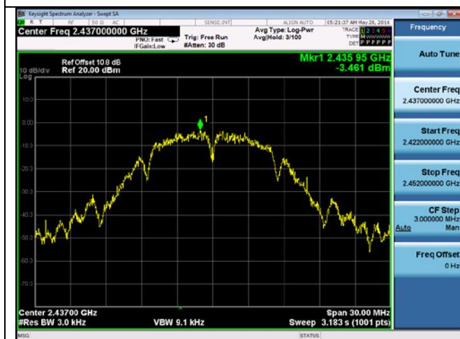
PSD-2.4G-802.11b 2437MHz
