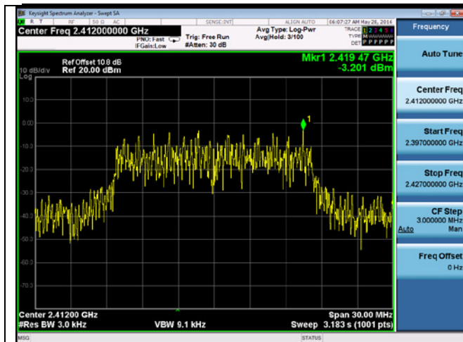
PSD-2.4G-802.11n-20M 2412MHz
