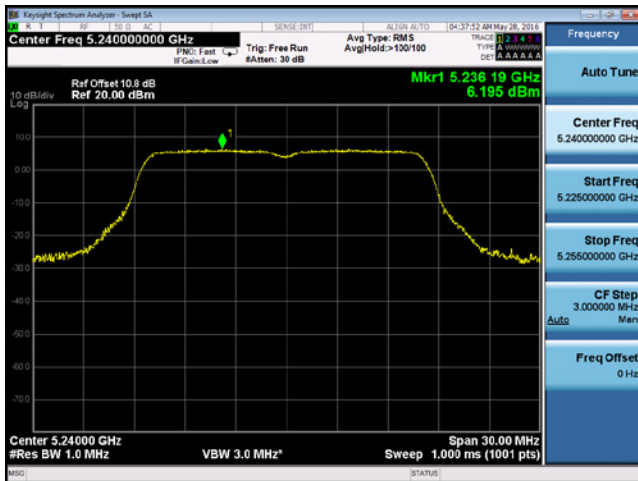
PSD-802.11a-5240M-chain3
