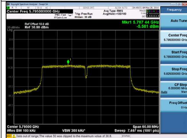
PSD-802.11n-40-5795M-chain3
