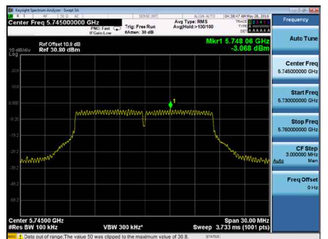
PSD-802.11a-5745M-chain3
