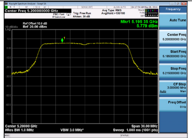
PSD-802.11n-20M-5200M-chain2
