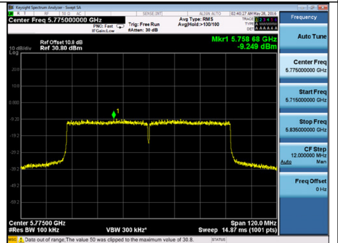
PSD-802.11ac-80-5775M-chain1
