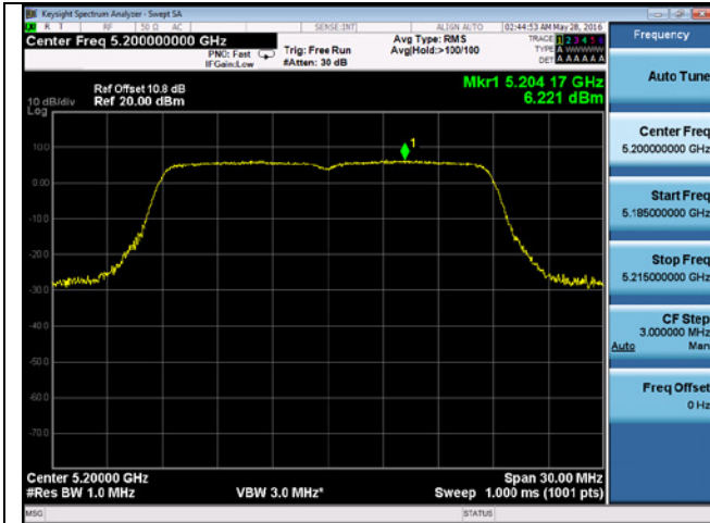
PSD-802.11n-20M-5200M-chain1
