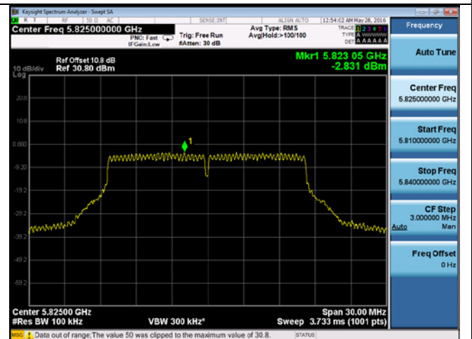
PSD-802.11a-5825M-chain1
