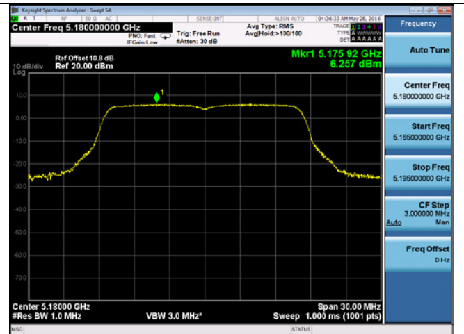
PSD-802.11n-20M -5180M-chain3
