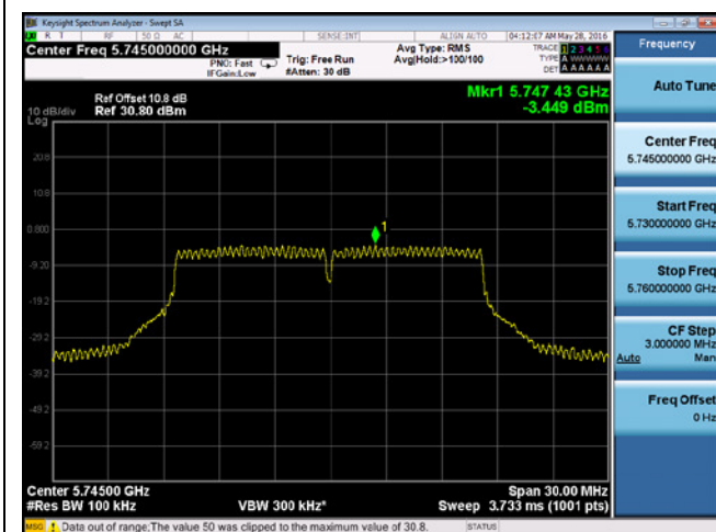
PSD-802.11a-5745M-chain2
