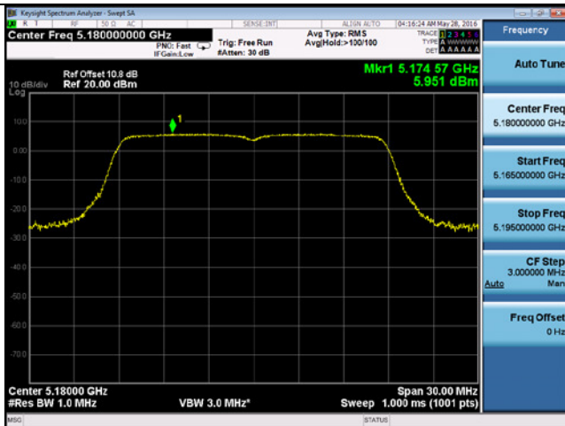
PSD-802.11n-20M -5180M-chain2
