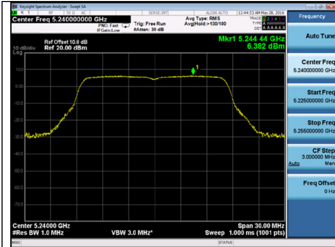
PSD-802.11a-5240M-chain1
