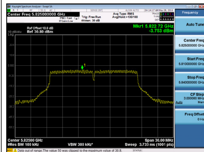
PSD-802.11a-5825M-chain2
