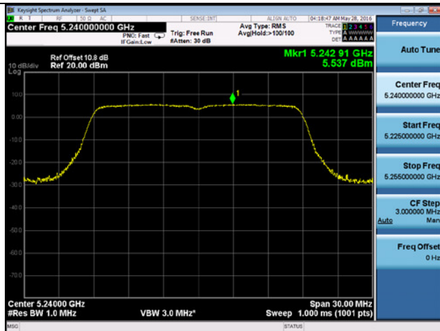
PSD-802.11n-20M-5240M-chain2
