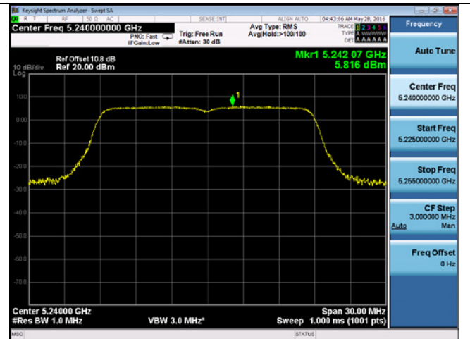
PSD-802.11n-20M-5240M-chain3
