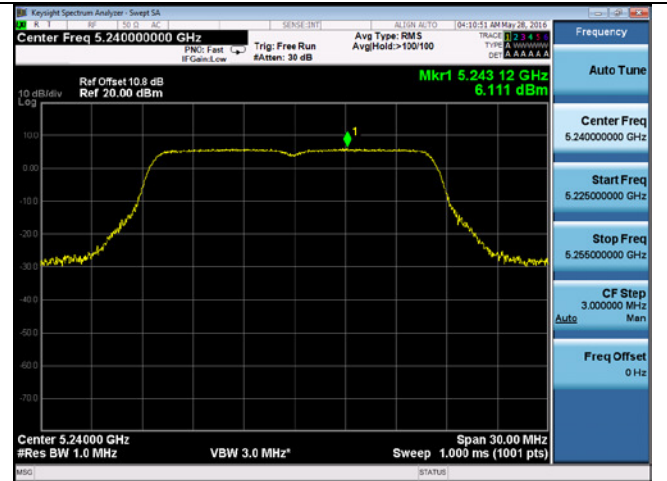
PSD-802.11a-5240M-chain2
