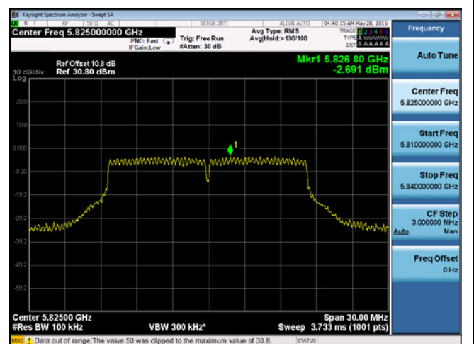
PSD-802.11a-5825M-chain3
