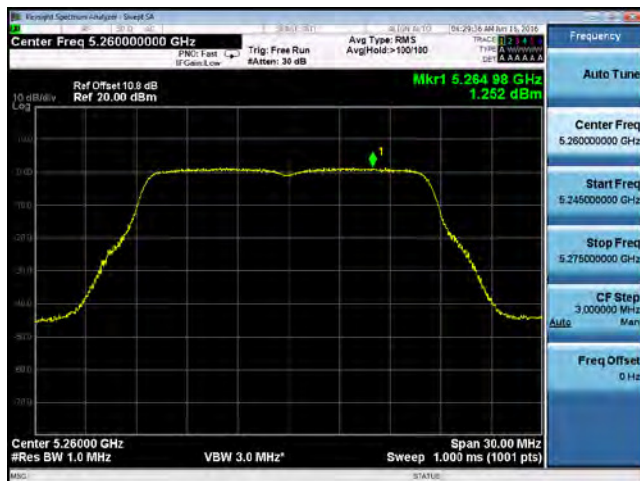
PSD-802.11a-5260M-chain3
