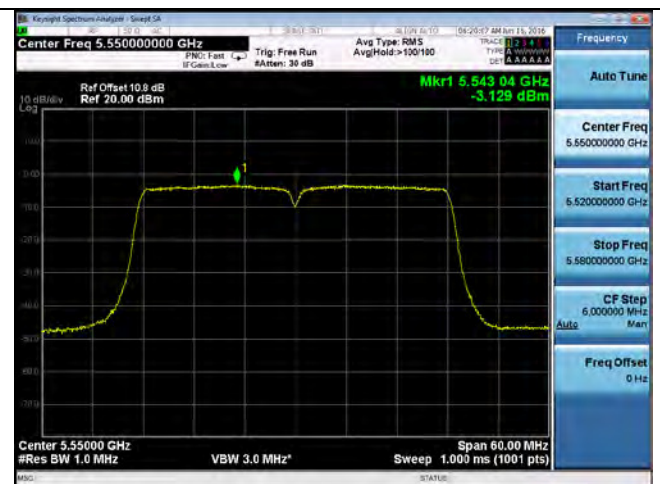
PSD-802.11n-40-5550M-chain2
