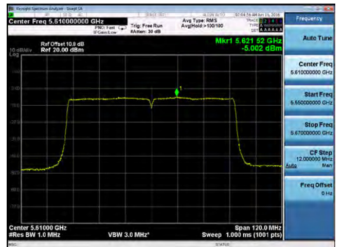
PSD-802.11ac-80-5610M-chain3
