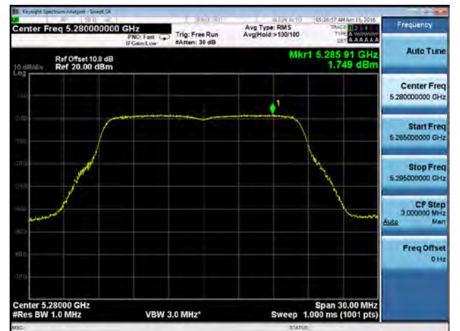
PSD-802.11a-5280M-chain1
