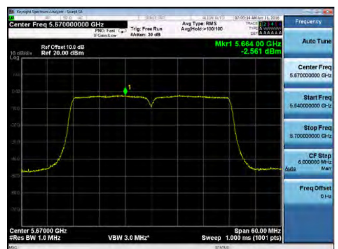
PSD-802.11n-40-5670M-chain3
