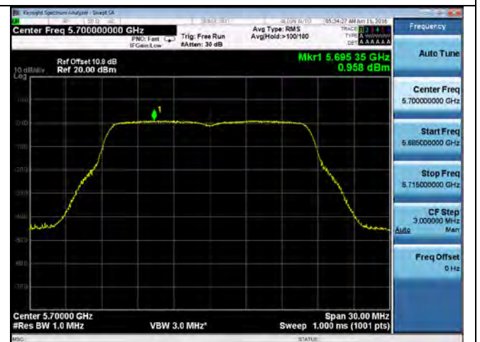
PSD-802.11a-5700M-chain1
