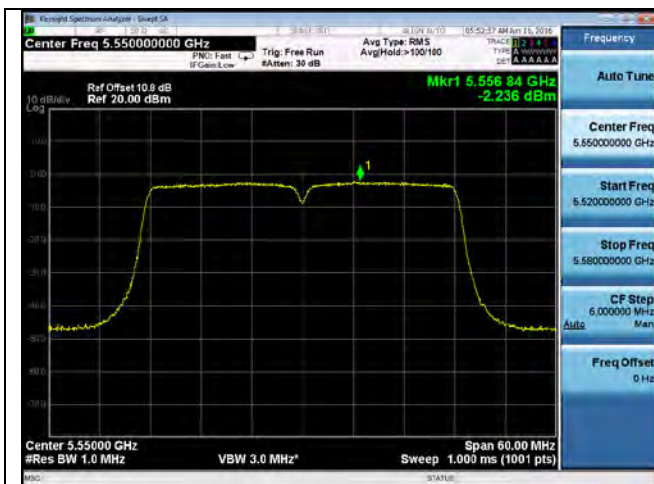
PSD-802.11n-40-5550M-chain1
