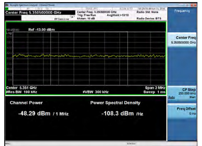
Band Edge-802.11a-5320M-chain1
