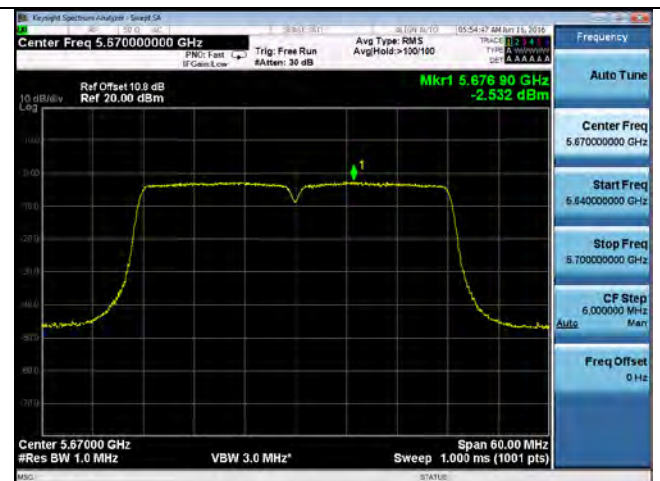
PSD-802.11n-40-5670M-chain1
