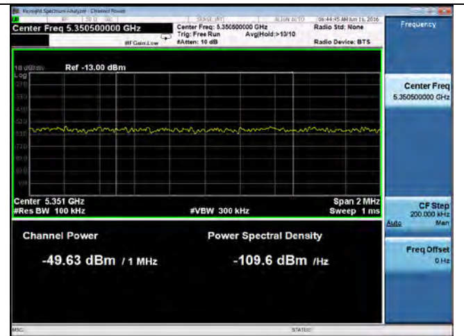
Band Edge-802.11a-5320M-chain3
