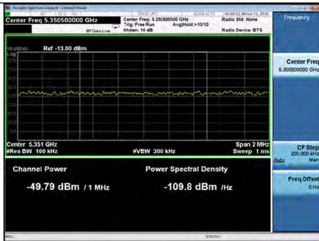
Band Edge-802.11a-5320M-chain2
