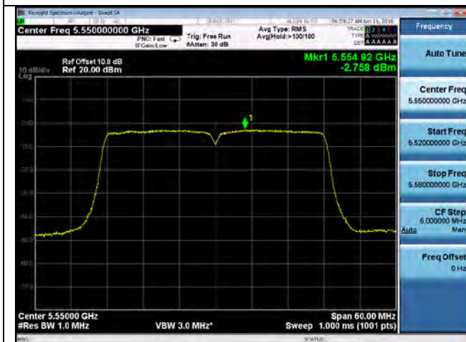
PSD-802.11n-40-5550M-chain3
