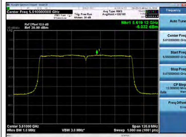
PSD-802.11ac-80-5610M-chain2
