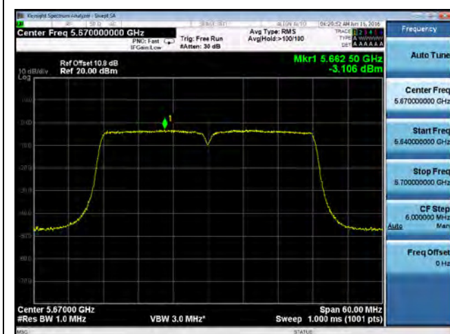
PSD-802.11n-40-5670M-chain2
