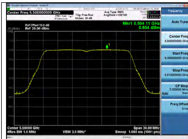
PSD-802.11n-20-5500M-chain1
