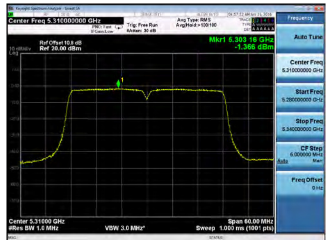
PSD-802.11n-40M-5310M-chain3
