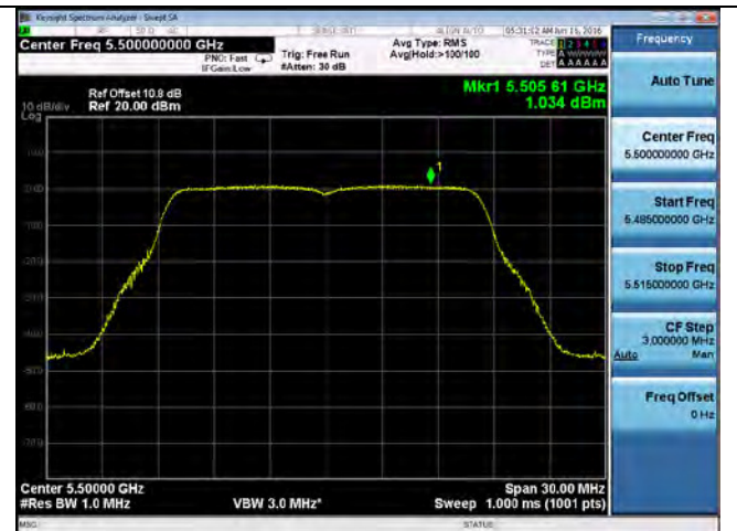
PSD-802.11a-5500M-chain1
