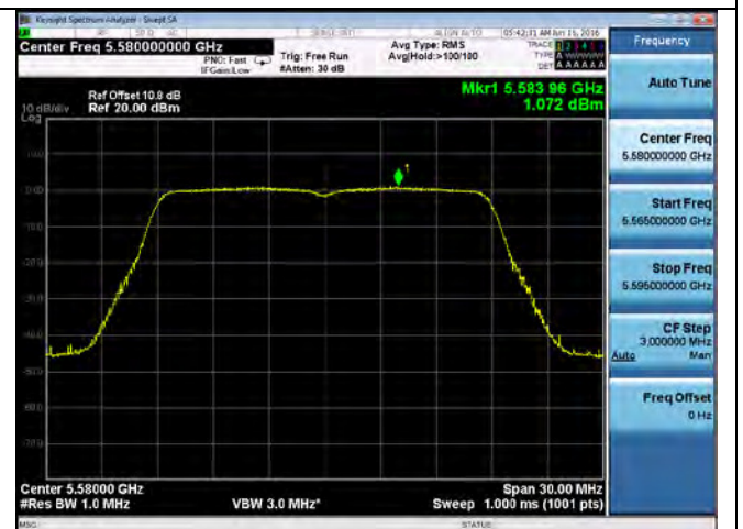
PSD-802.11n-20-5580M-chain1
