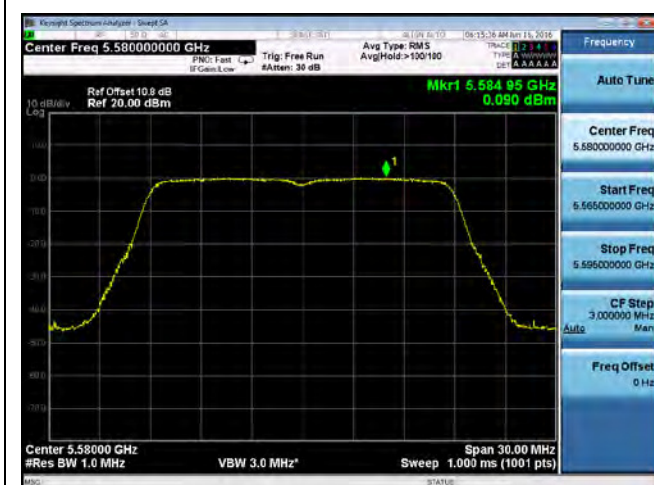
PSD-802.11n-20-5580M-chain2
