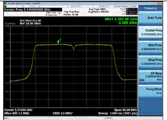
PSD-802.11n-40M-5310M-chain1
