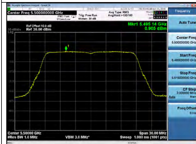
PSD-802.11n-20-5500M-chain3
