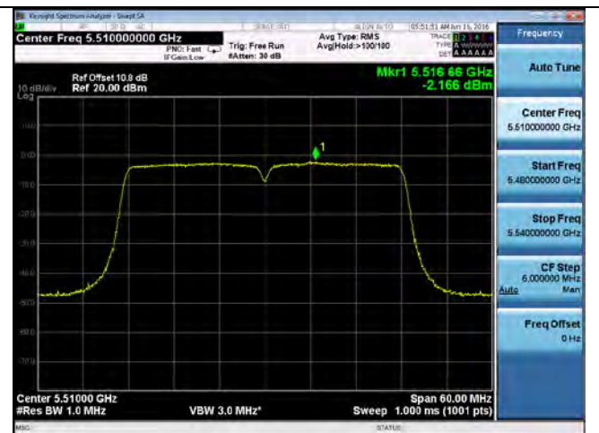
PSD-802.11n-40-5510M-chain1
