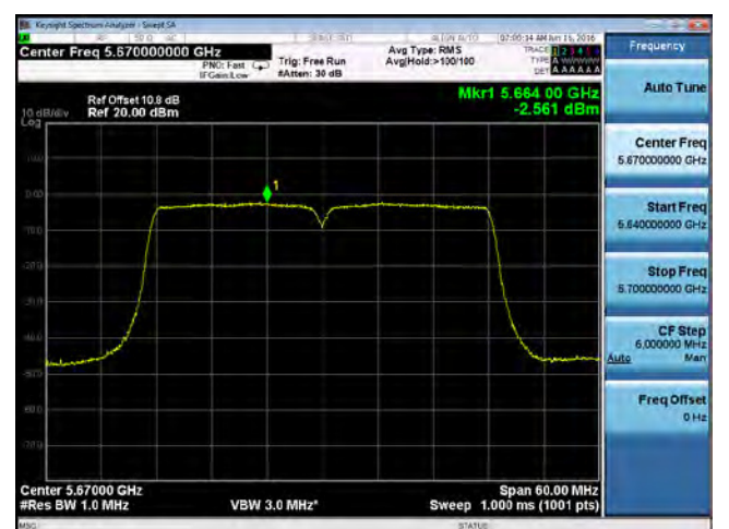
PSD-802.11n-40-5670M-chain3
