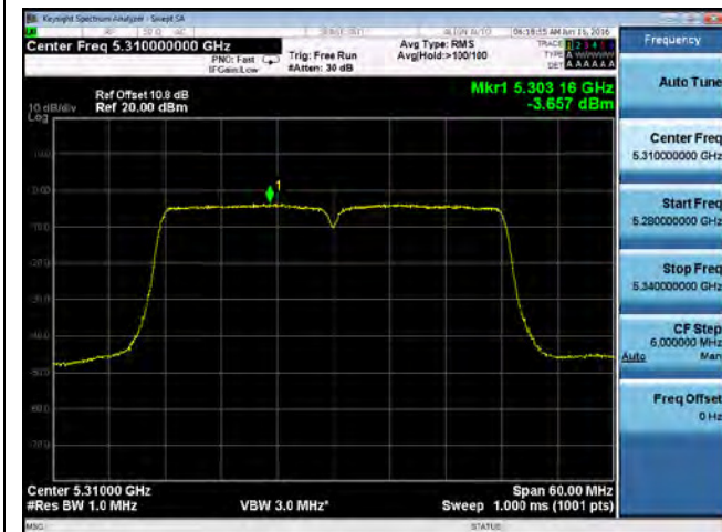
PSD-802.11n-40M-5310M-chain2
