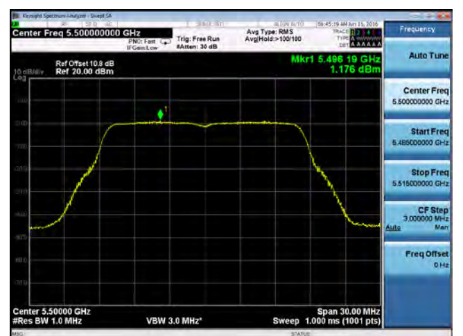
PSD-802.11a-5500M-chain3
