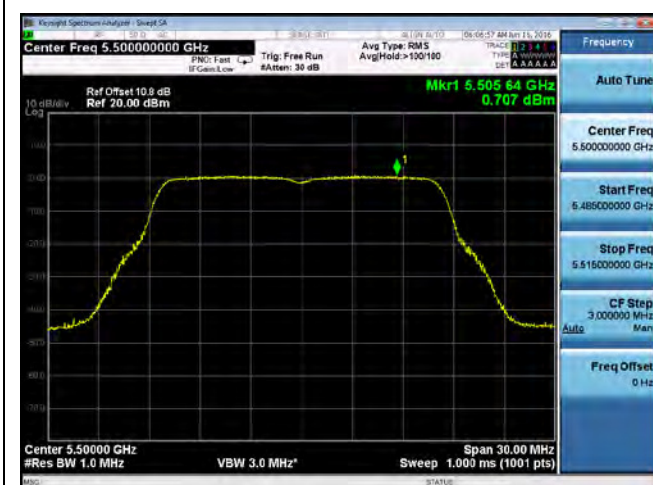
PSD-802.11a-5500M-chain2
