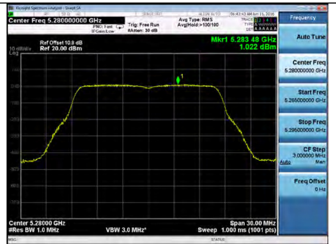
PSD-802.11a-5280M-chain3
