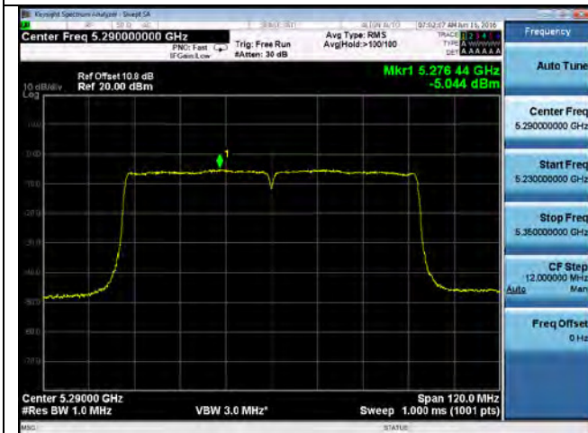
PSD-802.11ac-80M-5290M-chain3
