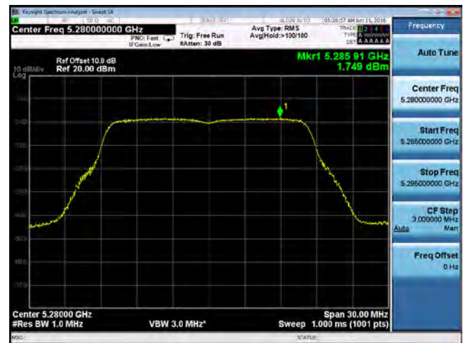
PSD-802.11a-5280M-chain1
