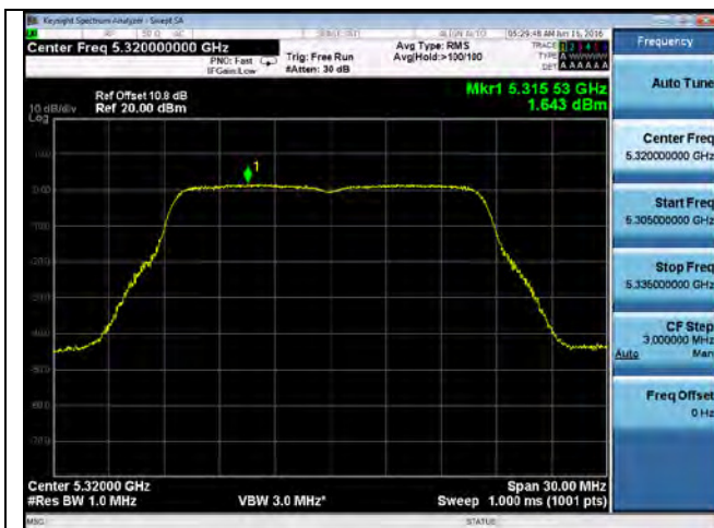
PSD-802.11a-5320M-chain1
