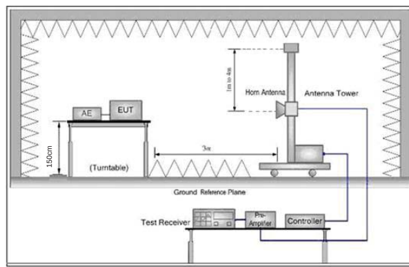
Figure 3. Above 1 GHz
