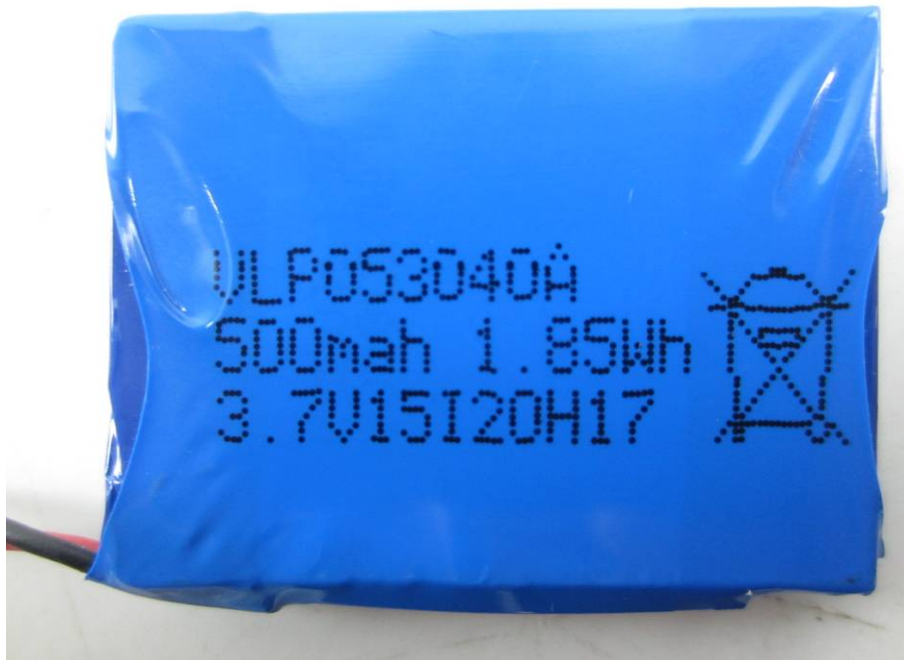
BATTERY PHOTO OF SAMPLE – 3
