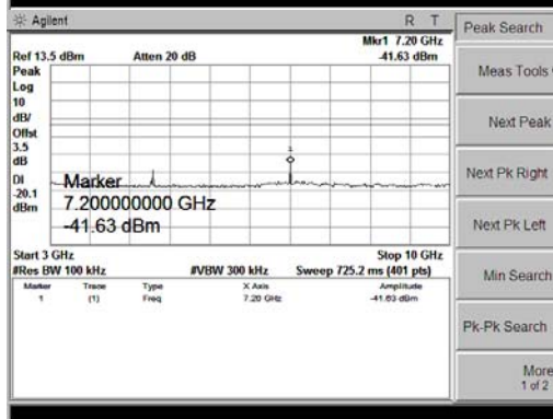
GFSK Mode, Ch0 \pi/4 -DQPSK Mode, Hopping
