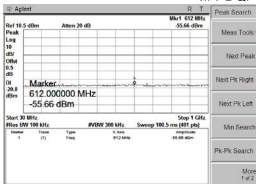
GFSK Mode, Ch0 \pi/4 -DQPSK Mode, Hopping
