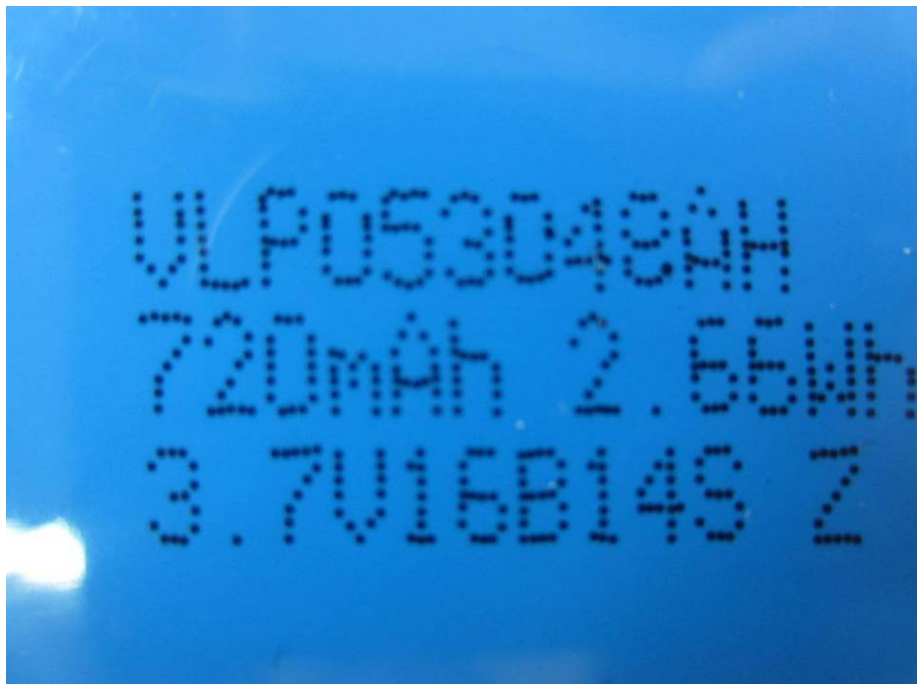
LABEL PHOTO OF BATTERY - 6
