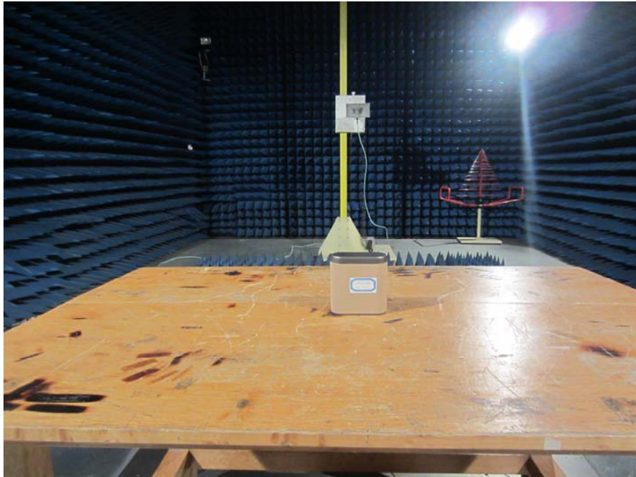
RF TEST SETUP
