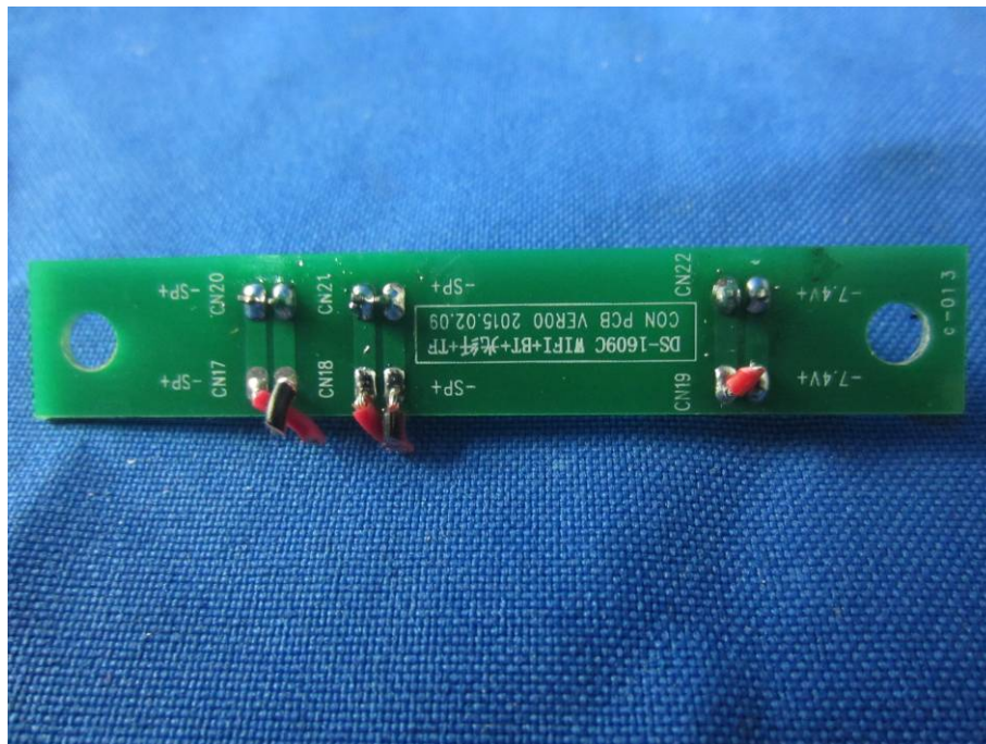
INTERNAL PHOTO OF SAMPLE – 21
