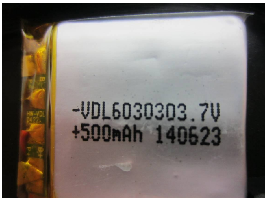
BATTERY PHOTO OF SAMPLE – 3
