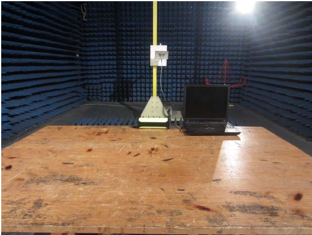
SPURIOUS EMISSION TEST SETUP
