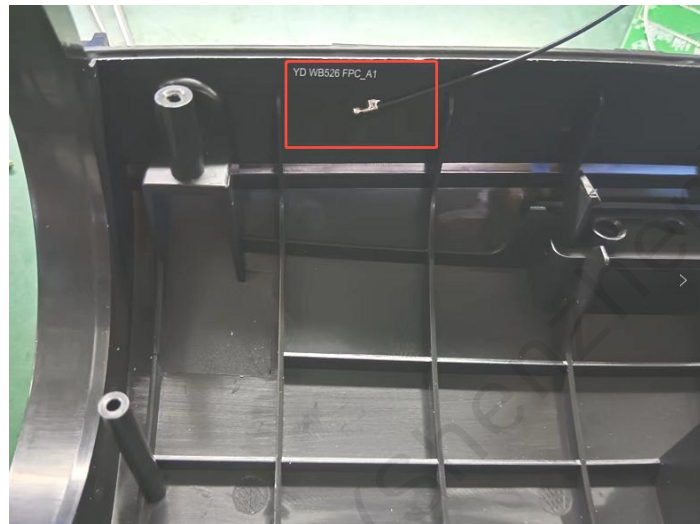
Figure 2 Antenna Position
