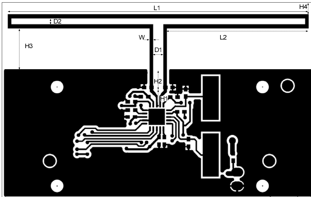
Figure 2: Antenna dimension.
