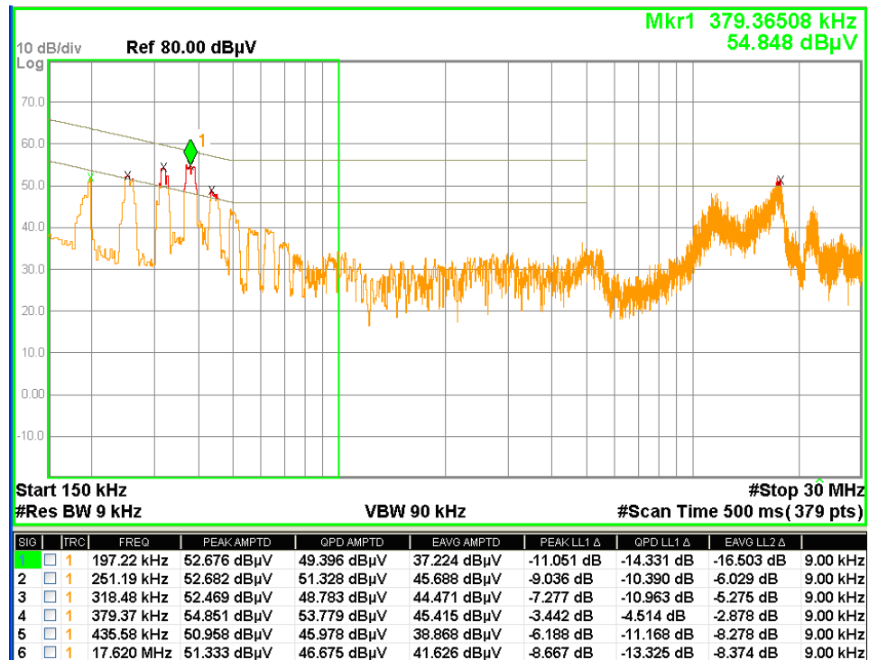
Plot # 30. AC line conducted emissions test. Line Neutral
