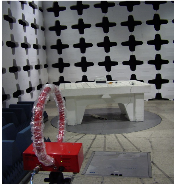
Photo 1.. Radiated emissions test setup with Loop antenna.
