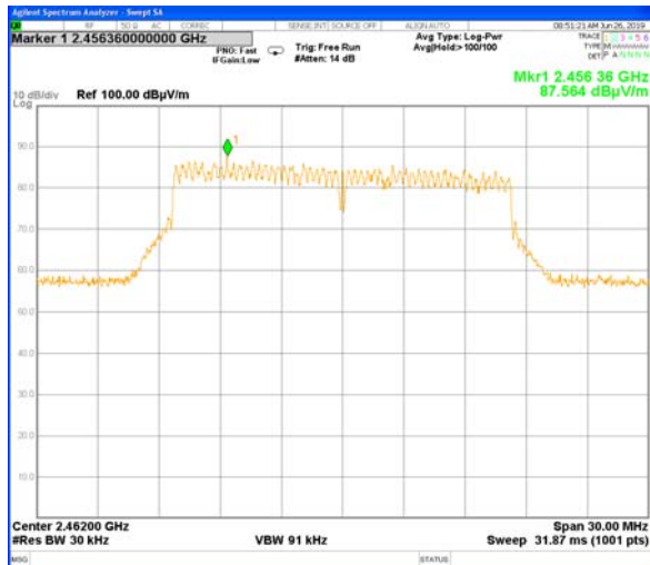
Plot # 24. Carrier frequency – 2462 MHz
