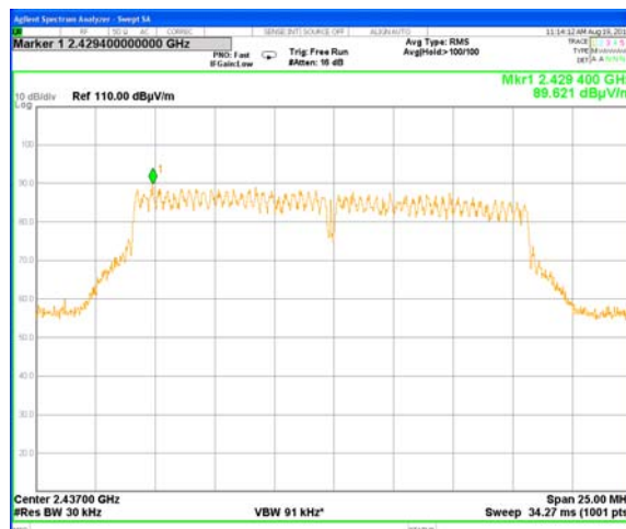
Plot # 23. Carrier frequency – 2437 MHz
