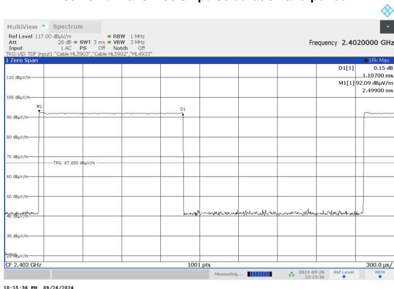
Plot 7.3.16 Transmission pulse duration and period
