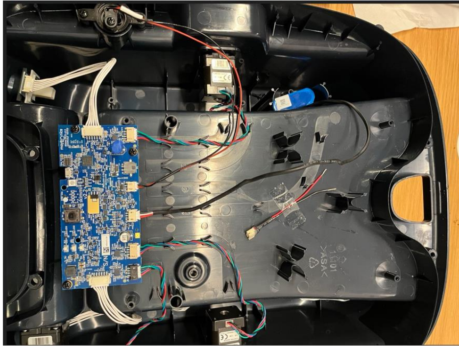
Photograph No.1 Pool surface cleaner Internal view
