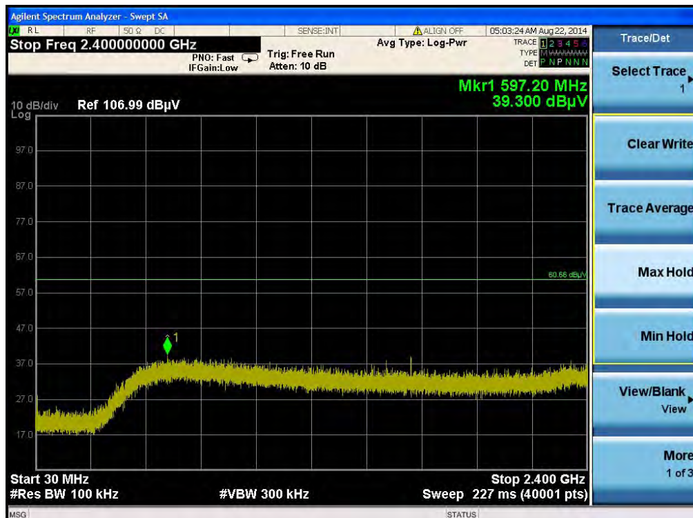
Plot on Configuration IEEE 802.11b / CH 11 / Ant. 1 / 30MHz~2400MHz (down 30dBc)
