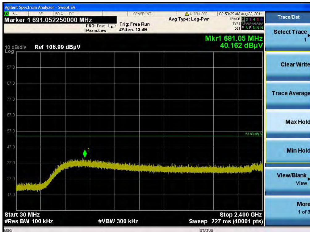
Plot on Configuration IEEE 802.11n MCS0 HT40 / CH 9 / Ant. 2 / 30MHz~2400MHz (down 30dBc)
