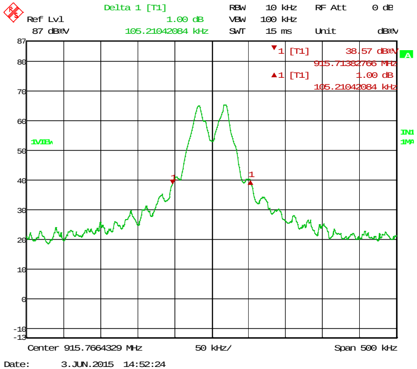
Plot 8.2 2: 20 dB bandwidth 915.767 MHz
