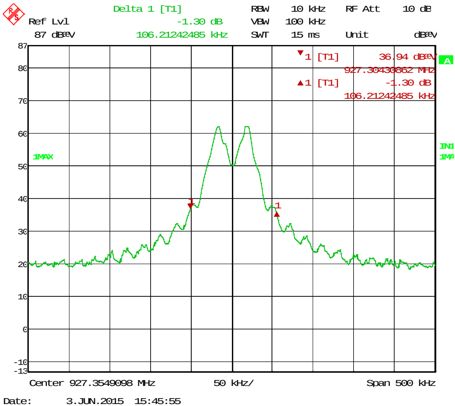
Plot 8.1-2: 20 dB bandwidth 927.356 MHz
