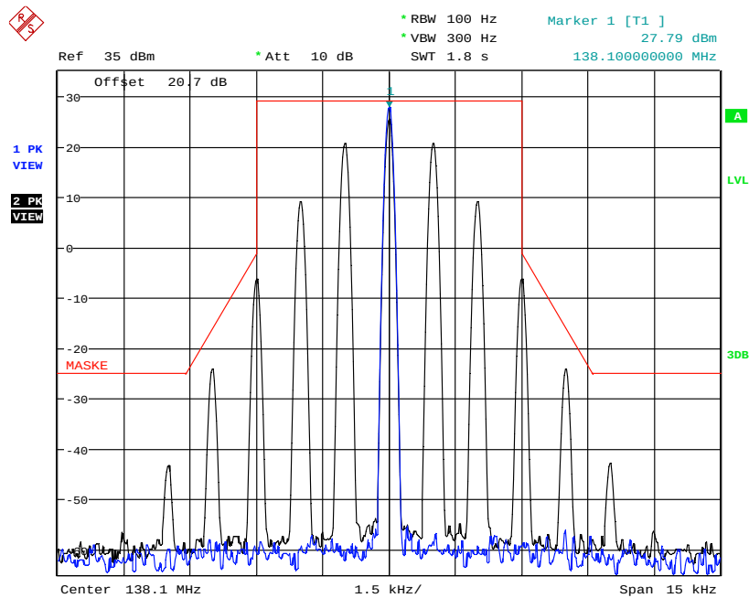
138.1MHz-Analog-6.25KHz, Signal Input_3dB above AGC
