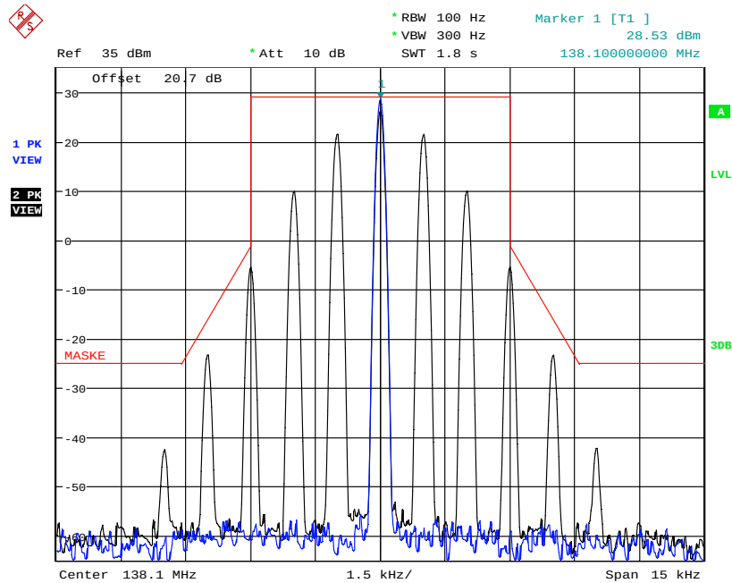
138.1MHz-Analog-6.25KHz, Signal Input_0.2dB below
