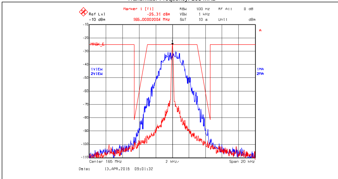
Plot 5.3.4.1.61. Emission Mask E – Input Signal, DIGITAL, 6.25kHz Ch Spacing Transmitter Frequency: 165 MHz
