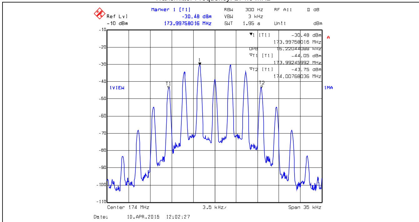
Plot 5.3.4.1.29. 99% Occupied Bandwidth – Input Signal, ANALOG, 25kHz Ch Spacing Transmitter Frequency: 174.0 MHz
