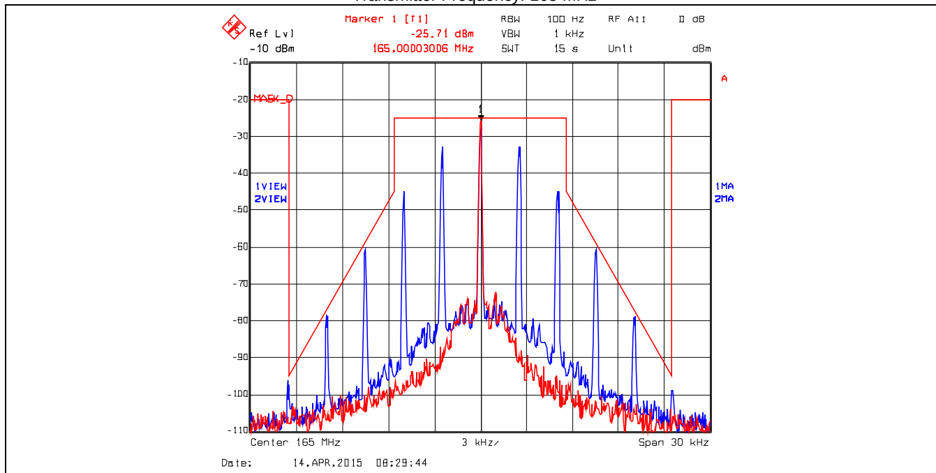
Plot 5.3.4.1.73. Emission Mask D, Input Signal, ANALOG, 12.5kHz Ch Spacing Transmitter Frequency: 165 MHz
