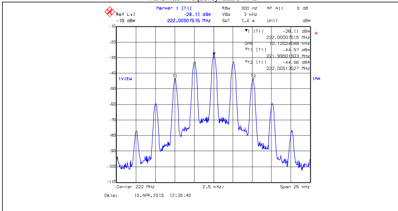
Plot 5.3.4.1.53. 99% Occupied Bandwidth – Input Signal, ANALOG, 12.5kHz Ch Spacing Transmitter Frequency: 222.0 MHz
