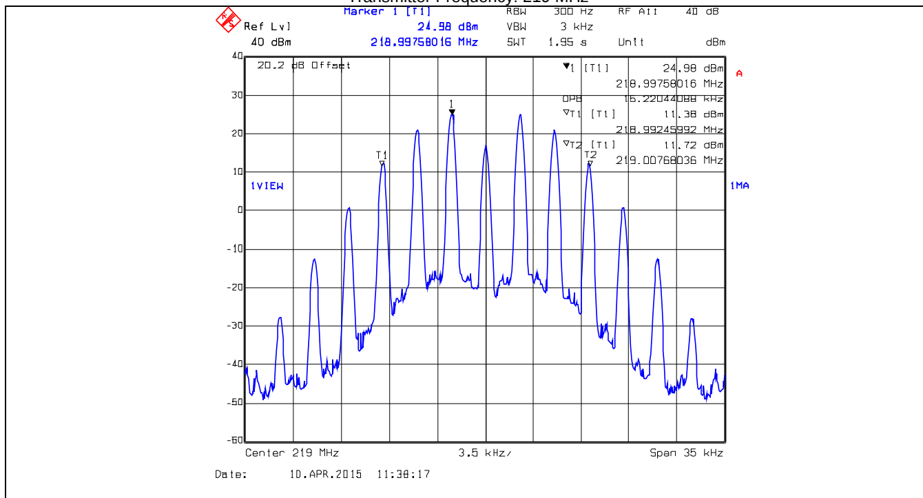
Plot 5.3.4.1.58. 99% Occupied Bandwidth – Output Signal, ANALOG, 25kHz Ch Spacing Transmitter Frequency: 219 MHz
