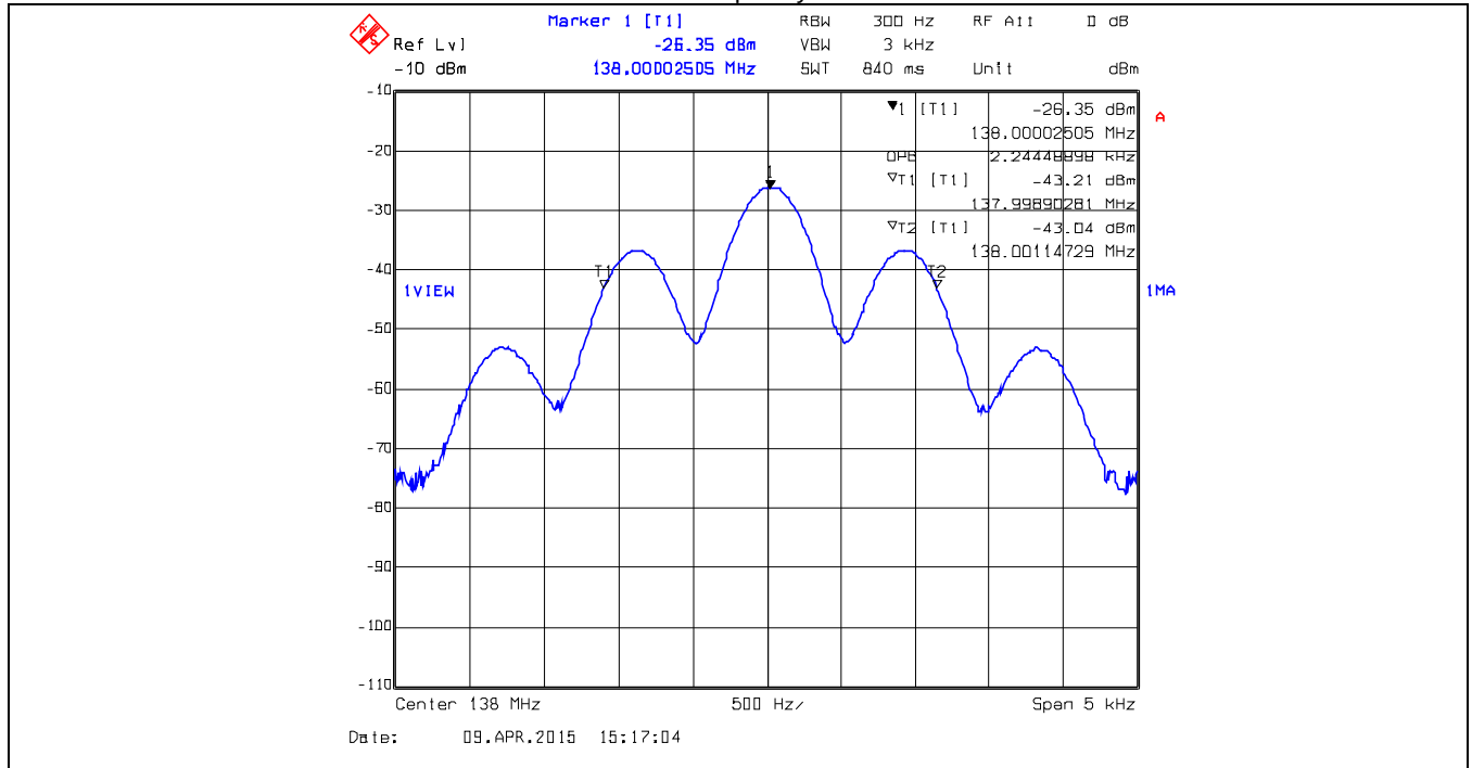
Plot 5.3.4.1.13. 99% Occupied Bandwidth – Input Signal, ANALOG, 6.25kHz Ch Spacing Transmitter Frequency: 138 MHz
