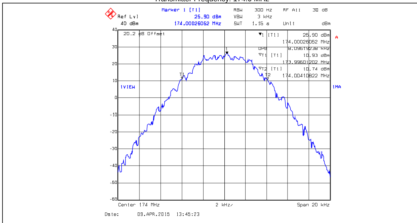
Plot 5.3.4.1.12. 99% Occupied Bandwidth – Output Signal, DIGITAL, 12.5kHz Ch Spacing Transmitter Frequency: 174.0 MHz
