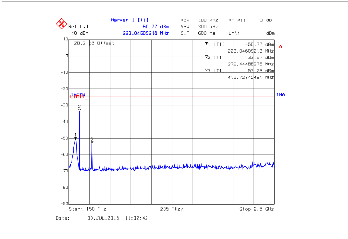
Plot 5.4.4.14. Conducted Transmitter Spurious Emissions for Multi Channel Inputs (3 Adjacent Channels) 138, 137.99375 & 138.00625 MHz, 150 MHz - 2.5 GHz
