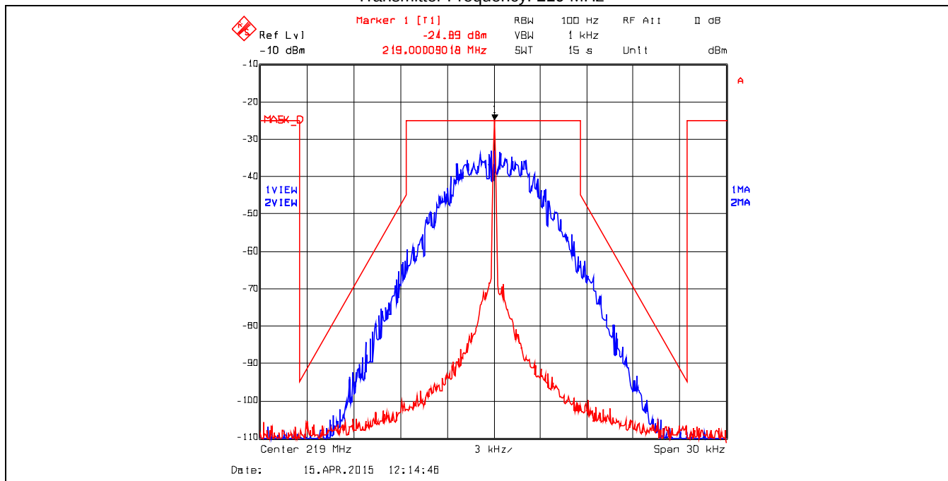
Plot 5.3.4.1.67. Emission Mask D, Input Signal, DIGITAL, 12.5kHz Ch Spacing Transmitter Frequency: 219 MHz
