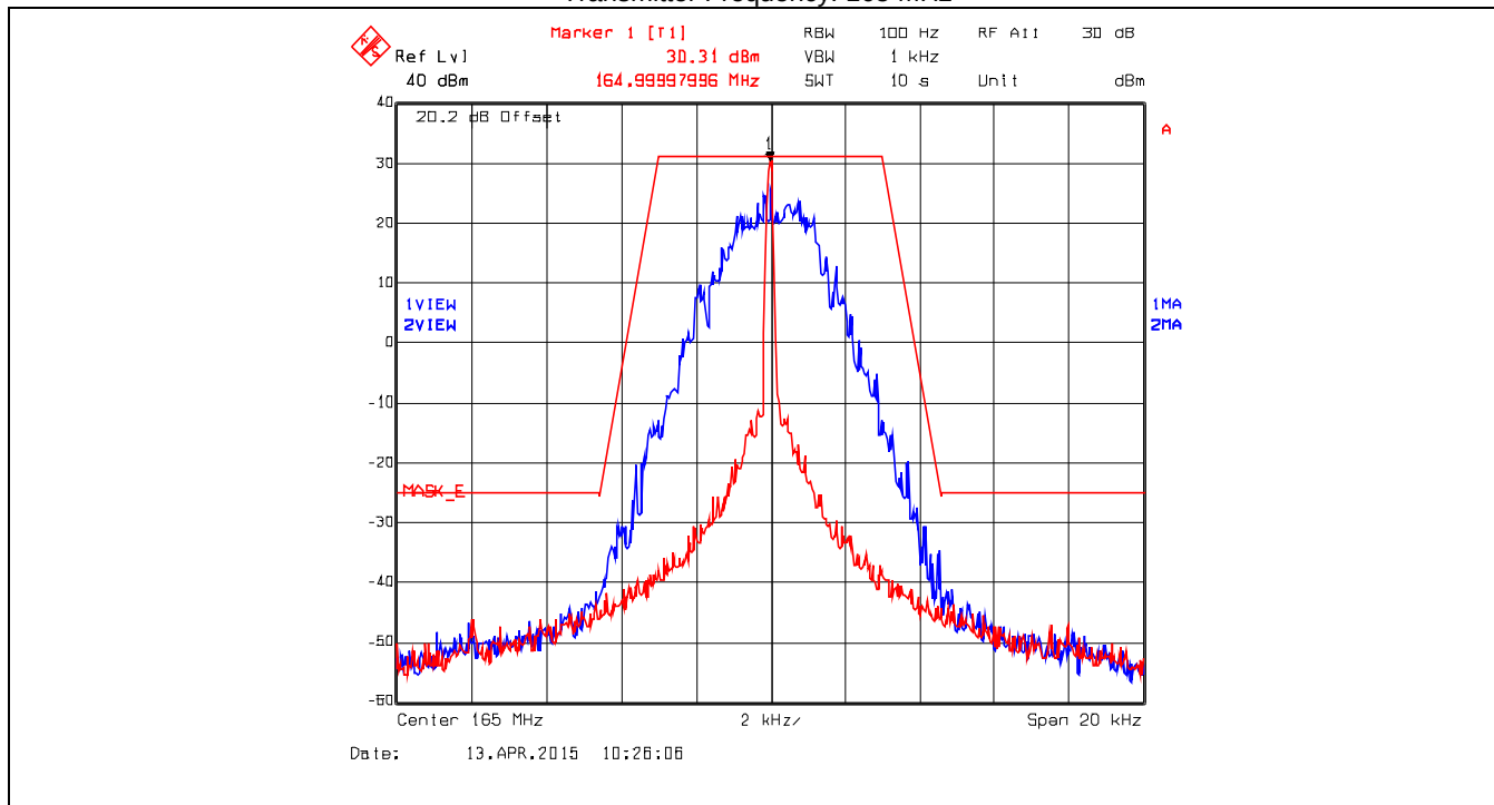
Plot 5.3.4.1.62. Emission Mask E – Output Signal, DIGITAL, 6.25kHz Ch Spacing Transmitter Frequency: 165 MHz
