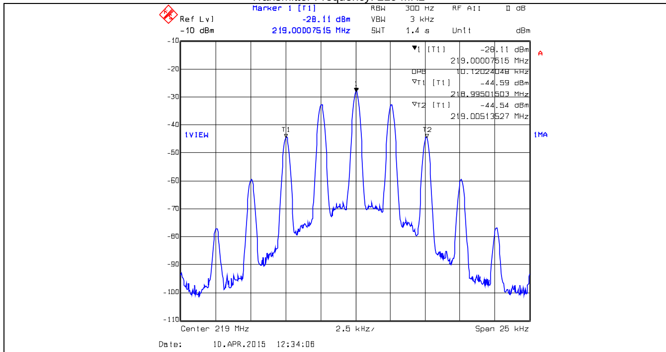
Plot 5.3.4.1.51. 99% Occupied Bandwidth – Input Signal, ANALOG, 12.5kHz Ch Spacing Transmitter Frequency: 219 MHz
