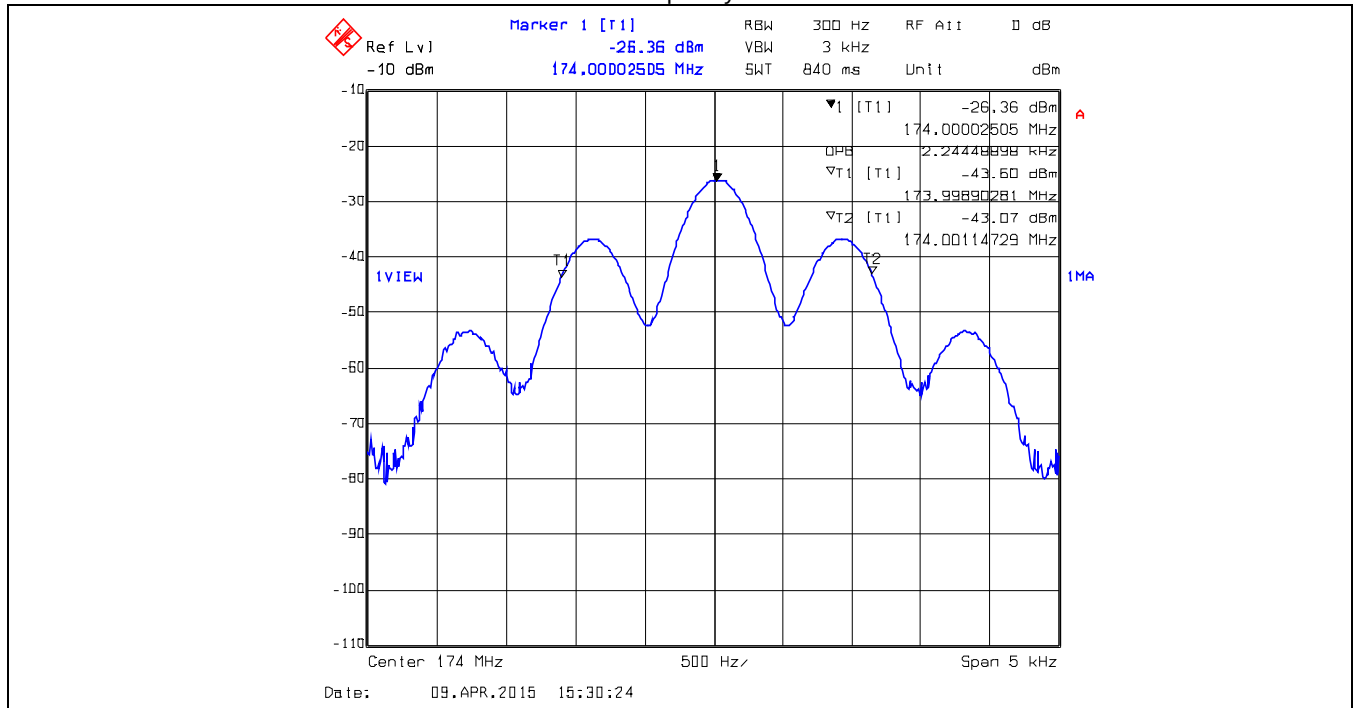
Plot 5.3.4.1.17. 99% Occupied Bandwidth – Input Signal, ANALOG, 6.25kHz Ch Spacing Transmitter Frequency: 174.0 MHz
