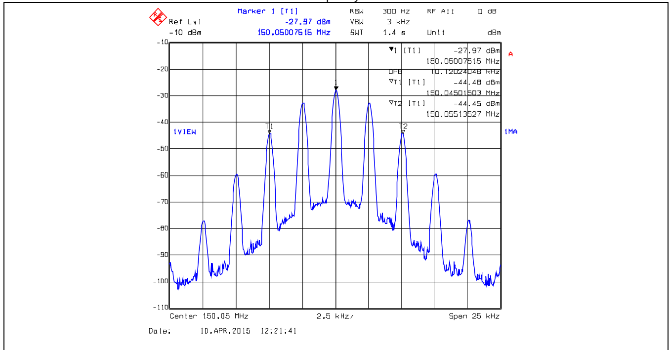
Plot 5.3.4.1.22. 99% Occupied Bandwidth – Output Signal, ANALOG, 12.5kHz Ch Spacing Transmitter Frequency: 150.05 MHz
