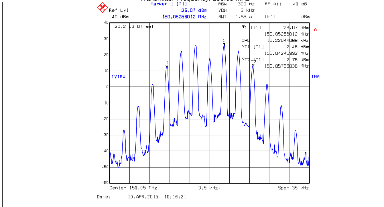
Plot 5.3.4.1.28. 99% Occupied Bandwidth – Output Signal, ANALOG, 25kHz Ch Spacing Transmitter Frequency: 150.05 MHz
