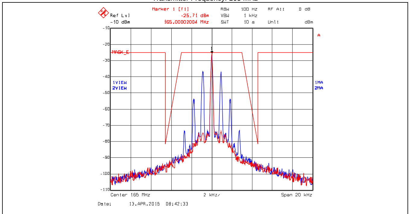
Plot 5.3.4.1.69. Emission Mask E – Input Signal, ANALOG, 6.25kHz Ch Spacing Transmitter Frequency: 165 MHz
