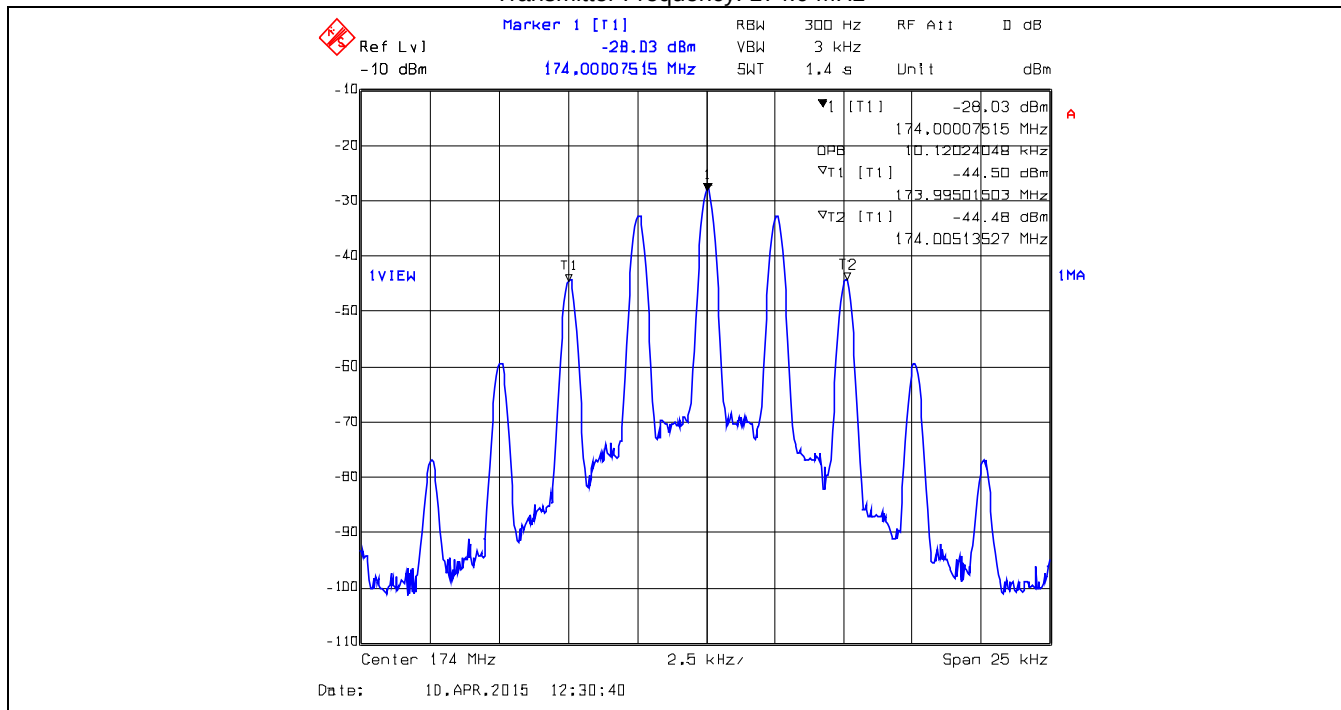
Plot 5.3.4.1.23. 99% Occupied Bandwidth – Input Signal, ANALOG, 12.5kHz Ch Spacing Transmitter Frequency: 174.0 MHz
