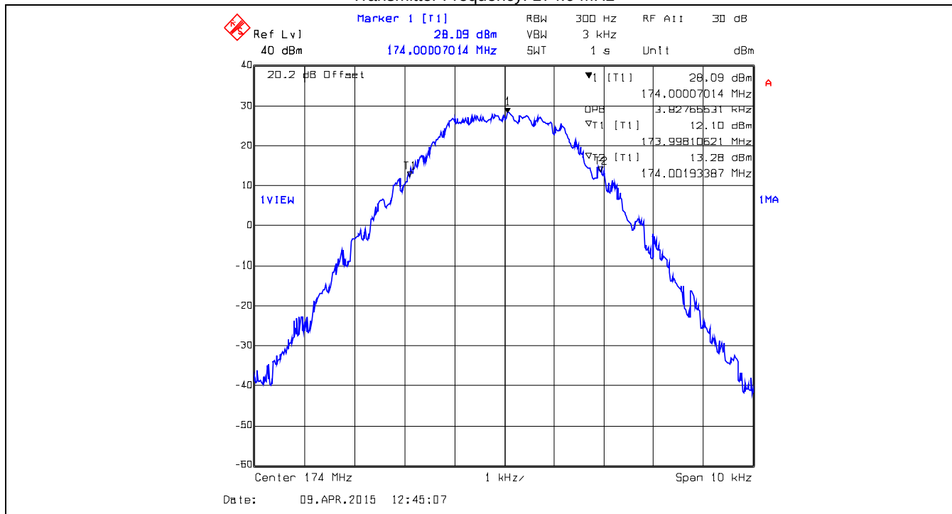
Plot 5.3.4.1.6. 99% Occupied Bandwidth – Output Signal, DIGITAL, 6.25kHz Ch Spacing Transmitter Frequency: 174.0 MHz
