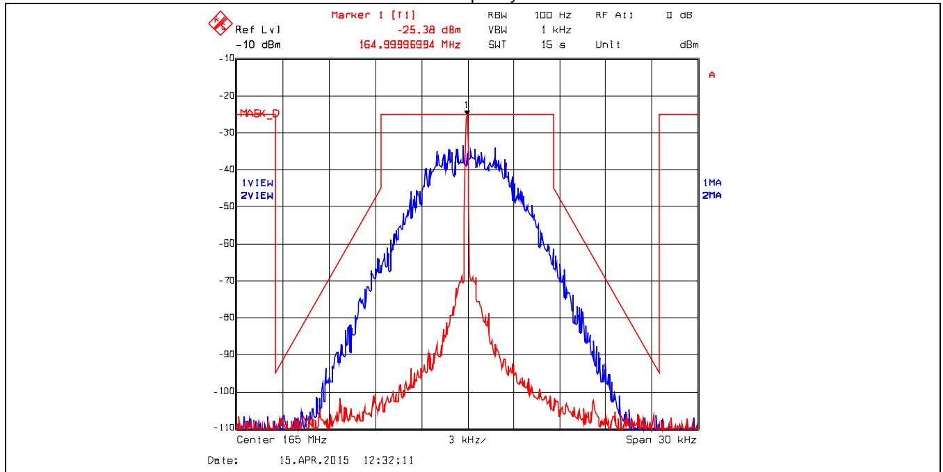
Plot 5.3.4.1.66. Emission Mask D, Output Signal, DIGITAL, 12.5kHz Ch Spacing Transmitter Frequency: 165 MHz
