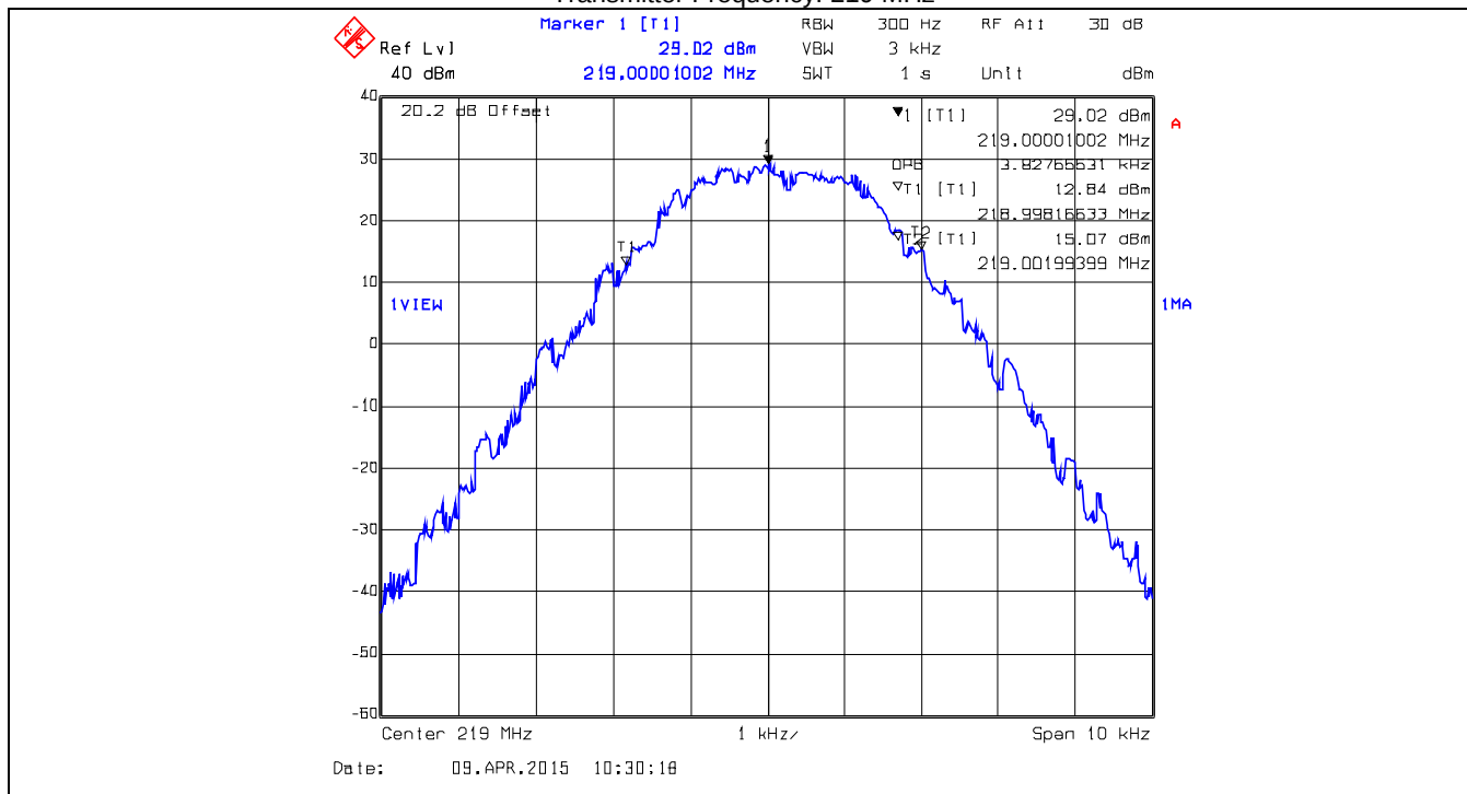
Plot 5.3.4.1.34. 99% Occupied Bandwidth – Output Signal, DIGITAL, 6.25kHz Ch Spacing Transmitter Frequency: 219 MHz
