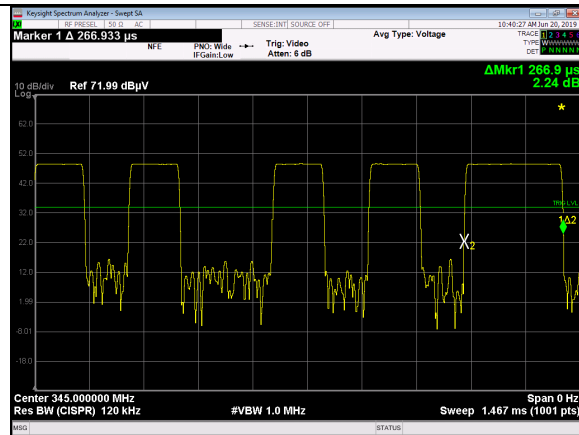
Figure 3 Large Pulse Duration (RED)
