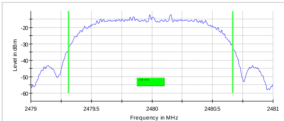
20 dB Bandwidth
