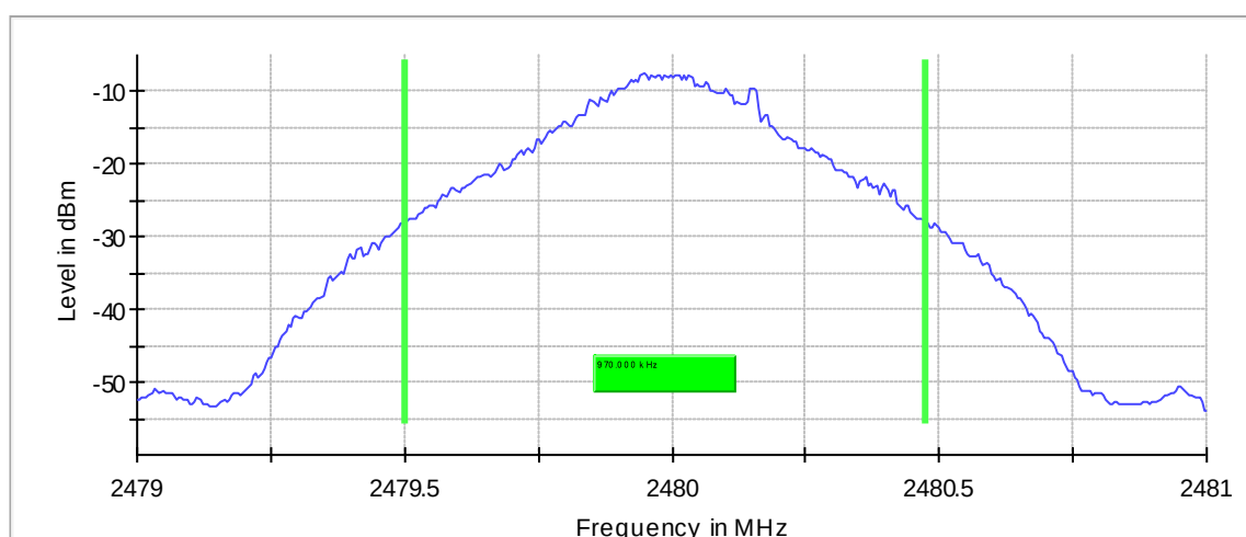
20 dB Bandwidth
