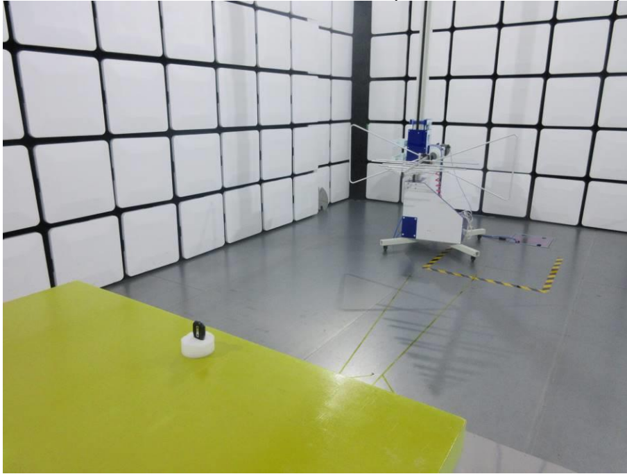
RADIATED RF MEASUREMENT SETUP (30MHz ~ 1 GHz - X axis)
