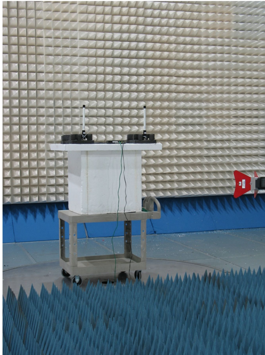
Radiated Spurious Emissions - BS2400XL3 Antenna
