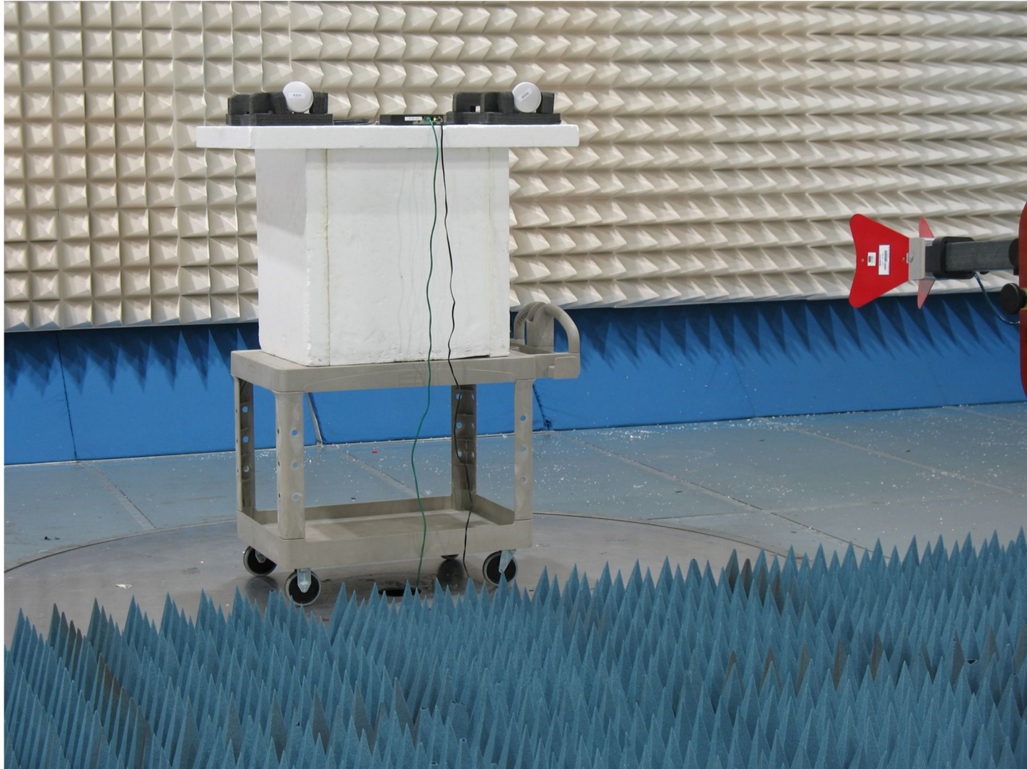
Radiated Spurious Emissions - MC2400PTMSMA Antenna
