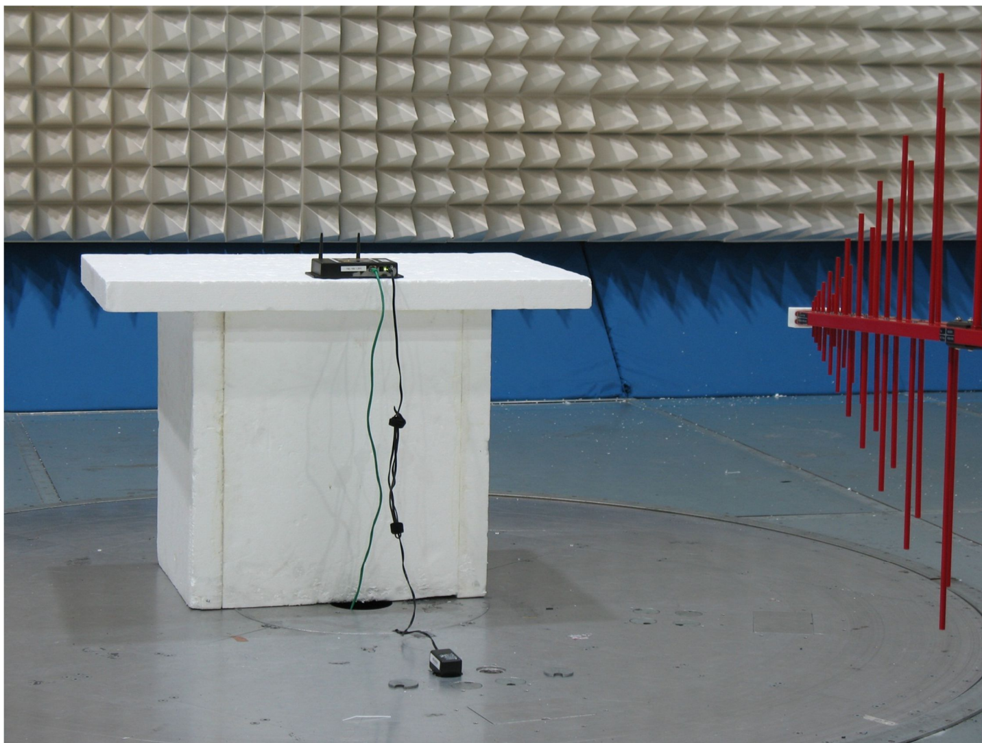
Radiated Spurious Emissions – HG2402RD-RSF Antenna
