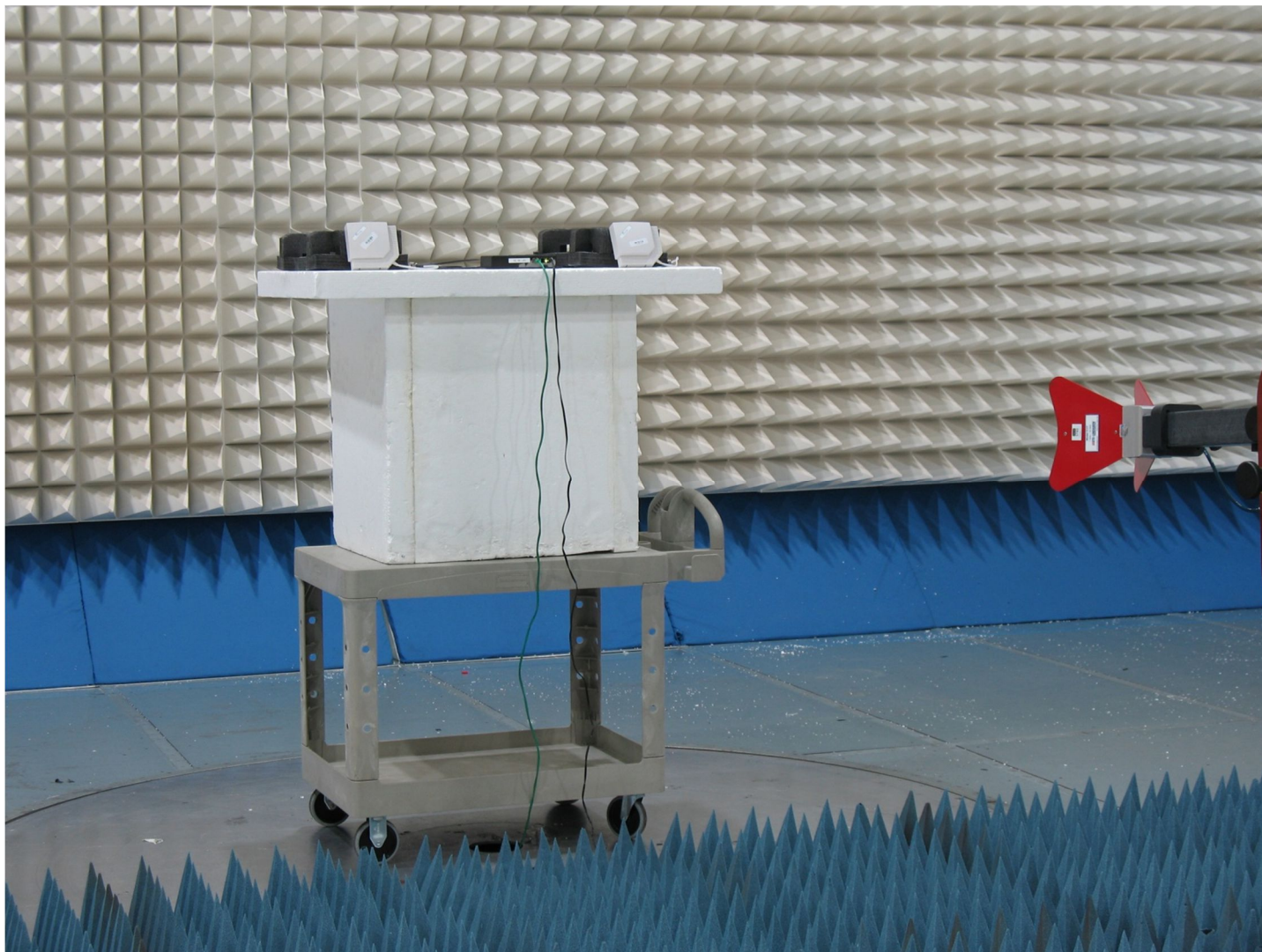
Radiated Spurious Emissions - MP24008XFPTNF Antenna
