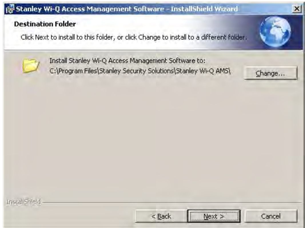
Figure 34 Destination Folder
