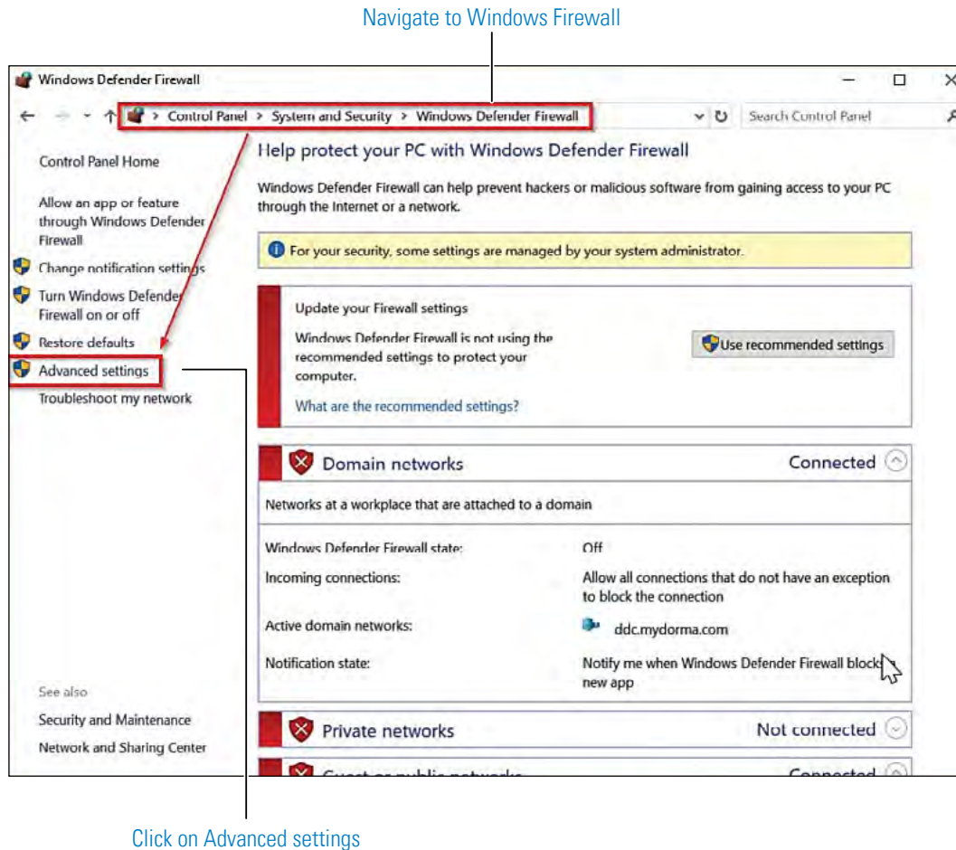
Figure 12 Windows Firewall
