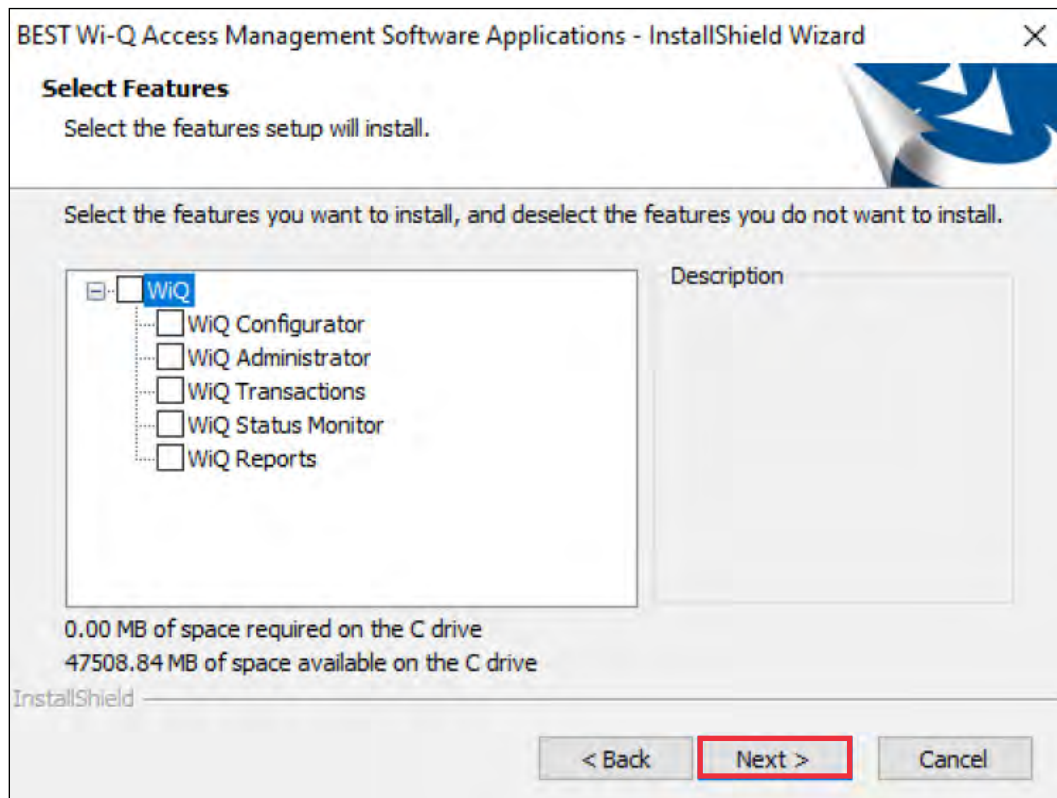
Figure 37 Custom Setup
