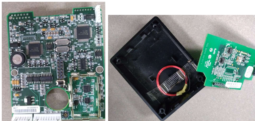
45HQ-PKP configuration internals
