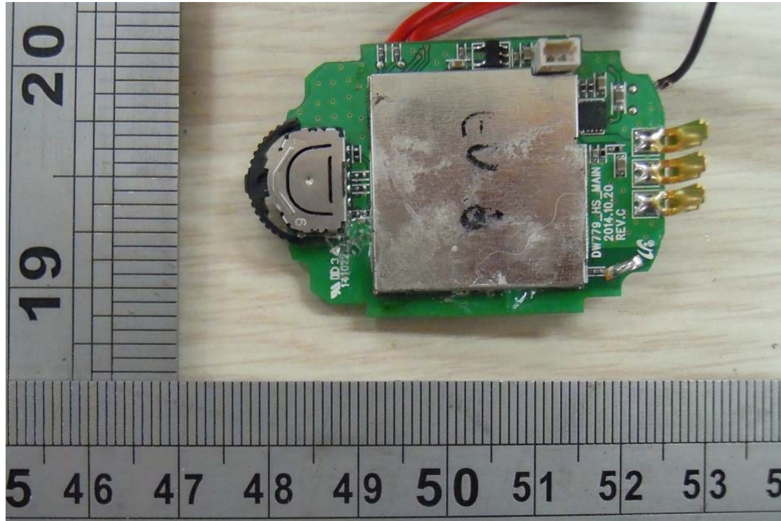
[Main board Front]
