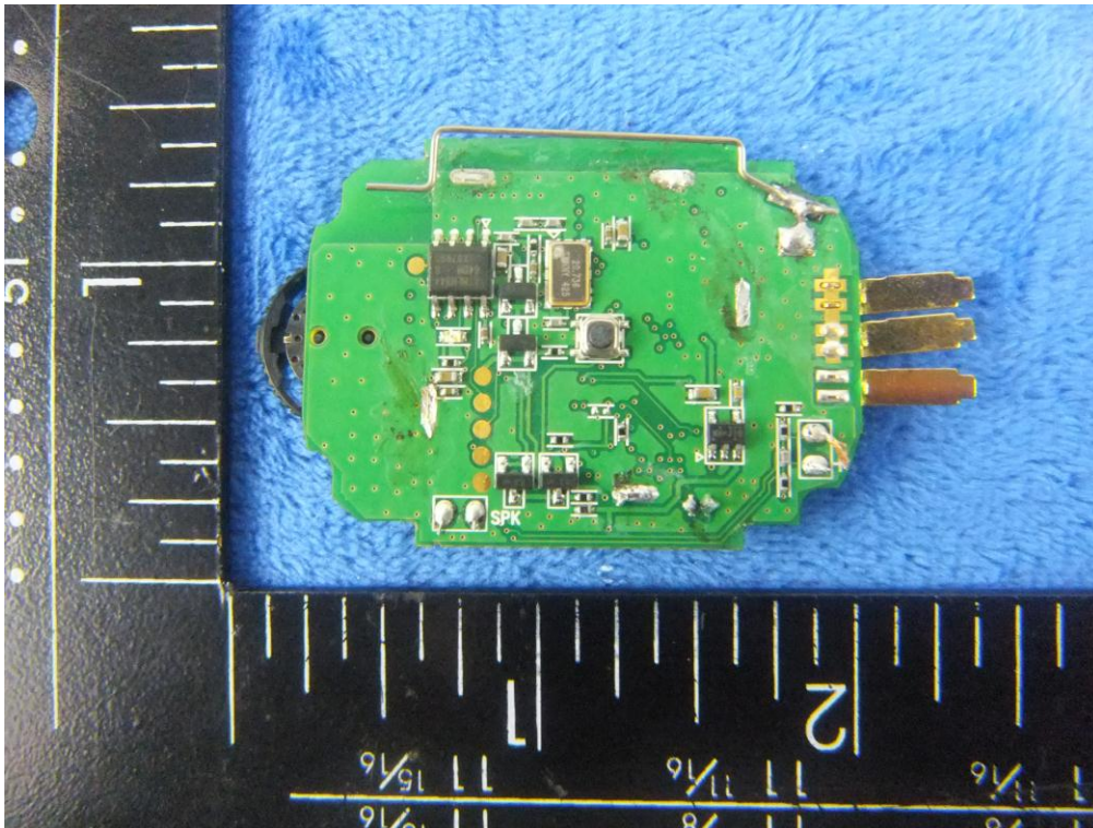
EUT – Mainboard Front View PP
