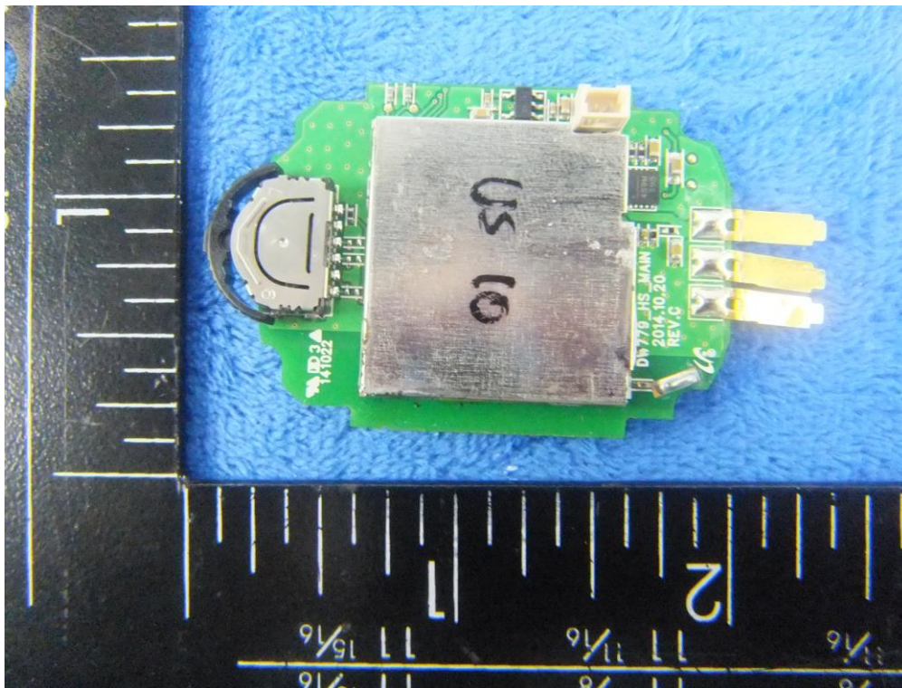
EUT – Mainboard Rear View PP
