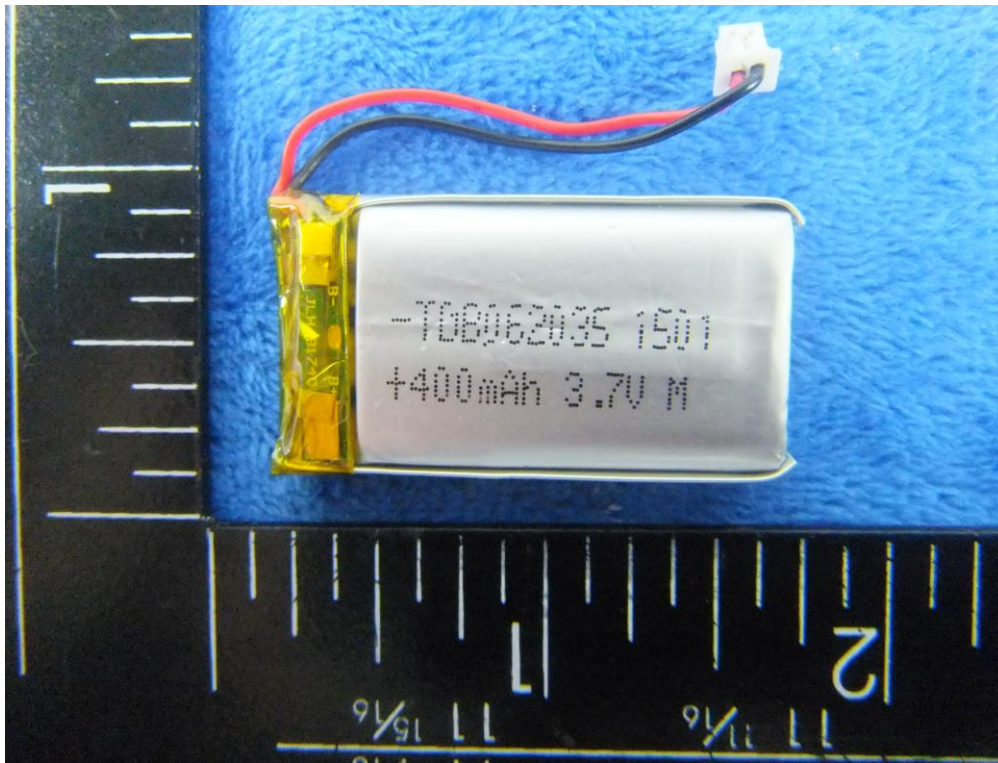
Battery – Front View PP
