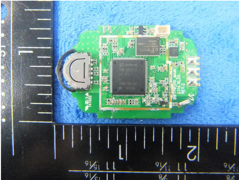
EUT – Mainboard Without Sheilding Rear View PP
