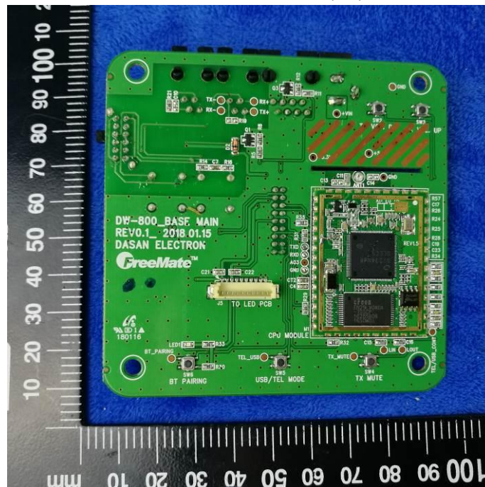
Mainboard - Rear View(FP)
