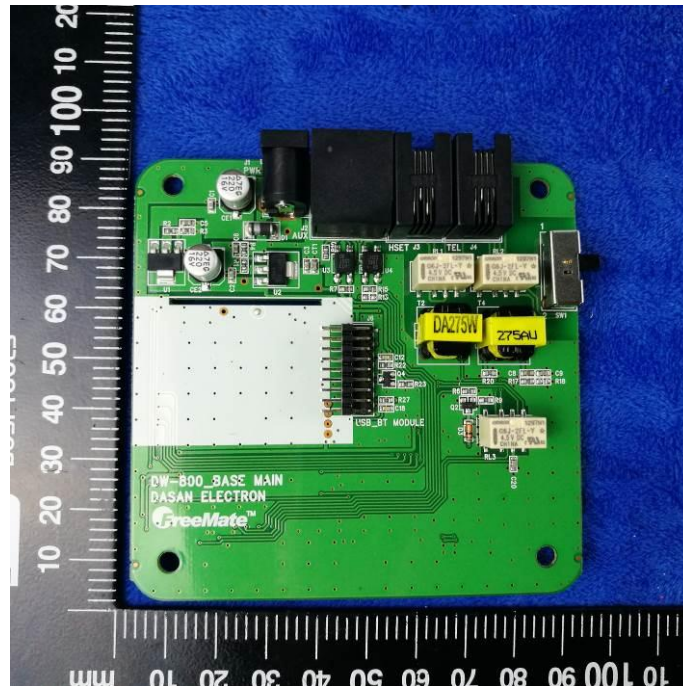
Mainboard - Front View(FP)
