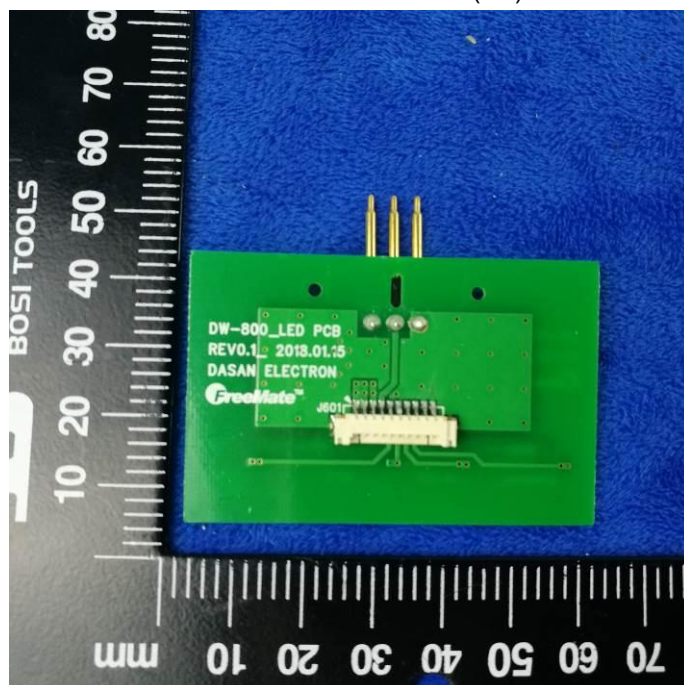
Small board - Rear View (FP)
