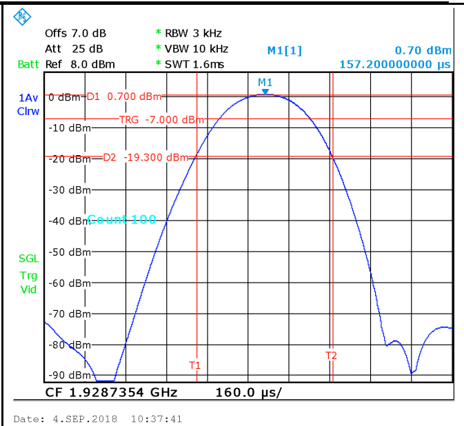
GFSK - High Channel 2
