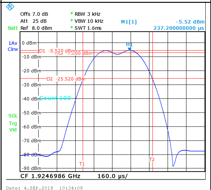
GFSK - Middle Channel 2
