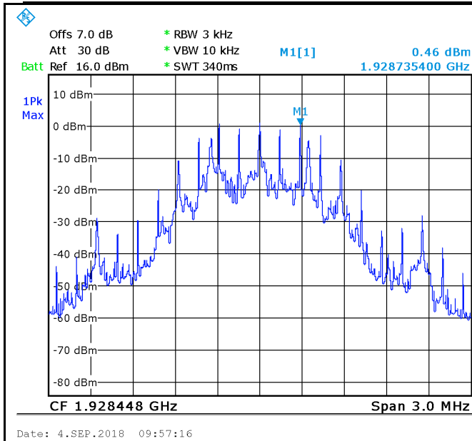
GFSK - High Channel 1
