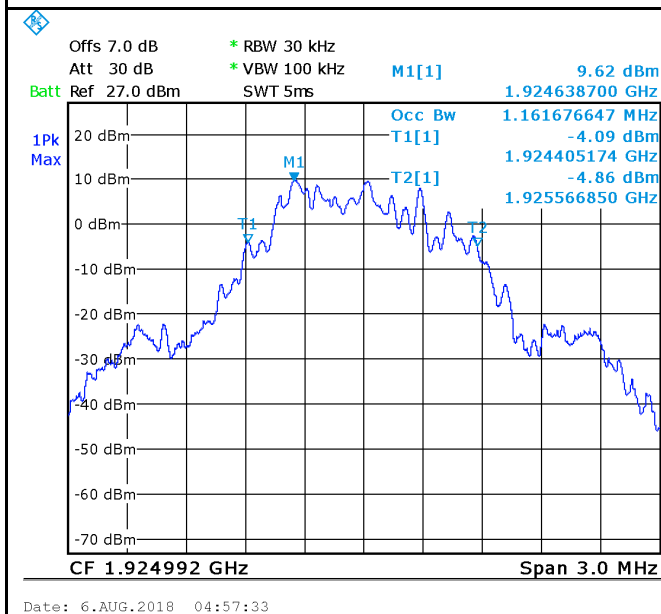
GFSK - Middle Channel 99%
