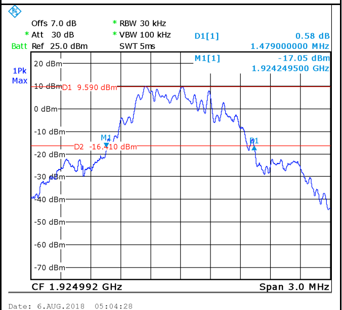
GFSK - Middle Channel 26dB
