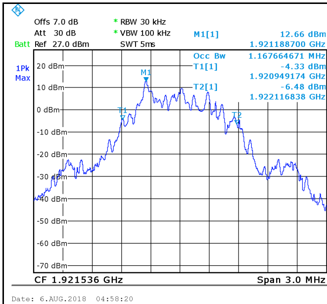
GFSK - Low Channel 99%
