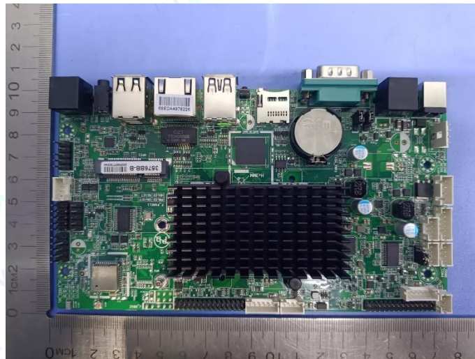
Photo 14 Appearance of PCB
