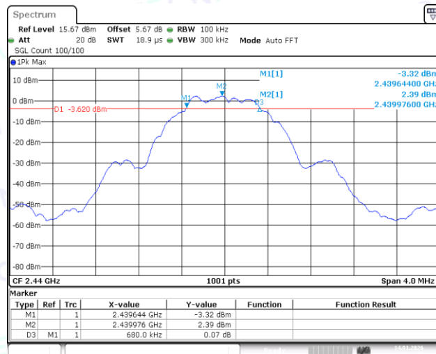
BLE_1M-Ant1-2440-PASS
