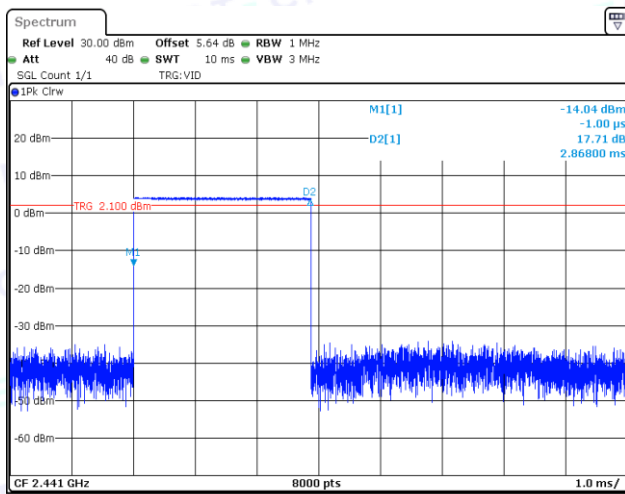
DH3-Ant1-Hop-PASS
