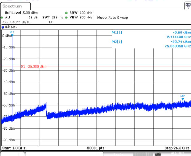
2DH5-Ant1-2441-0~Reference-PASS
