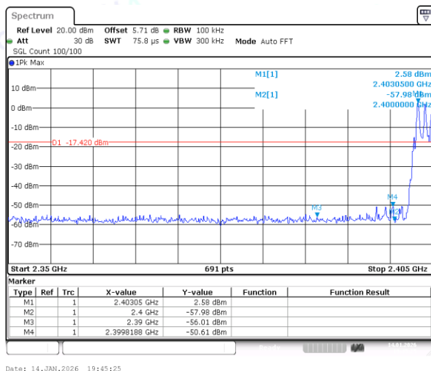
DH5-Ant1-Hop_2402-PASS
