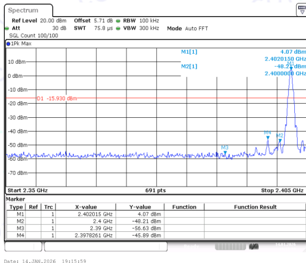
DH5-Ant1-2402-PASS
