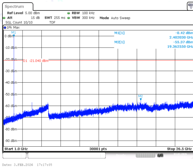
DH5-Ant1-2402-1000~26500-PASS
