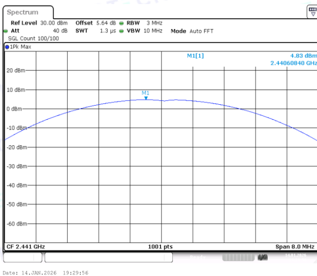
2DH5-Ant1-2441-PASS
