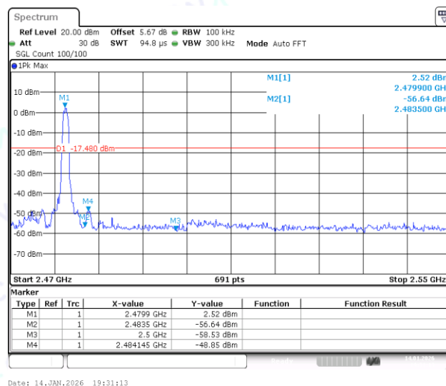
2DH5-Ant1-2480-PASS
