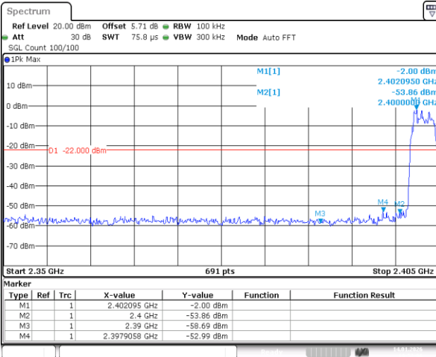
2DH5-Ant1-Hop_2402-PASS
