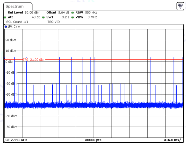
DH3-Ant1-Hop-PASS
