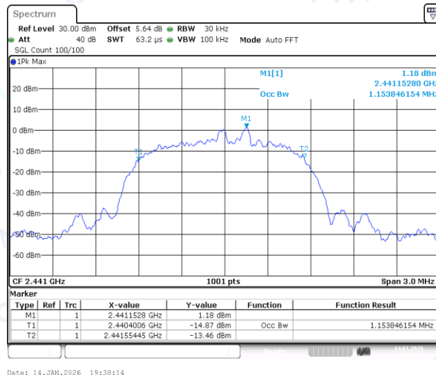
3DH5-Ant1-2441
