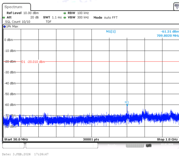
DH5-Ant1-2441-30~1000-PASS
