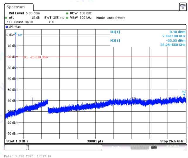
DH5-Ant1-2441-1000~26500-PASS
