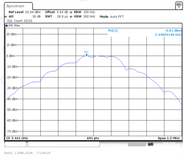
DH5-Ant1-2441-0~Reference-PASS
