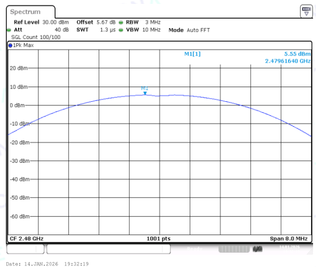
2DH5-Ant1-2480-PASS
