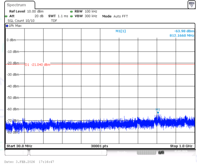
DH5-Ant1-2402-30~1000-PASS
