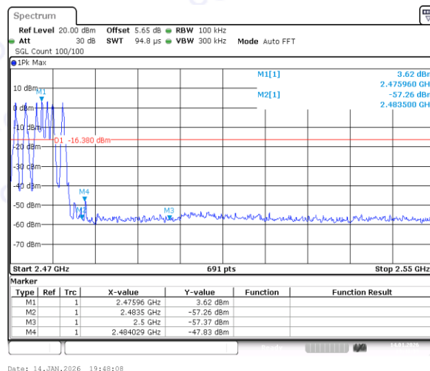
DH5-Ant1-Hop_2480-PASS
