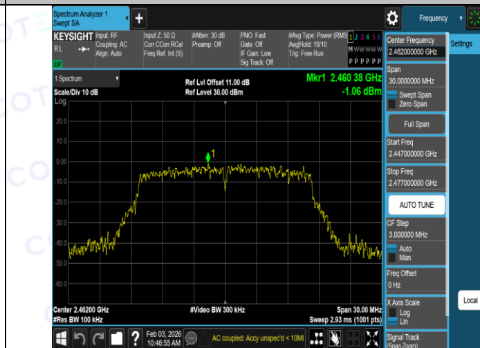
11G-Ant1-2462-0~Reference-PASS
