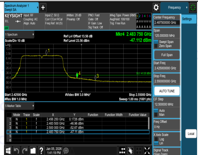
11N40SISO-Ant1-2452-PASS
