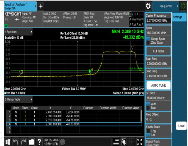
11N40SISO-Ant1-2422-PASS
