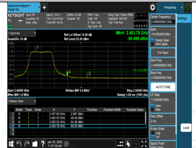
11N20SISO-Ant1-2462-PASS
