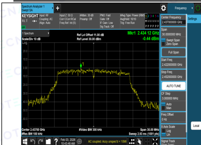
11G-Ant1-2437-0~Reference-PASS
