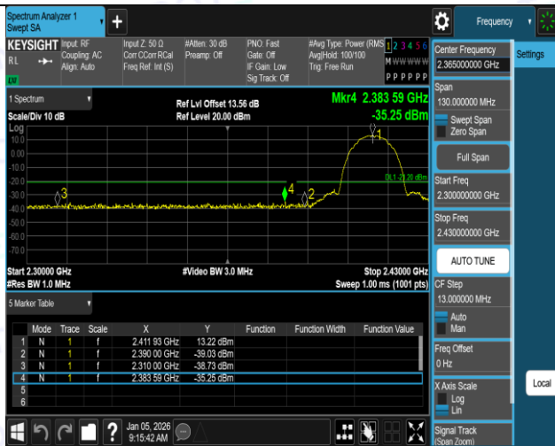
11B-Ant1-2412-PASS
