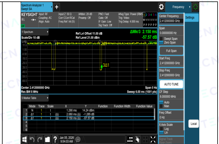
NTNV-11G-Ant1-2412
