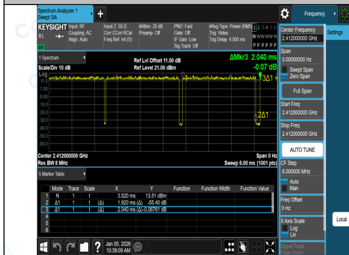
NTNV-11N20SISO-Ant1-2412
