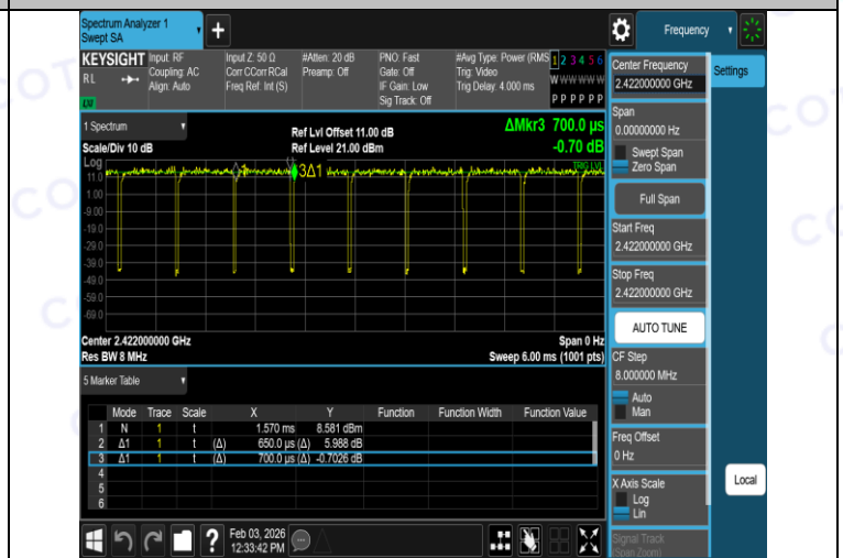
NTNV-11N40SISO-Ant1-2422
