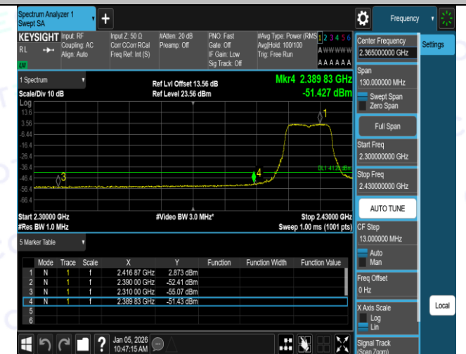
11N20SISO-Ant1-2412-PASS
