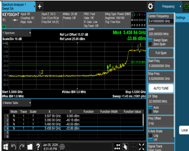
11AC40SISO-Ant1-5510-PASS
