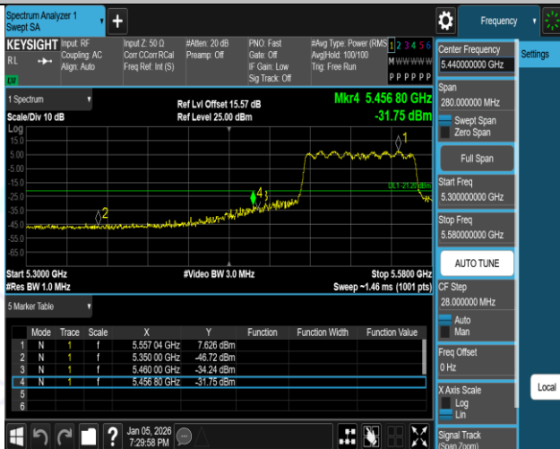
11AC80ISO-Ant1-5530-PASS
