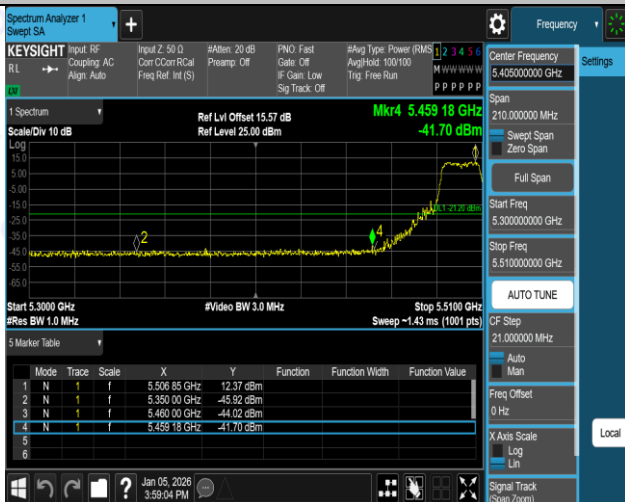
11AC20SISO-Ant1-5500-PASS
