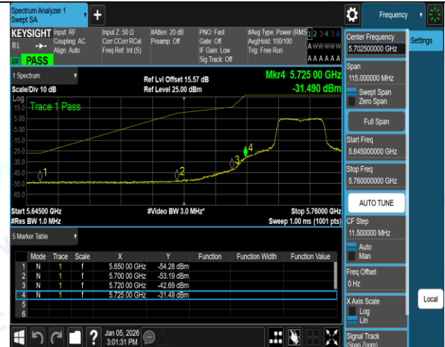
11A-Ant1-5745-PASS
