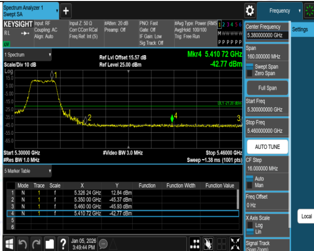
11AC20SISO-Ant1-5320-PASS
