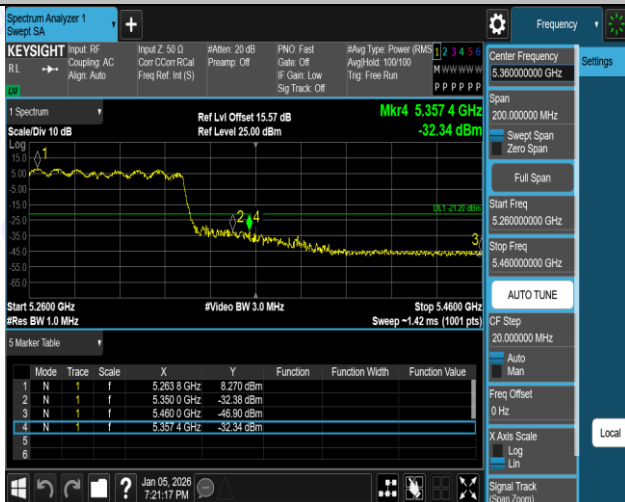
11AC80ISO-Ant1-5290-PASS
