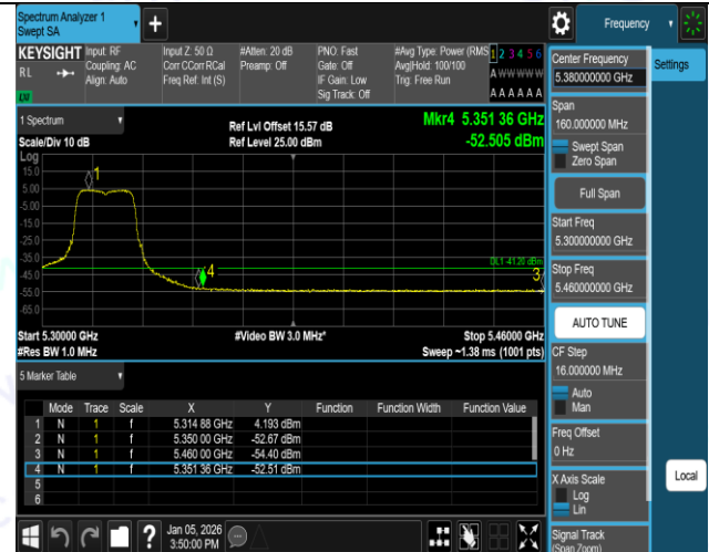
11AC20SISO-Ant1-5320-PASS
