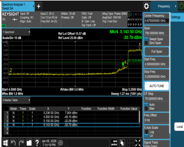
11AC80ISO-Ant1-5210-PASS
