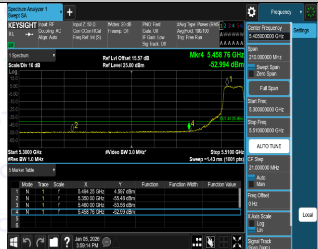
11AC20SISO-Ant1-5500-PASS
