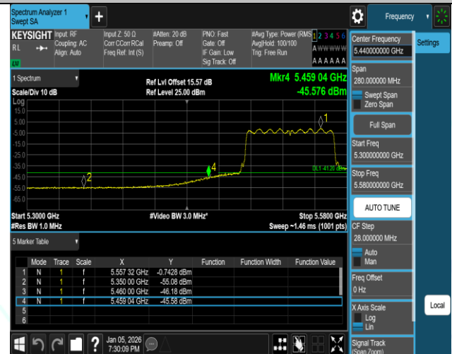
11AC80ISO-Ant1-5530-PASS
