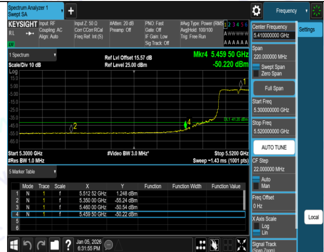
11AC40SISO-Ant1-5510-PASS
