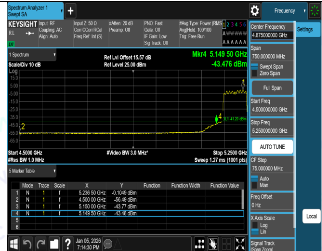
11AC80ISO-Ant1-5210-PASS
