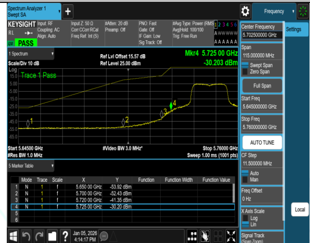
11AC20SISO-Ant1-5745-PASS
