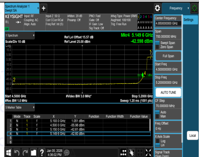
11AC40SISO-Ant1-5190-PASS
