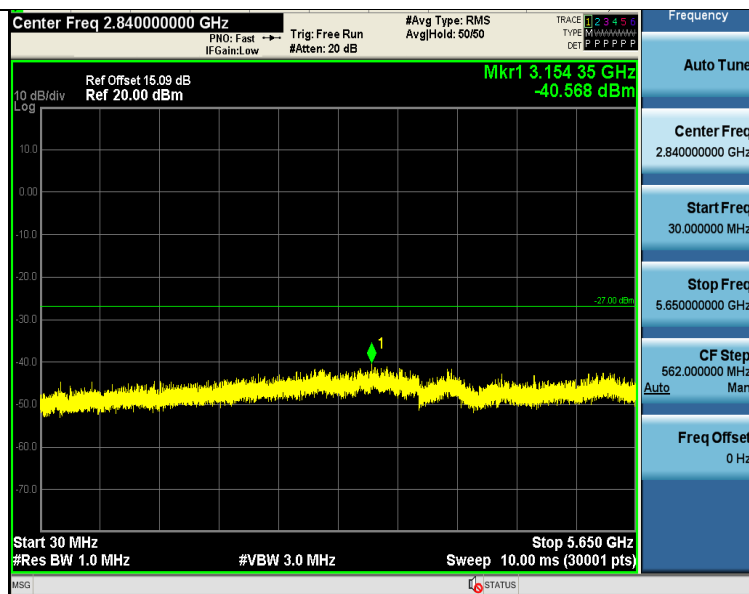
11A-Ant1-5825-30~5650-PASS
