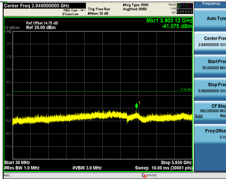
11A-Ant1-5745-30~5650-PASS
