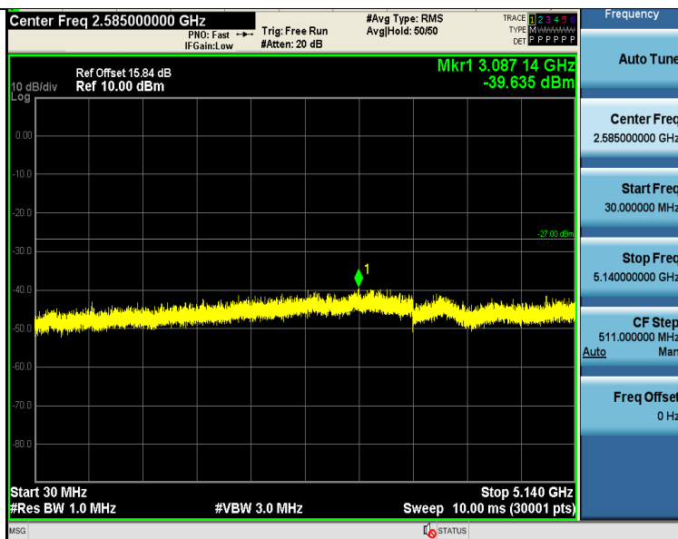
11AC20SISO-Ant1-5200-30~5140-PASS
