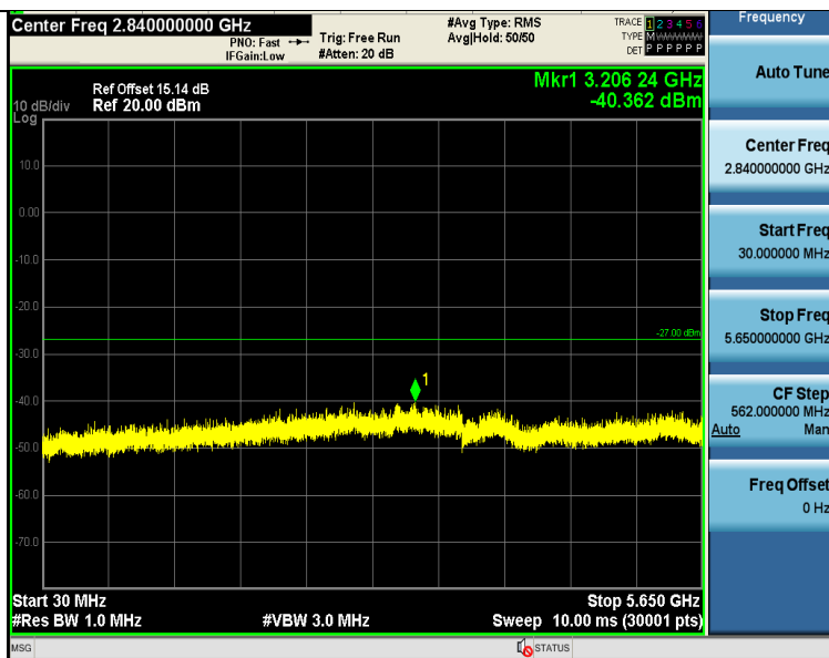
11N40SISO-Ant1-5795-30~5650-PASS
