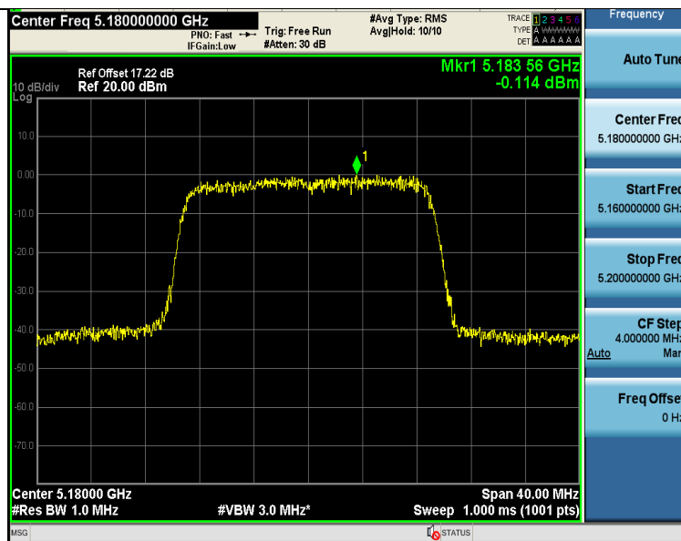
11AC20SISO-Ant1-5180-PASS
