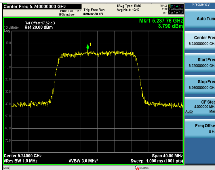
11N20SISO-Ant1-5240-PASS
