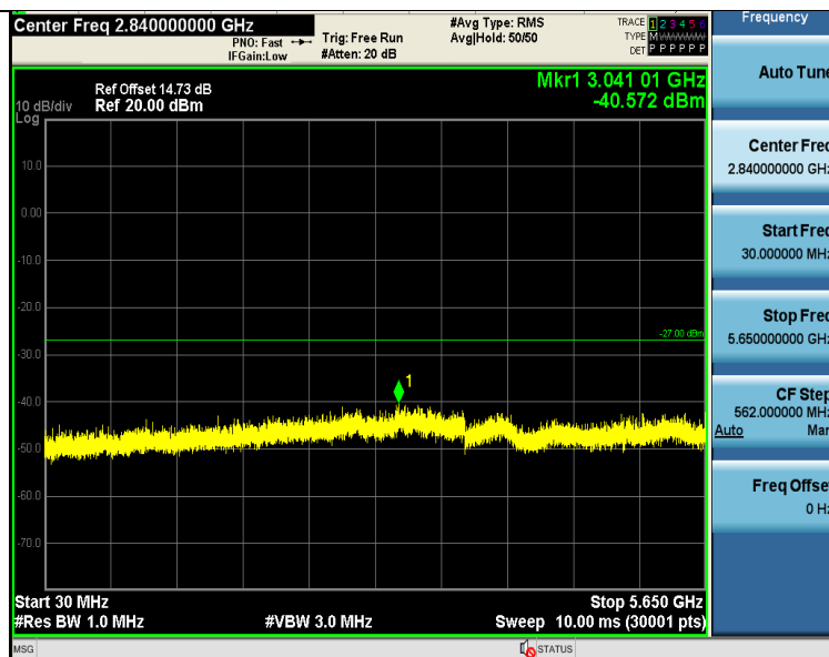
11AC40SISO-Ant1-5755-30~5650-PASS
