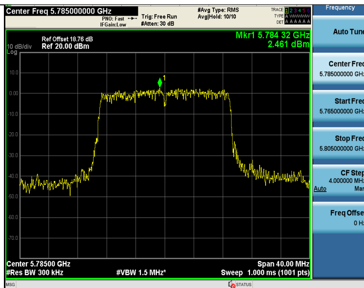
11AC20SISO-Ant1-5785-PASS
