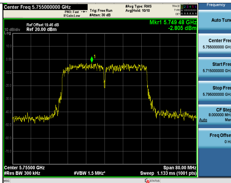
11AC40SISO-Ant1-5755-PASS
