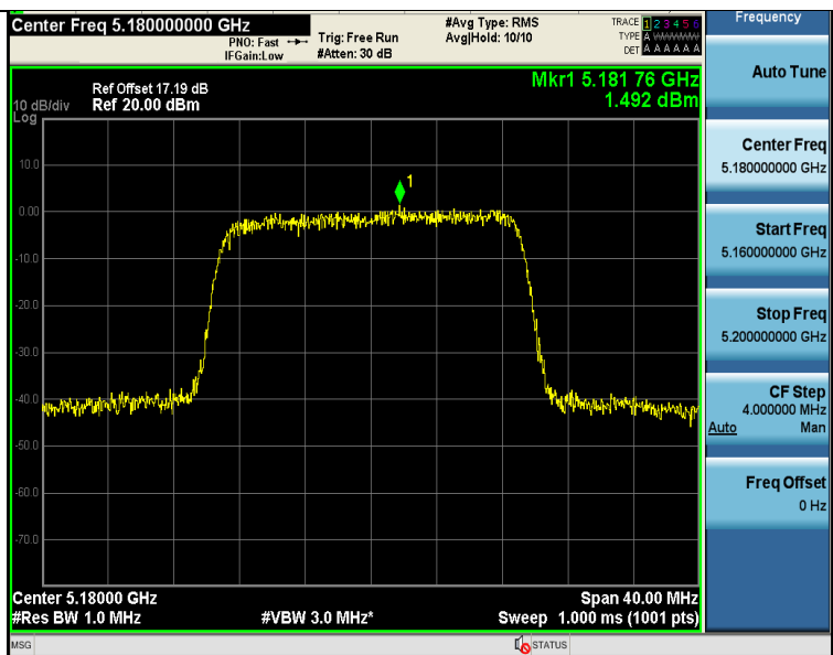
11N20SISO-Ant1-5180-PASS
