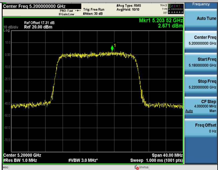
11N20SISO-Ant1-5200-PASS
